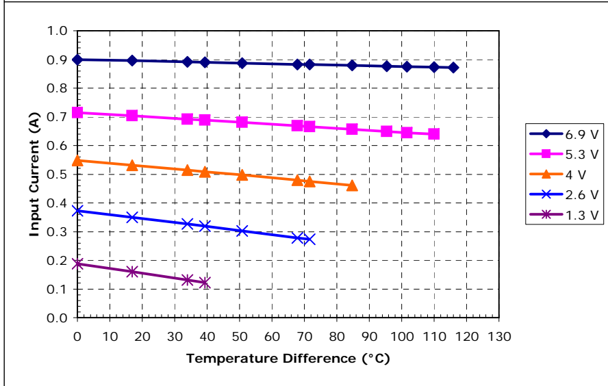
Unpotted TE-3-(59-17-4)-1.5 at a hot-side temperature of 30 °C
