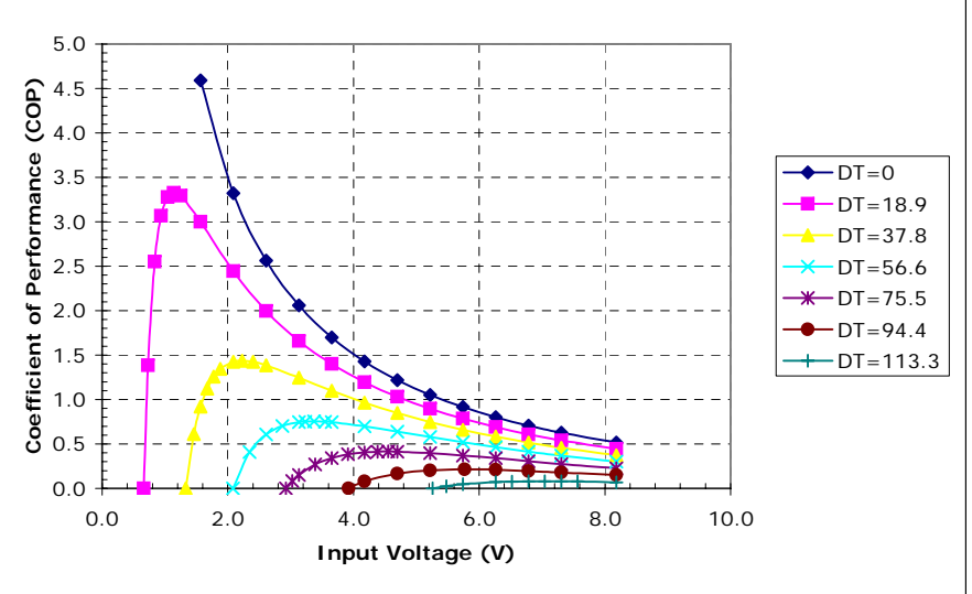
Potted TE-3-(59-17-4)-1.5 at a hot-side temperature of 70 °C
