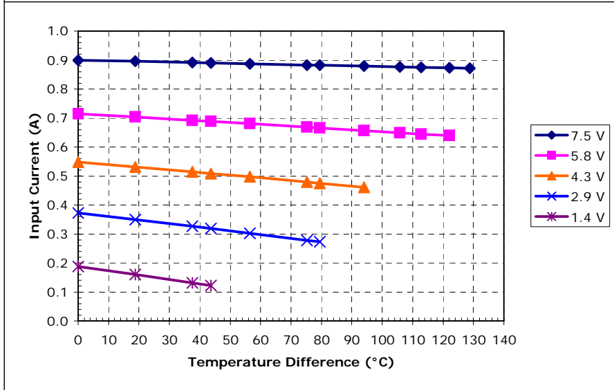
Unpotted TE-3-(59-17-4)-1.5 at a hot-side temperature of 50 °C
