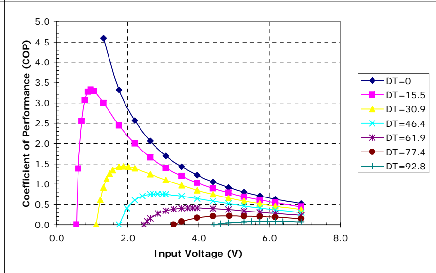
Potted TE-3-(59-17-4)-1.5 at a hot-side temperature of 30 °C
