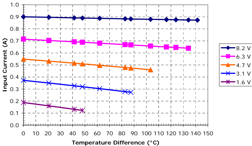
Unpotted TE-3-(59-17-4)-1.5 at a hot-side temperature of 70 °C
