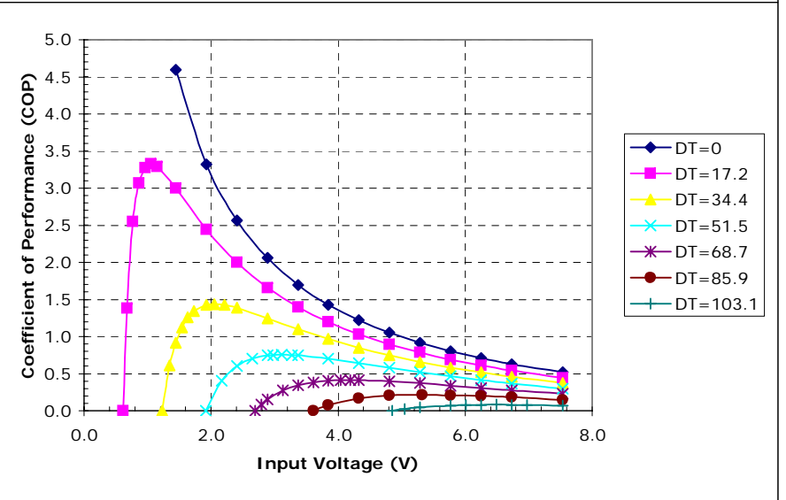
Potted TE-3-(59-17-4)-1.5 at a hot-side temperature of 50 °C
