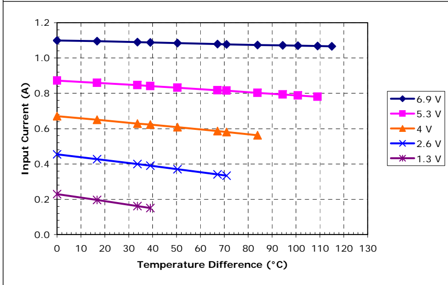
Unpotted TE-3-(59-17-4)-1.2 at a hot-side temperature of 30 °C
