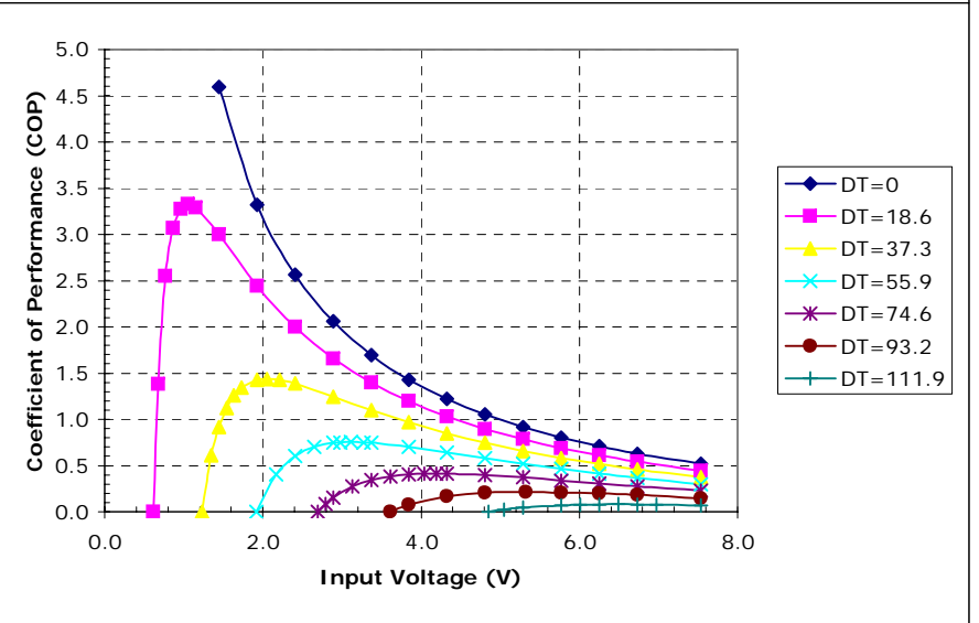
Unpotted TE-3-(59-17-4)-1.2 at a hot-side temperature of 50 °C
