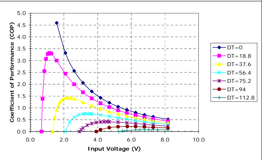
Potted TE-3-(59-17-4)-1.2 at a hot-side temperature of 70 °C
