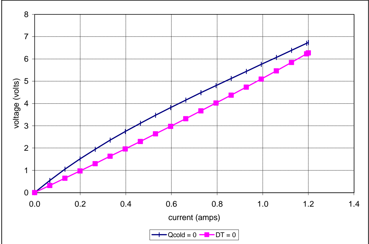
Unpotted TE-3-(59-17-4)-1.2 at a hot-side temperature of 25 °C
