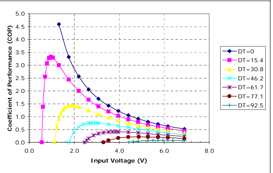
Potted TE-3-(59-17-4)-1.2 at a hot-side temperature of 30 °C
