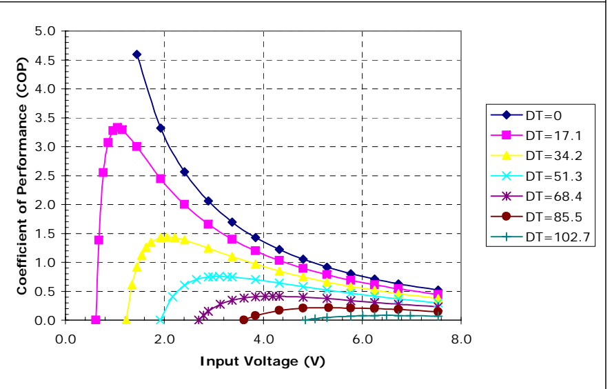
Potted TE-3-(59-17-4)-1.2 at a hot-side temperature of 50 °C
