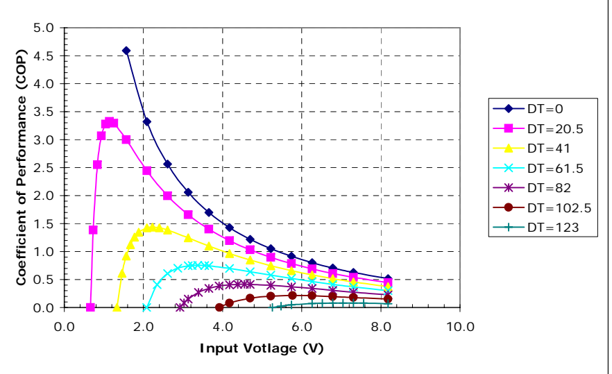
Unpotted TE-3-(59-17-4)-1.2 at a hot-side temperature of 70 °C
