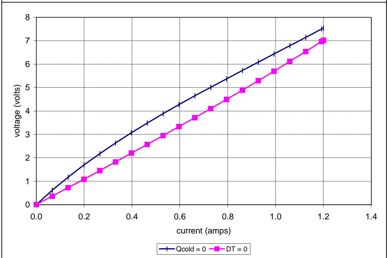
Unpotted TE-3-(59-17-4)-1.2 at a hot-side temperature of 50 °C
