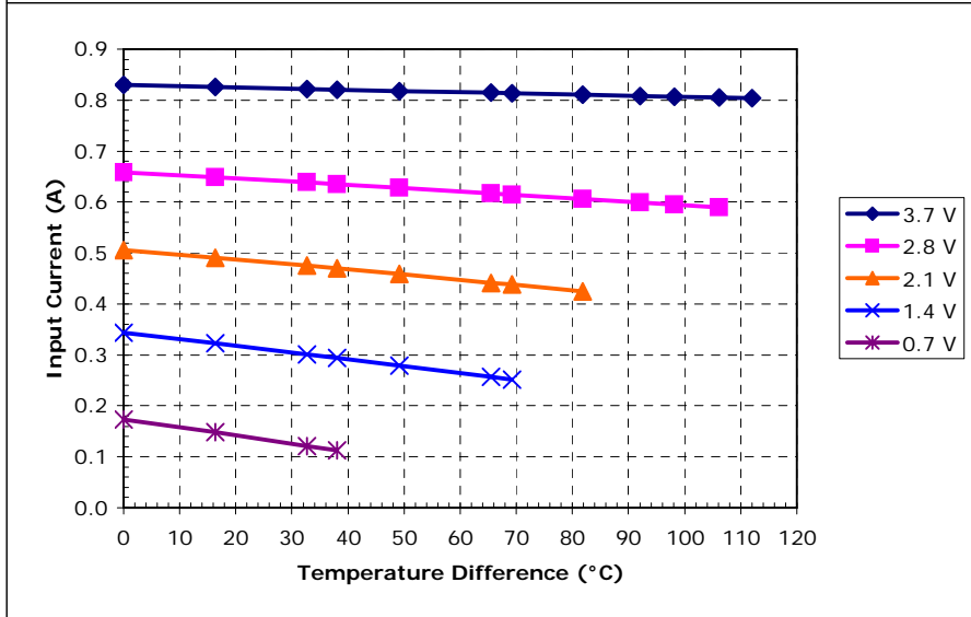
Unpotted TE-3-(31-11-4)-1.5 at a hot-side temperature of 30 °C
