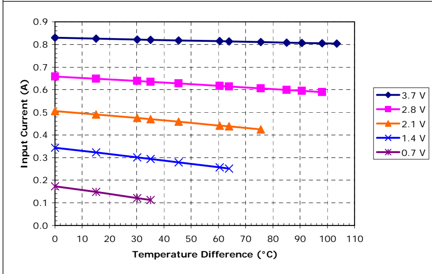
Potted TE-3-(31-11-4)-1.5 at a hot-side temperature of 30 °C
