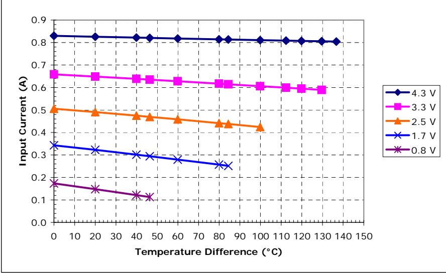
Unpotted TE-3-(31-11-4)-1.5 at a hot-side temperature of 70 °C
