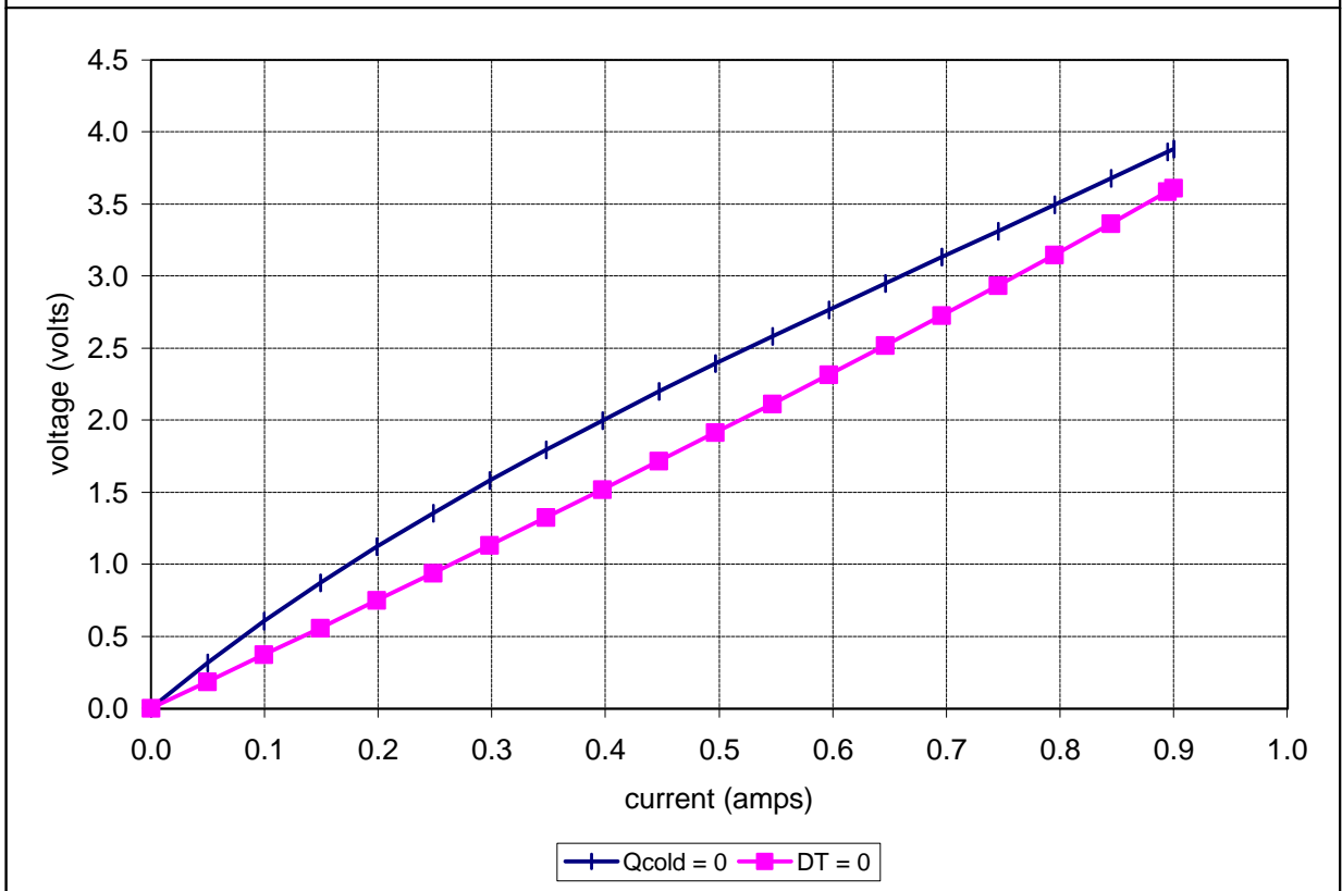
Unpotted TE-3-(31-11-4)-1.5 at a hot-side temperature of 50 °C
