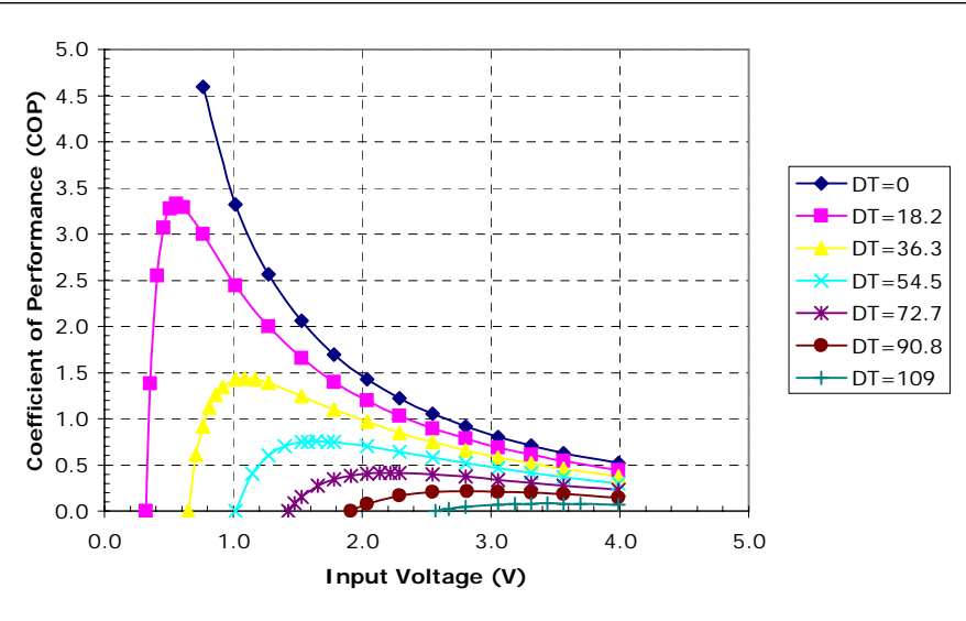
Unpotted TE-3-(31-11-4)-1.5 at a hot-side temperature of 50 °C
