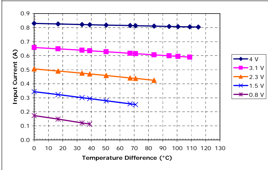
Potted TE-3-(31-11-4)-1.5 at a hot-side temperature of 50 °C
