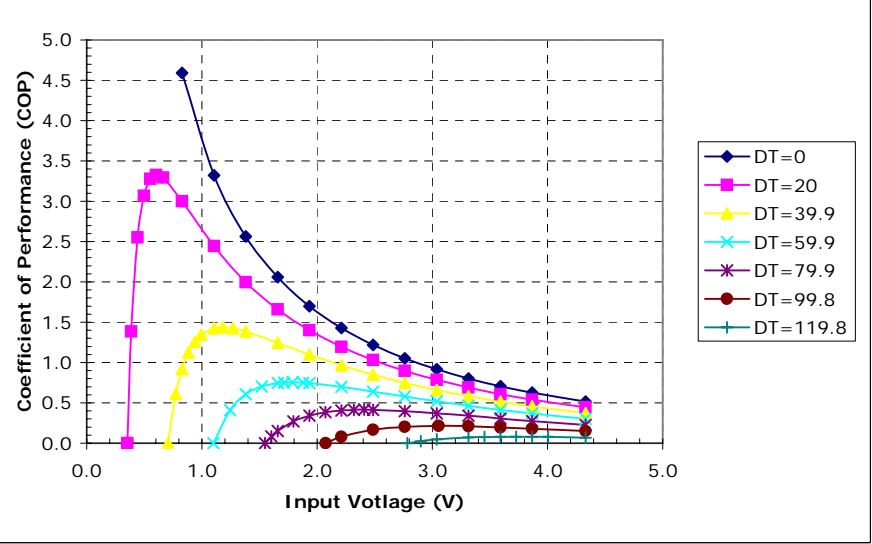
Unpotted TE-3-(31-11-4)-1.5 at a hot-side temperature of 70 °C
