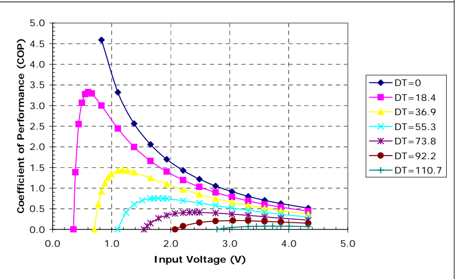
Potted TE-3-(31-11-4)-1.5 at a hot-side temperature of 70 °C
