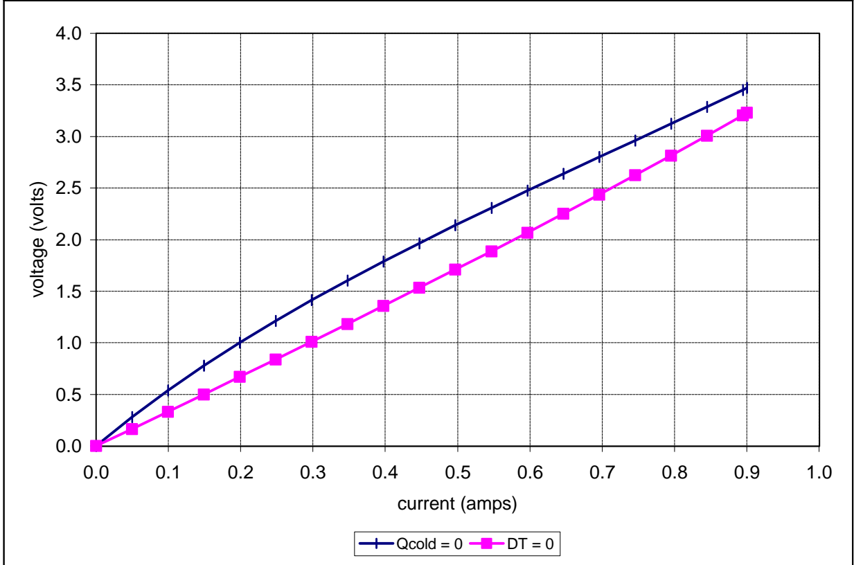
Unpotted TE-3-(31-11-4)-1.5 at a hot-side temperature of 25 °C
