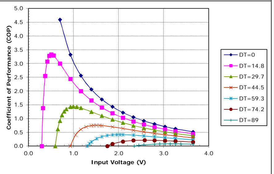
Potted TE-3-(31-11-4)-1.2 at a hot-side temperature of 30 °C
