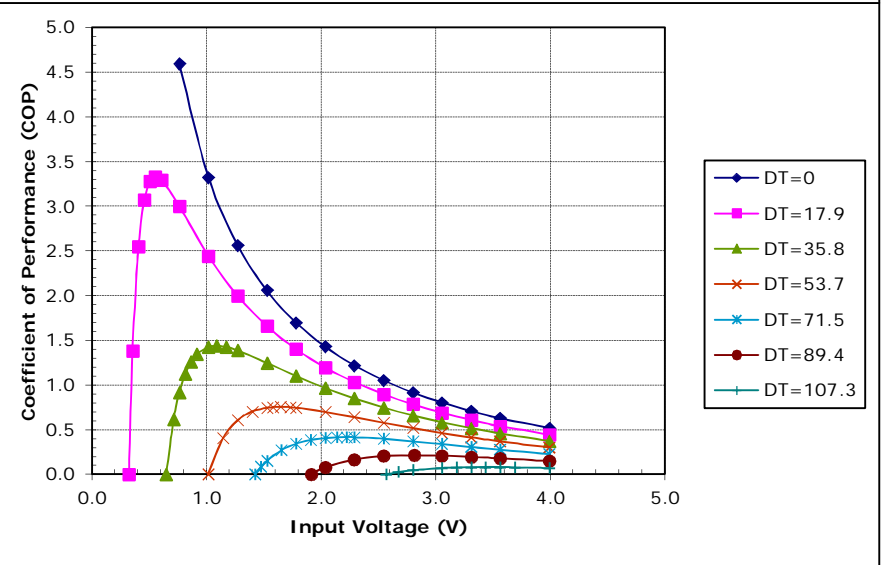
Unpotted TE-3-(31-11-4)-1.2 at a hot-side temperature of 50 °C
