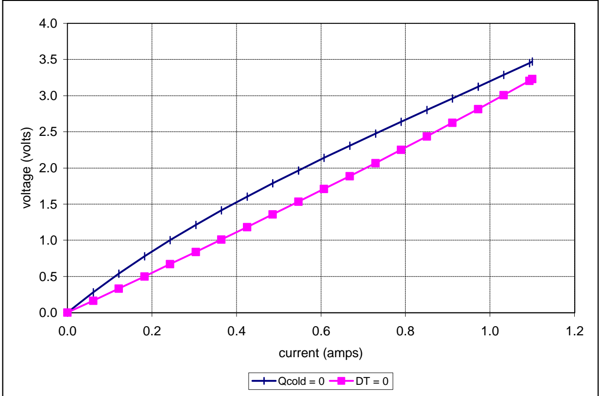
Unpotted TE-3-(31-11-4)-1.2 at a hot-side temperature of 25 °C
