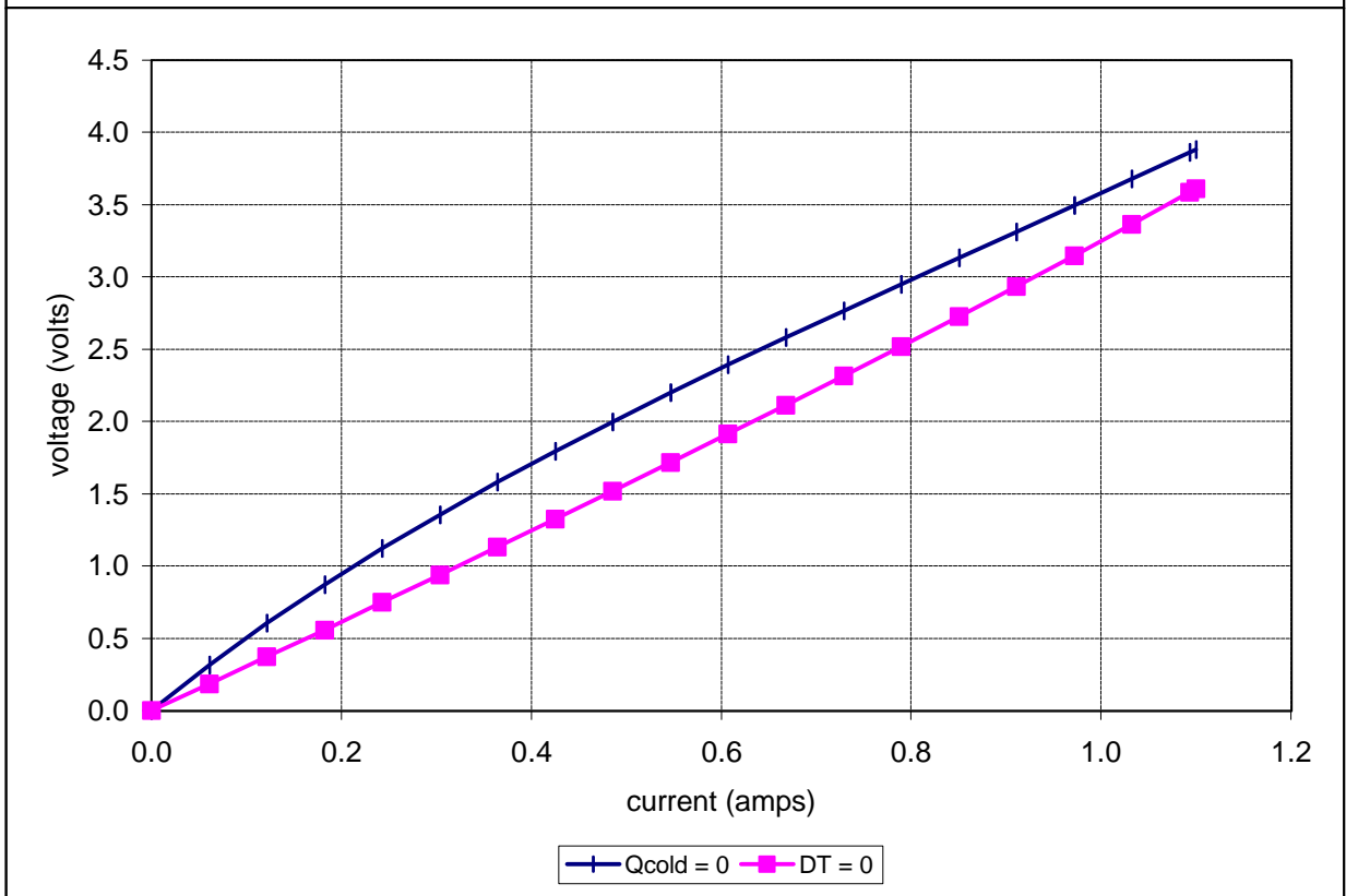
Unpotted TE-3-(31-11-4)-1.2 at a hot-side temperature of 50 °C
