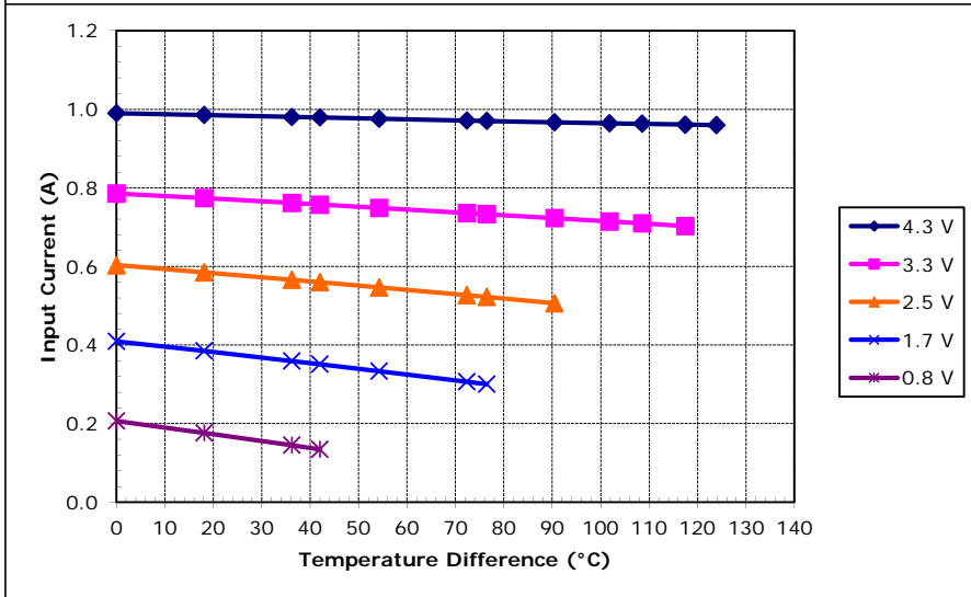
Potted TE-3-(31-11-4)-1.2 at a hot-side temperature of 70 °C
