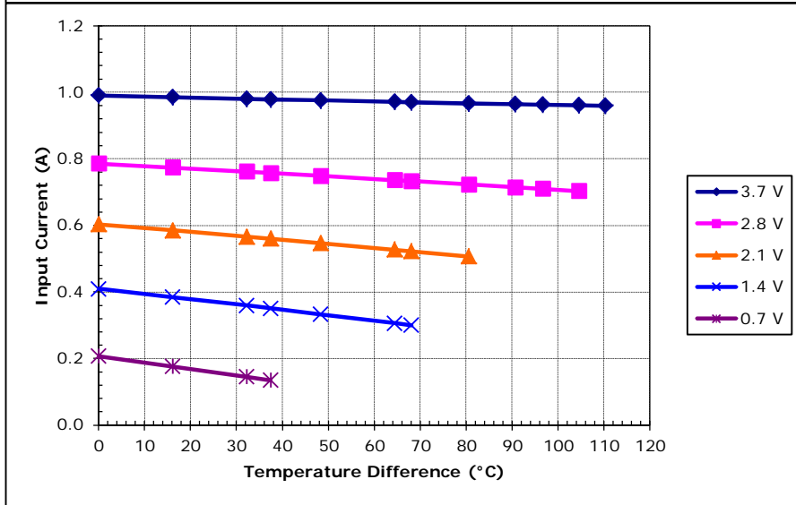
Unpotted TE-3-(31-11-4)-1.2 at a hot-side temperature of 30 °C
