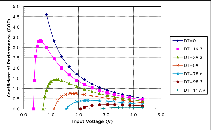
Unpotted TE-3-(31-11-4)-1.2 at a hot-side temperature of 70 °C
