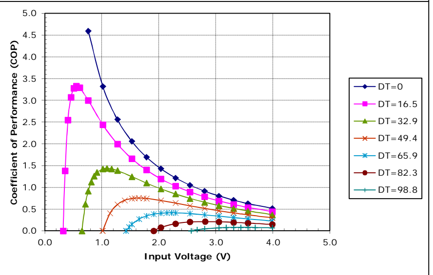
Potted TE-3-(31-11-4)-1.2 at a hot-side temperature of 50 °C
