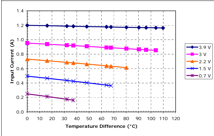
Potted TE-3-(31-11-4)-1.0 at a hot-side temperature of 50 °C
