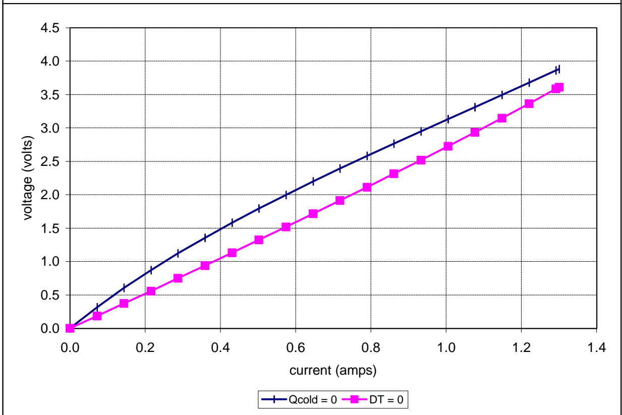
Unpotted TE-3-(31-11-4)-1.0 at a hot-side temperature of 50 °C
