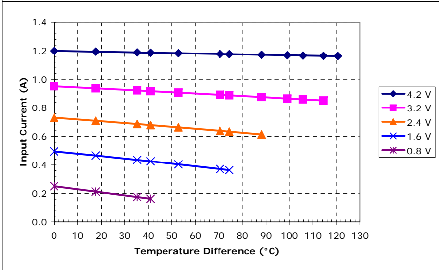
Potted TE-3-(31-11-4)-1.0 at a hot-side temperature of 70 °C
