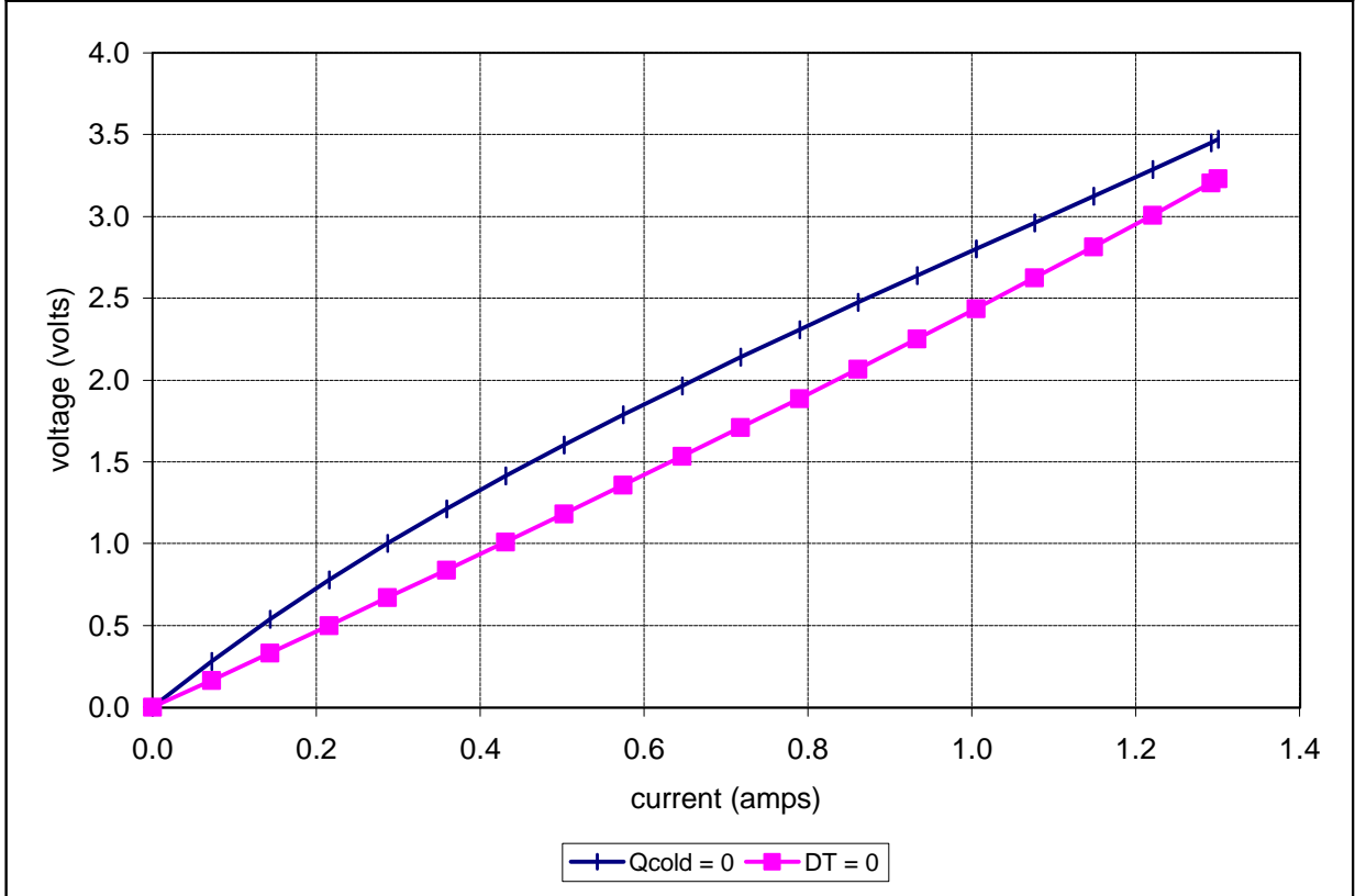
Unpotted TE-3-(31-11-4)-1.0 at a hot-side temperature of 25 °C
