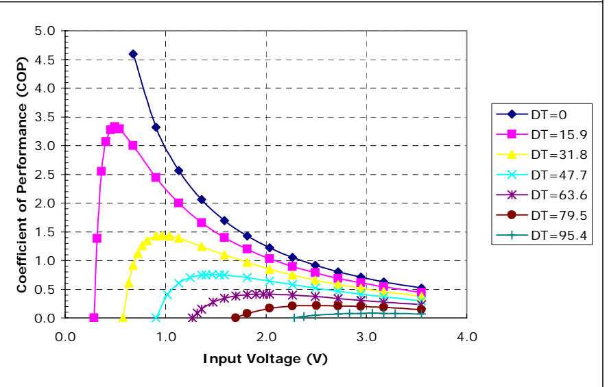
Unpotted TE-3-(31-11-4)-1.0 at a hot-side temperature of 30 °C
