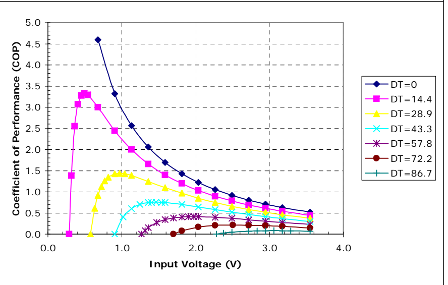
Potted TE-3-(31-11-4)-1.0 at a hot-side temperature of 30 °C
