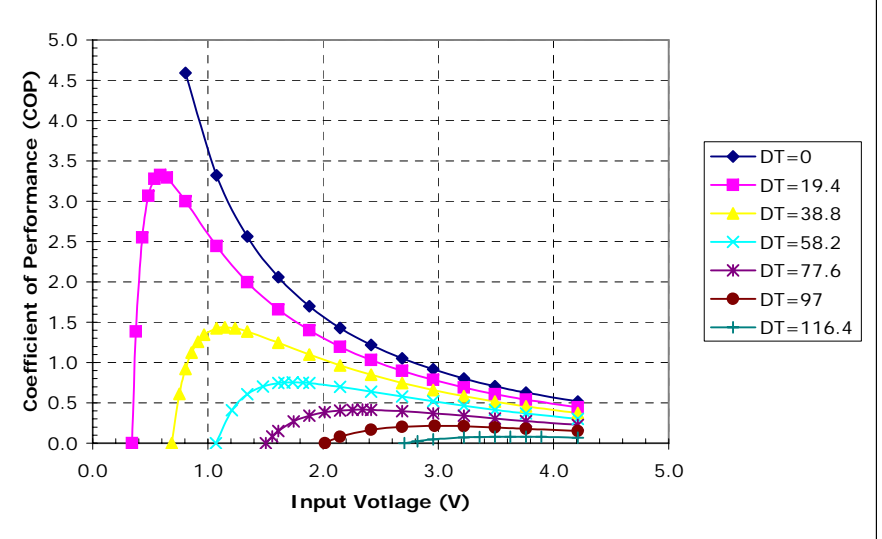
Unpotted TE-3-(31-11-4)-1.0 at a hot-side temperature of 70 °C
