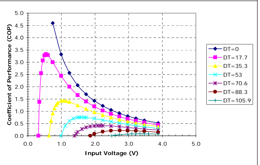
Unpotted TE-3-(31-11-4)-1.0 at a hot-side temperature of 50 °C
