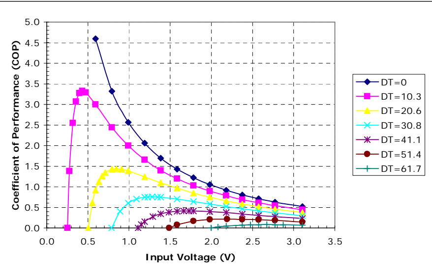
Potted TE-23-1.0-1.3 at a hot-side temperature of 50 °C
