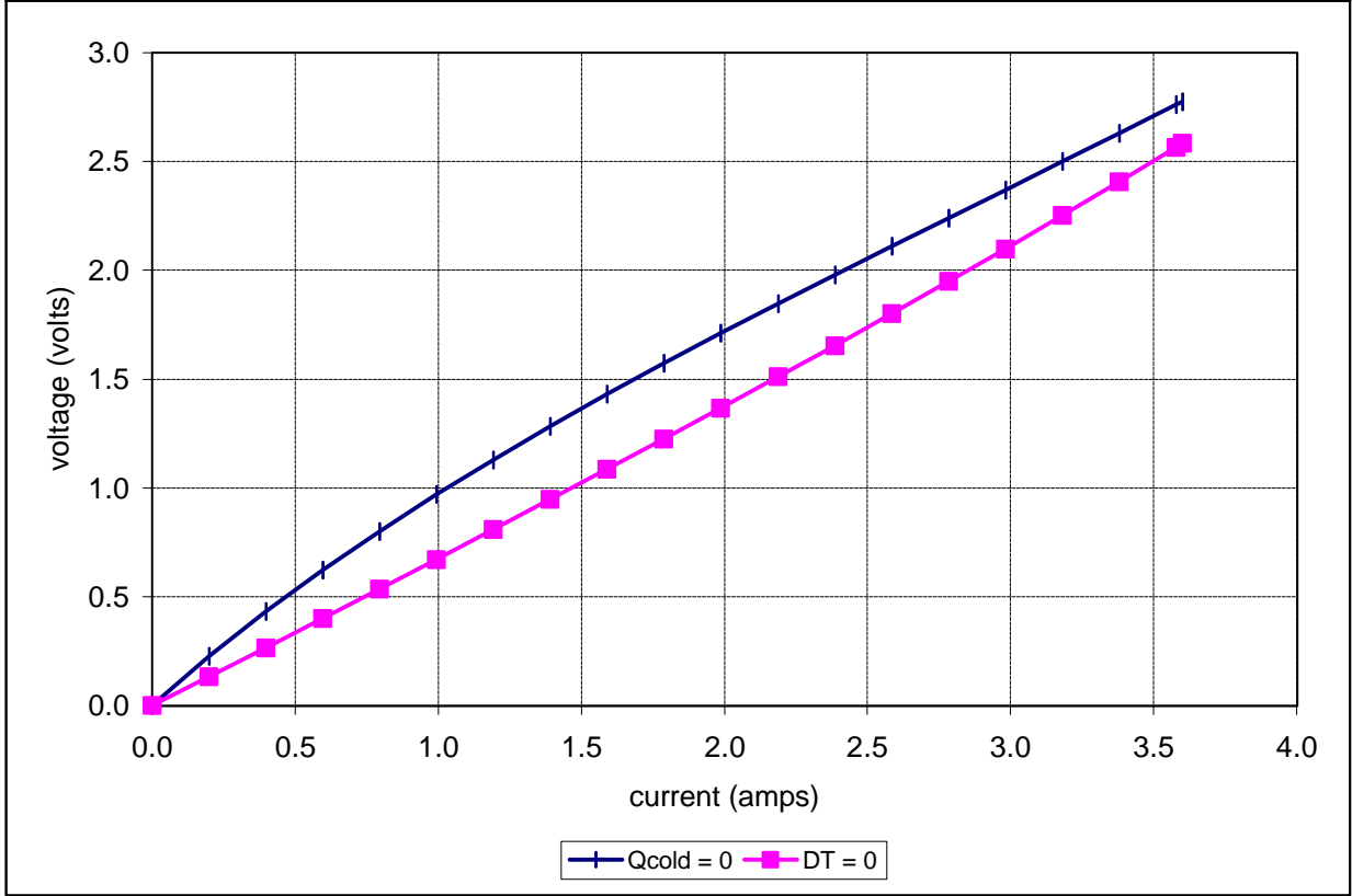
Unpotted TE-23-1.0-1.3 at a hot-side temperature of 25 °C
