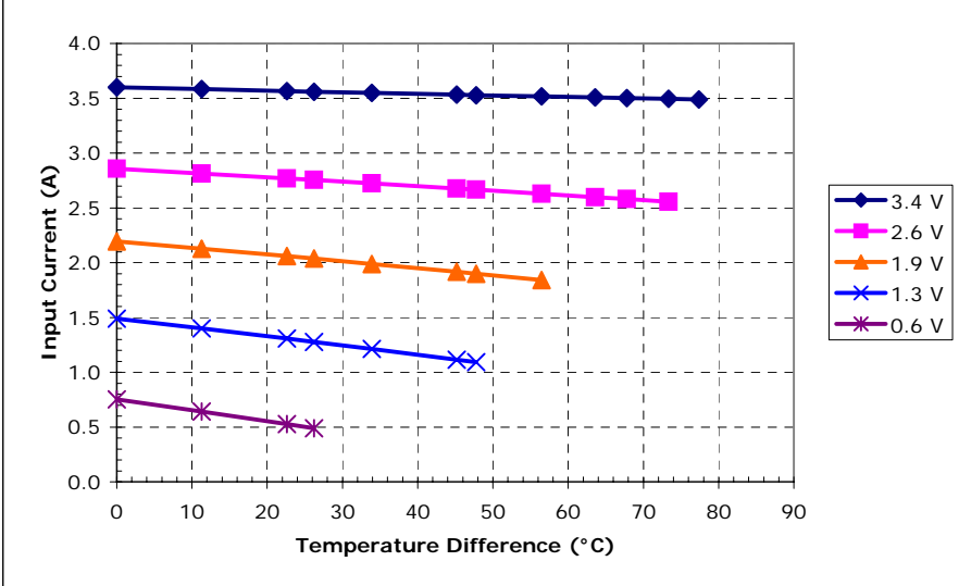
Potted TE-23-1.0-1.3 at a hot-side temperature of 70 °C
