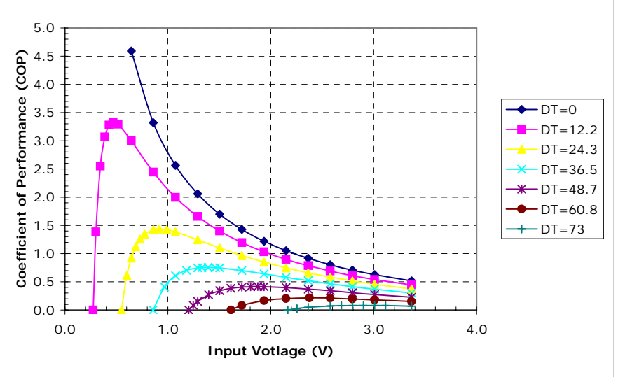
Unpotted TE-23-1.0-1.3 at a hot-side temperature of 70 °C
