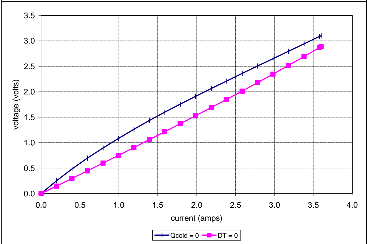
Potted TE-23-1.0-1.3 at a hot-side temperature of 50 °C
