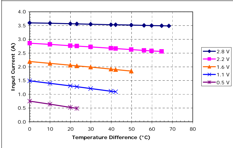
Unpotted TE-23-1.0-1.3 at a hot-side temperature of 30 °C
