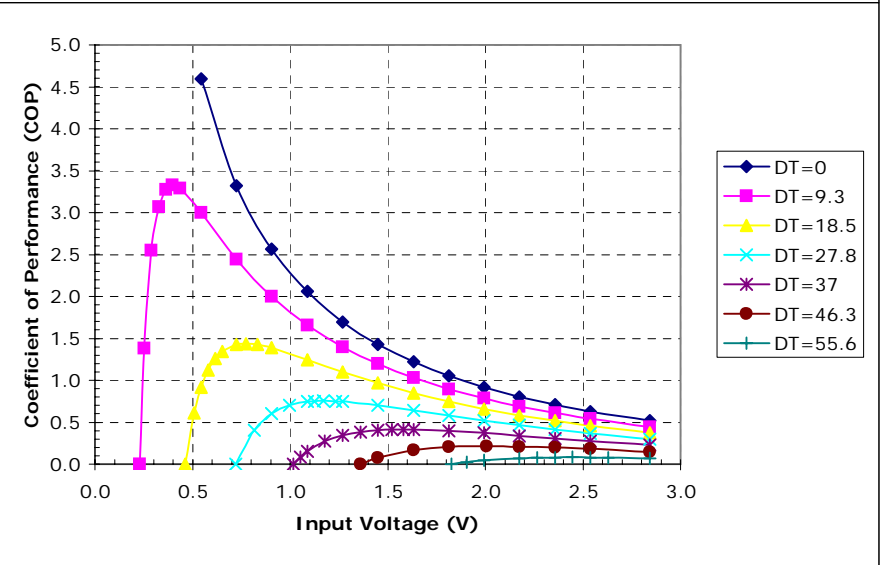
Potted TE-23-1.0-1.3 at a hot-side temperature of 30 °C
