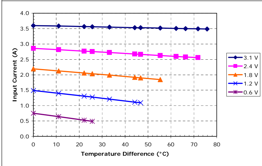
Unpotted TE-23-1.0-1.3 at a hot-side temperature of 50 °C
