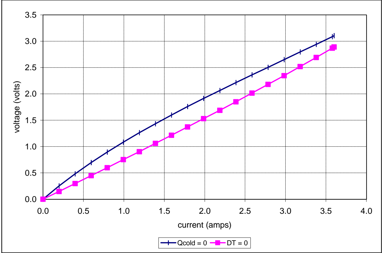
Unpotted TE-23-1.0-1.3 at a hot-side temperature of 50 °C
