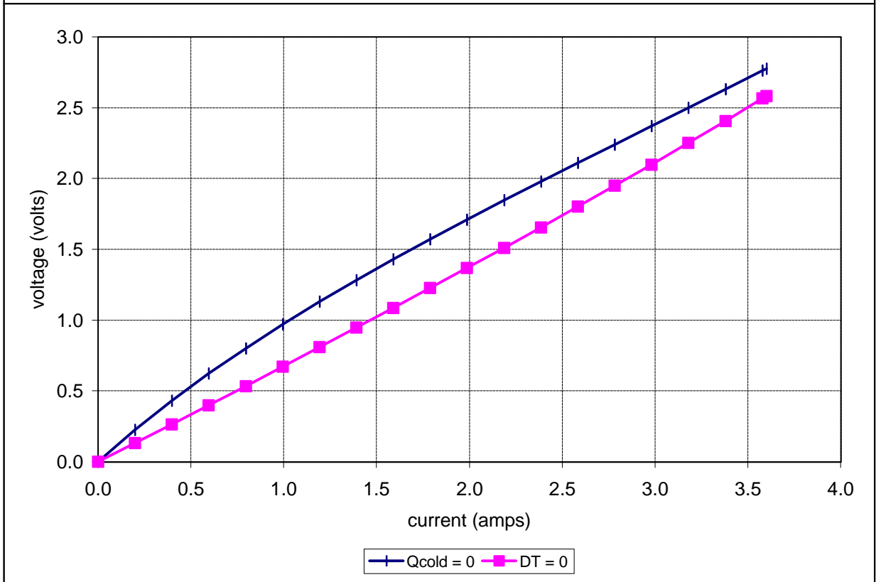
Potted TE-23-1.0-1.3 at a hot-side temperature of 25 °C
