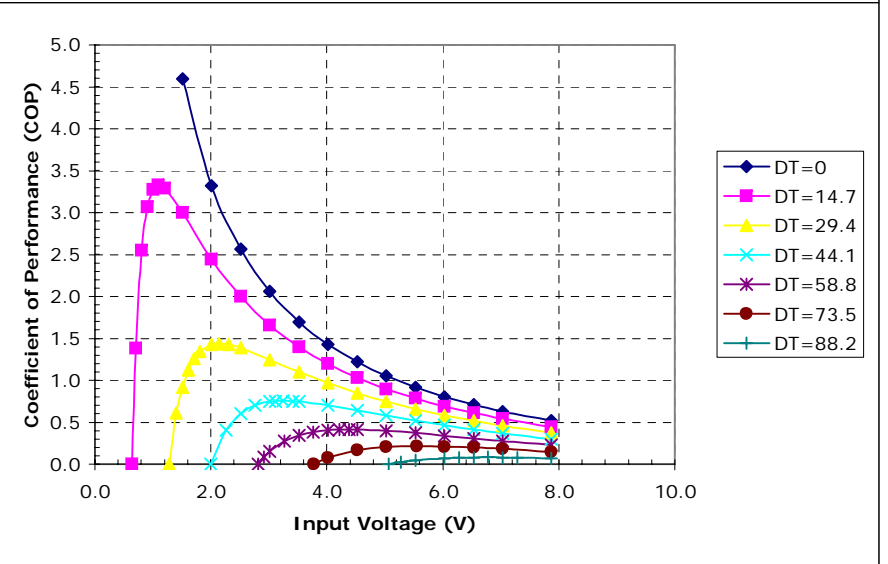
Potted TE-2-(59-18)-1.5 at a hot-side temperature of 50 °C
