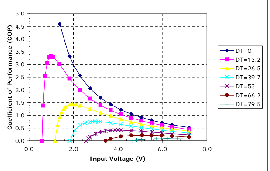
Potted TE-2-(59-18)-1.5 at a hot-side temperature of 30 °C
