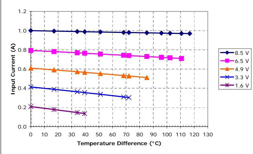
Unpotted TE-2-(59-18)-1.5 at a hot-side temperature of 70 °C
