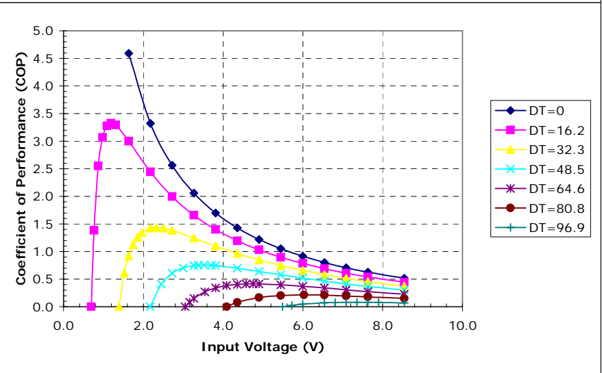
Potted TE-2-(59-18)-1.5 at a hot-side temperature of 70 °C
