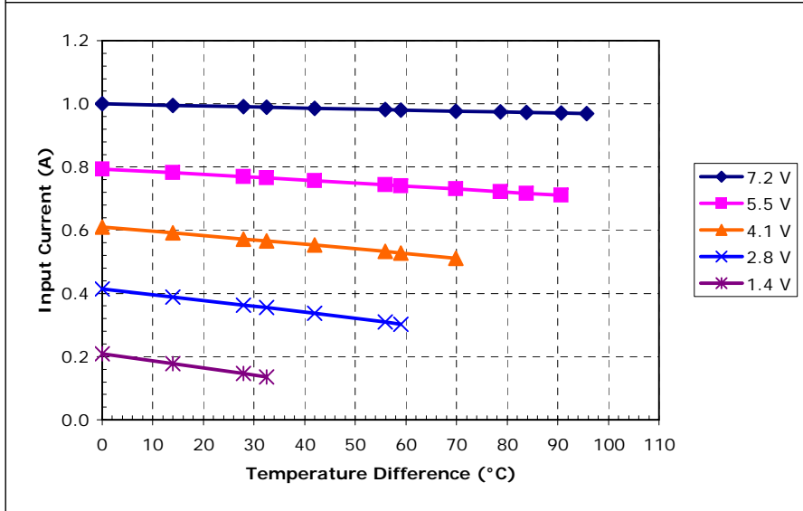
Unpotted TE-2-(59-18)-1.5 at a hot-side temperature of 30 °C
