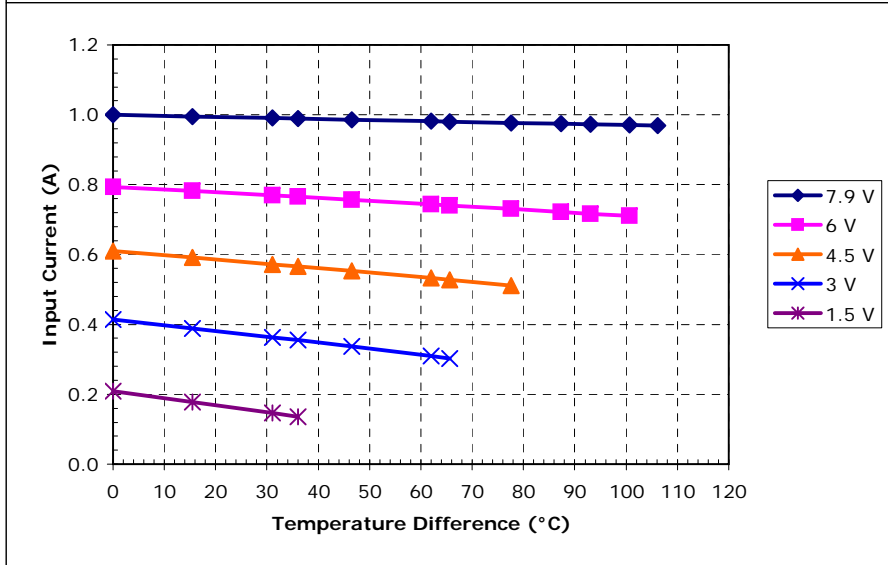
Unpotted TE-2-(59-18)-1.5 at a hot-side temperature of 50 °C
