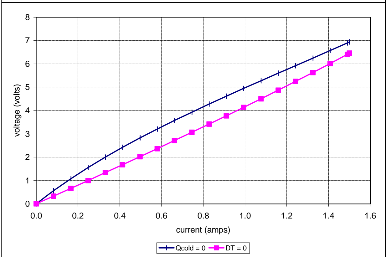
Unpotted TE-2-(59-18)-1.0 at a hot-side temperature of 25 °C
