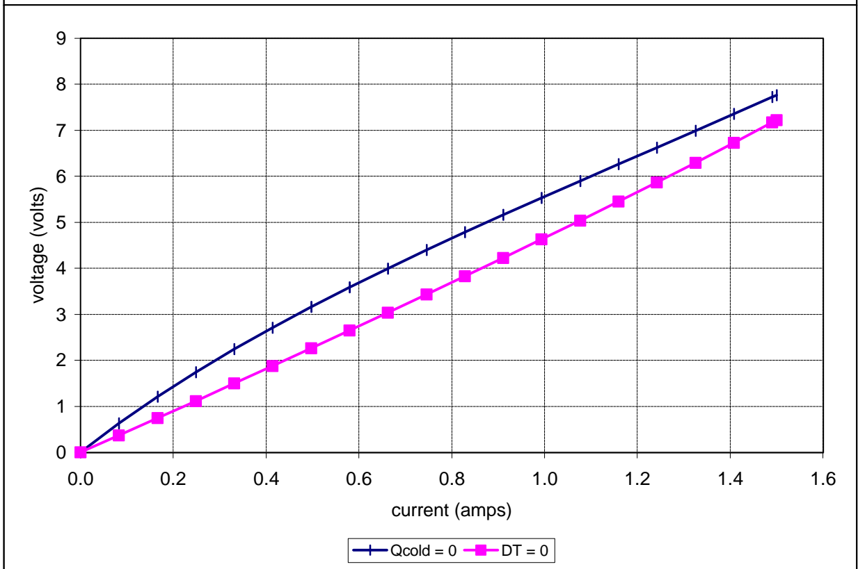
Unpotted TE-2-(59-18)-1.0 at a hot-side temperature of 50 °C
