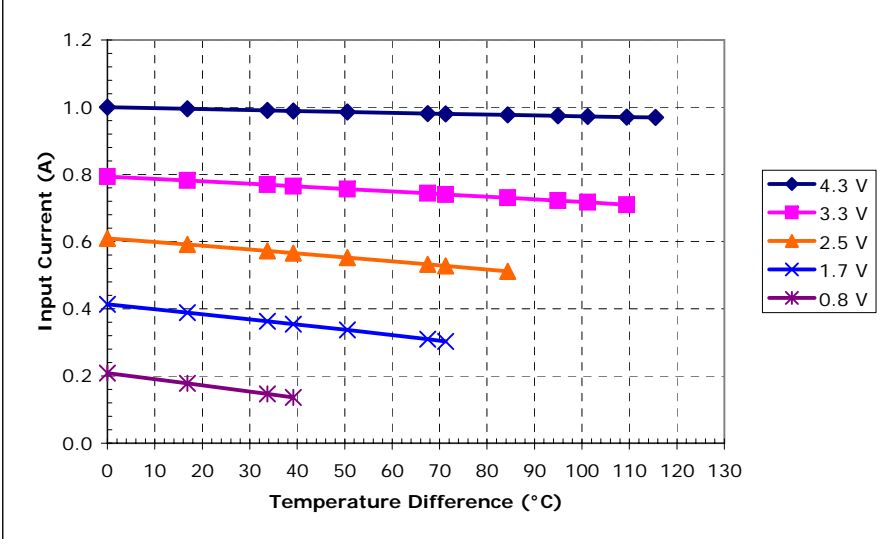
Unpotted TE-2-(31-8)-1.5 at a hot-side temperature of 70 °C
