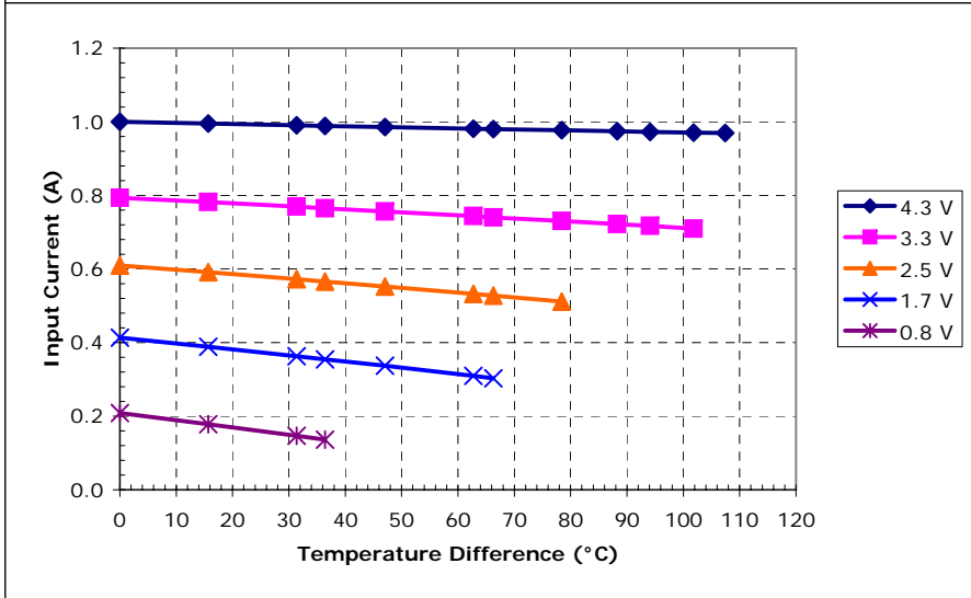
Potted TE-2-(31-8)-1.5 at a hot-side temperature of 70 °C
