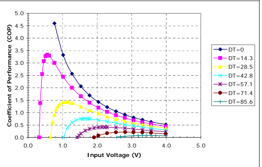
Potted TE-2-(31-8)-1.5 at a hot-side temperature of 50 °C
