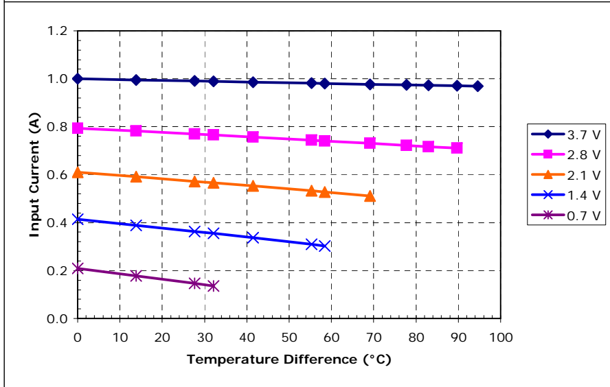
Unpotted TE-2-(31-8)-1.5 at a hot-side temperature of 30 °C
