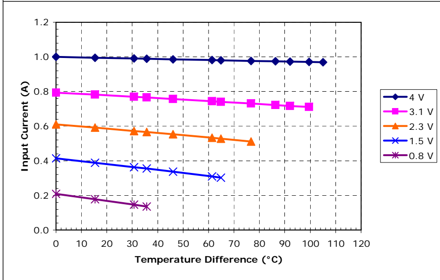
Unpotted TE-2-(31-8)-1.5 at a hot-side temperature of 50 °C
