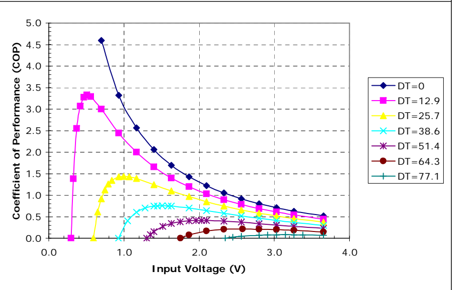
Potted TE-2-(31-8)-1.5 at a hot-side temperature of 30 °C
