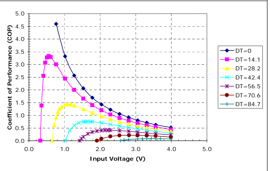
Potted TE-2-(31-8)-1.2 at a hot-side temperature of 50 °C
