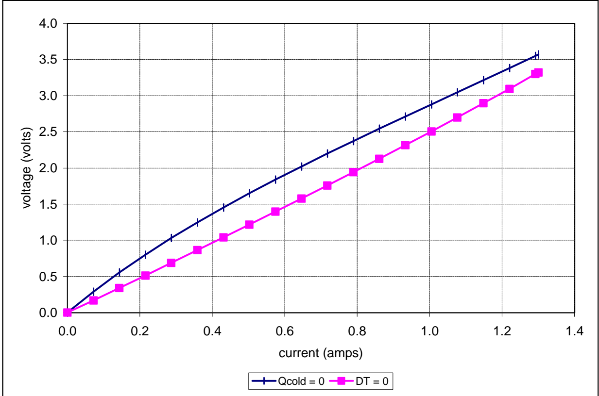
Unpotted TE-2-(31-8)-1.2 at a hot-side temperature of 25 °C
