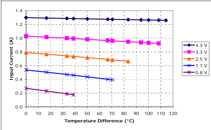
Unpotted TE-2-(31-8)-1.2 at a hot-side temperature of 70 °C
