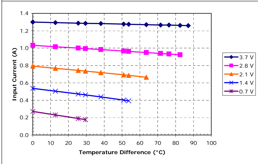
Potted TE-2-(31-8)-1.2 at a hot-side temperature of 30 °C
