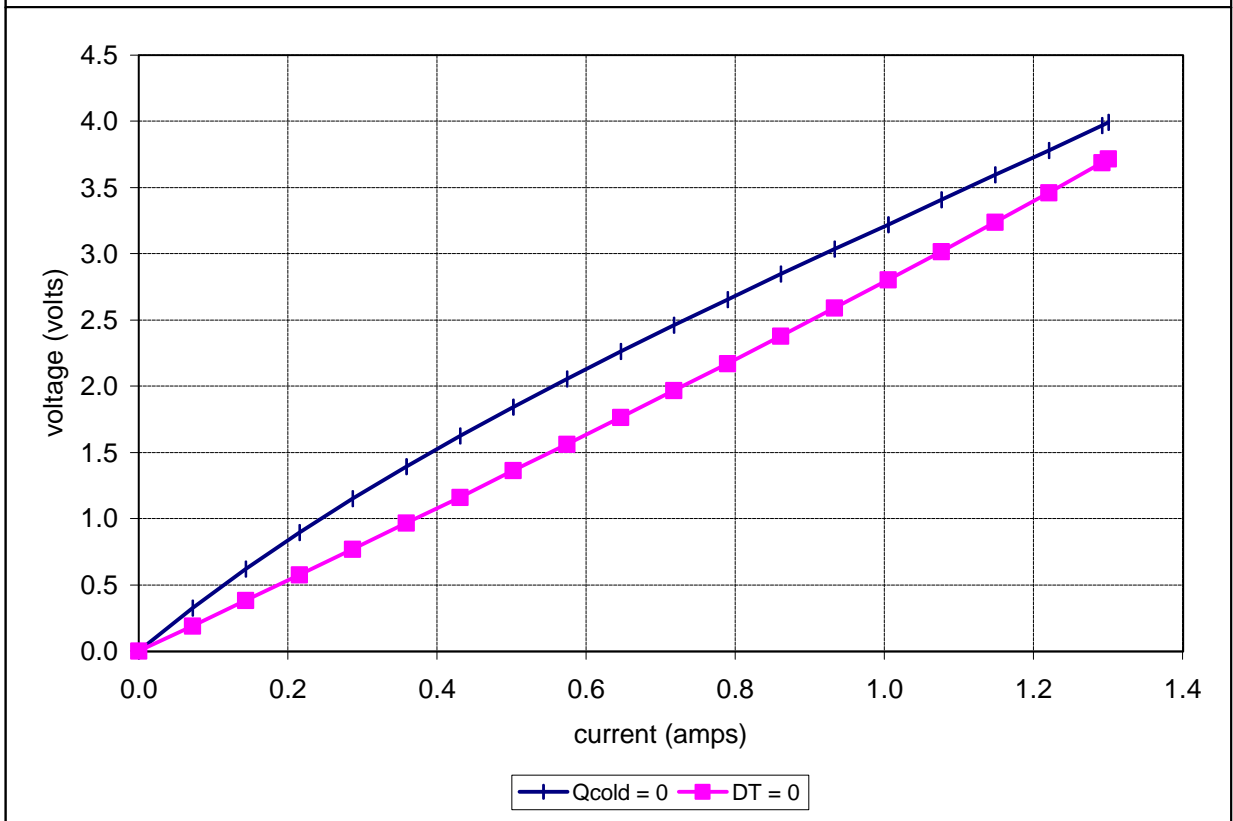
Unpotted TE-2-(31-8)-1.2 at a hot-side temperature of 50 °C
