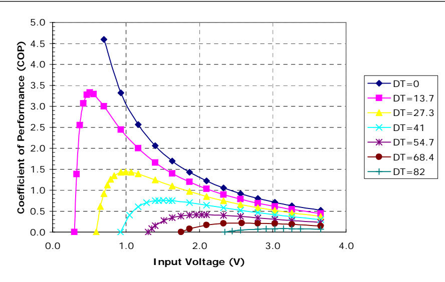
Unpotted TE-2-(31-8)-1.2 at a hot-side temperature of 30 °C
