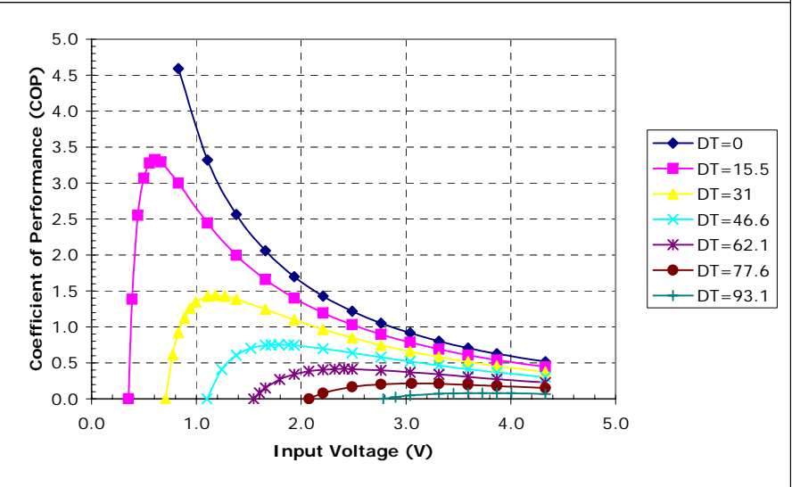
Potted TE-2-(31-8)-1.2 at a hot-side temperature of 70 °C
