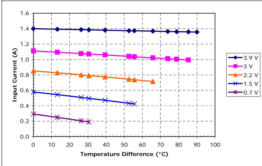
Potted TE-2-(31-8)-1.0 at a hot-side temperature of 30 °C
