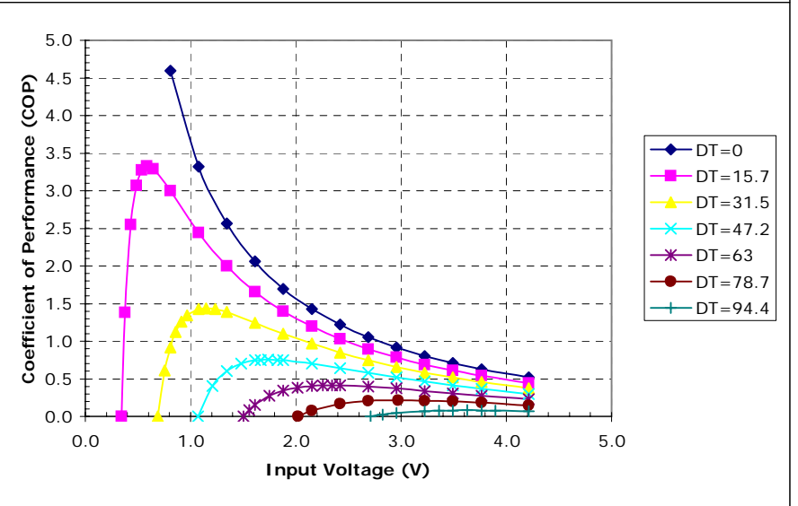
Unpotted TE-2-(31-8)-1.0 at a hot-side temperature of 50 °C
