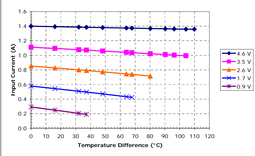
Potted TE-2-(31-8)-1.0 at a hot-side temperature of 70 °C
