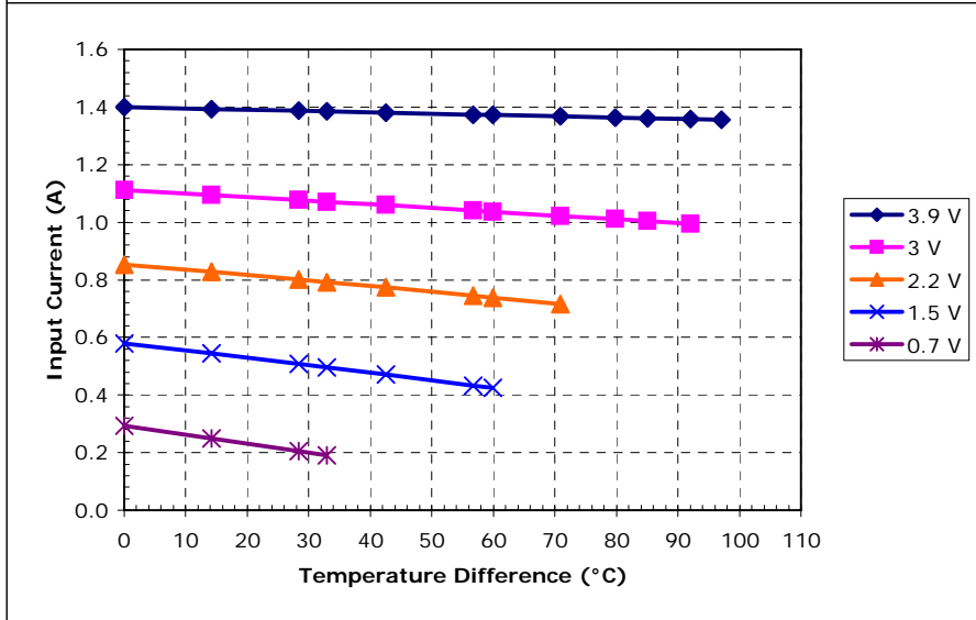
Unpotted TE-2-(31-8)-1.0 at a hot-side temperature of 30 °C
