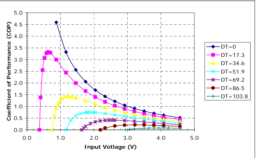
Unpotted TE-2-(31-8)-1.0 at a hot-side temperature of 70 °C
