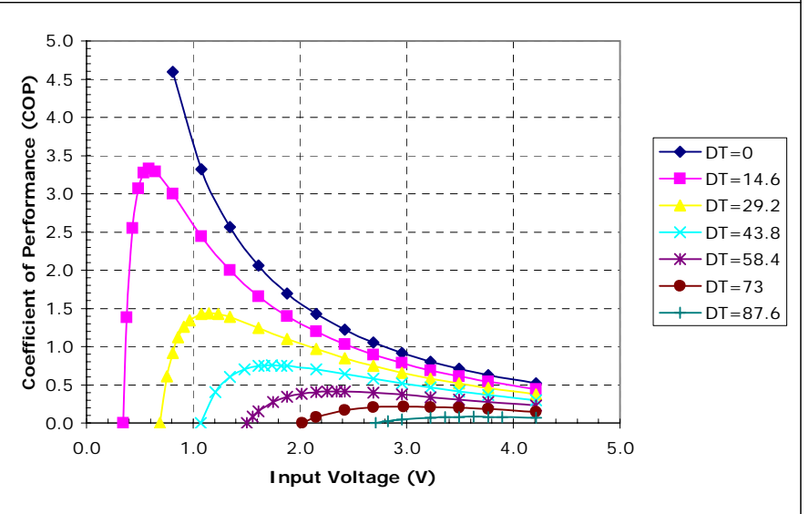
Potted TE-2-(31-8)-1.0 at a hot-side temperature of 50 °C
