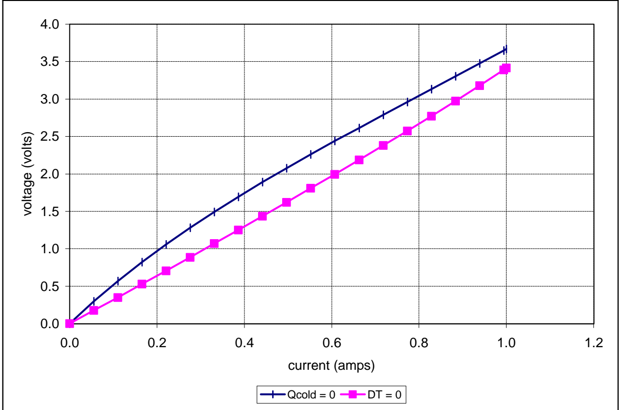
Unpotted TE-2-(31-12)-1.5 at a hot-side temperature of 25 °C
