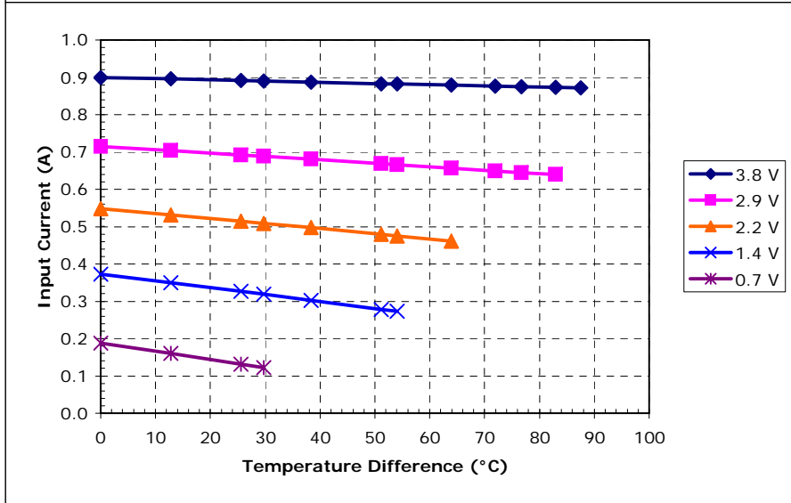
Potted TE-2-(31-12)-1.5 at a hot-side temperature of 30 °C
