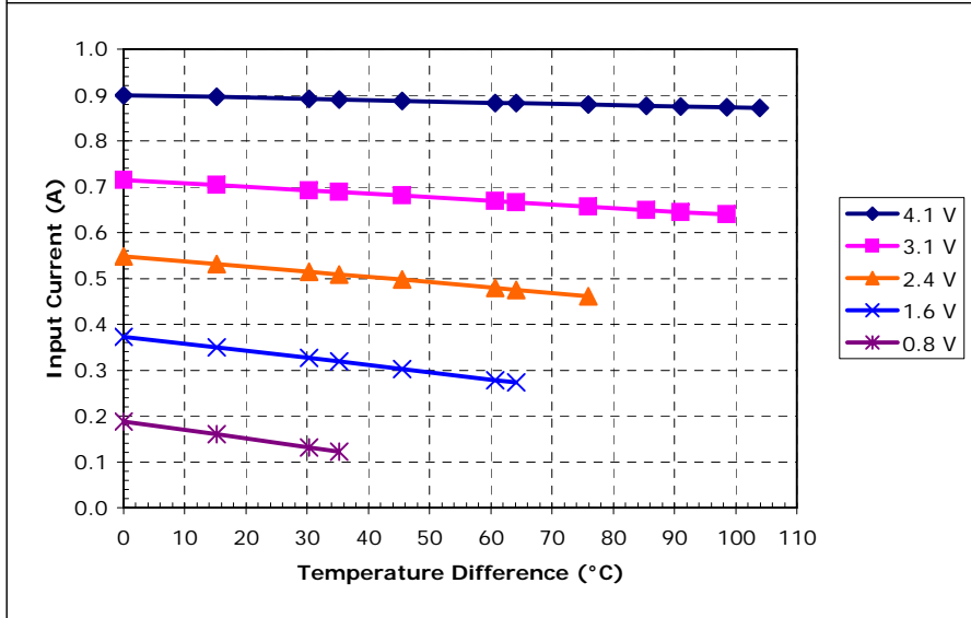
Unpotted TE-2-(31-12)-1.5 at a hot-side temperature of 50 °C
