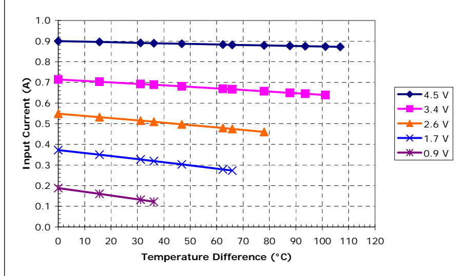
Potted TE-2-(31-12)-1.5 at a hot-side temperature of 70 °C
