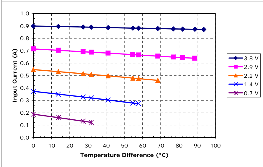
Unpotted TE-2-(31-12)-1.5 at a hot-side temperature of 30 °C
