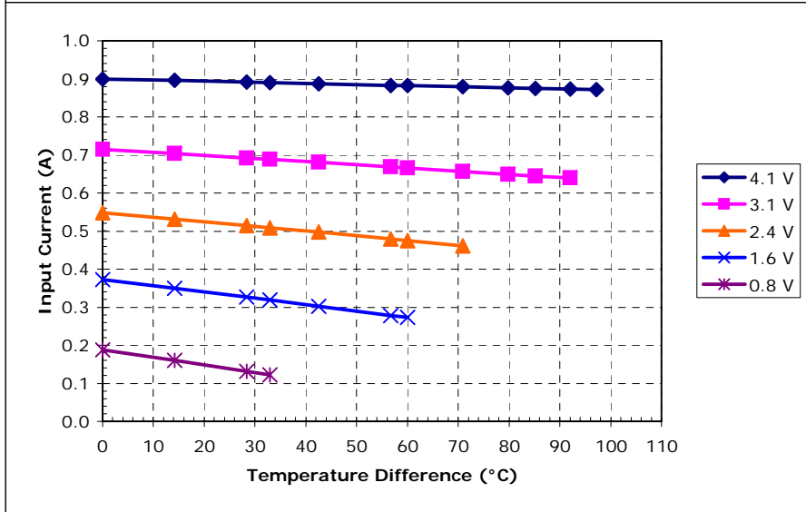
Potted TE-2-(31-12)-1.5 at a hot-side temperature of 50 °C
