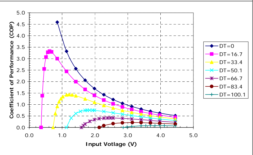
Unpotted TE-2-(31-12)-1.5 at a hot-side temperature of 70 °C
