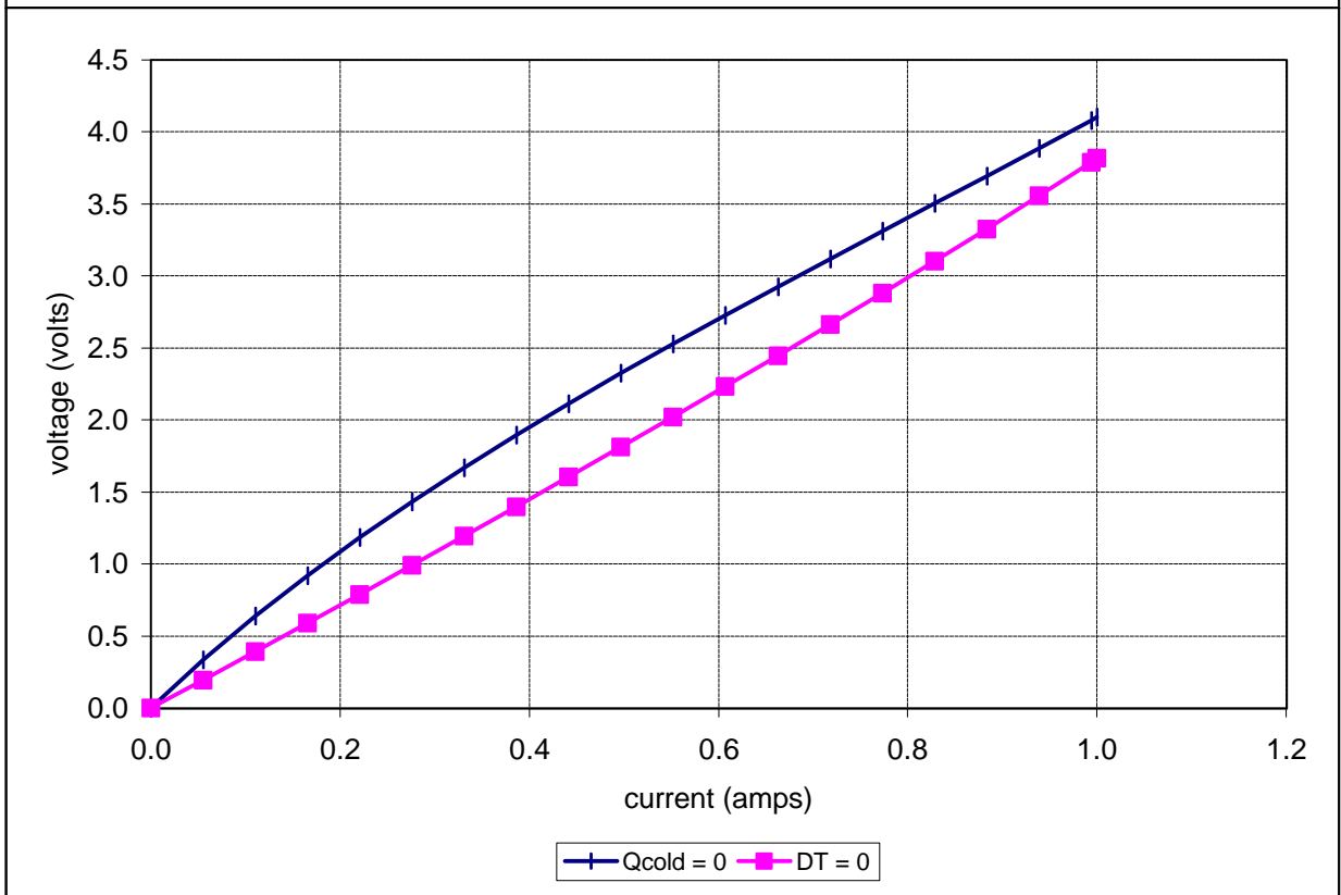
Unpotted TE-2-(31-12)-1.5 at a hot-side temperature of 50 °C
