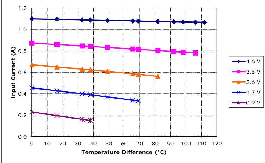
Unpotted TE-2-(31-12)-1.2 at a hot-side temperature of 70 °C
