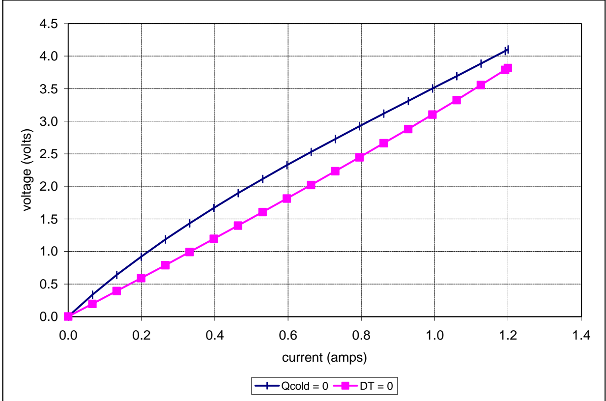
Unpotted TE-2-(31-12)-1.2 at a hot-side temperature of 50 °C
