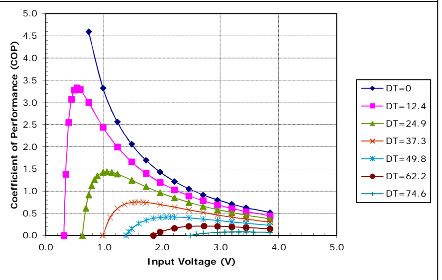
Potted TE-2-(31-12)-1.2 at a hot-side temperature of 30 °C
