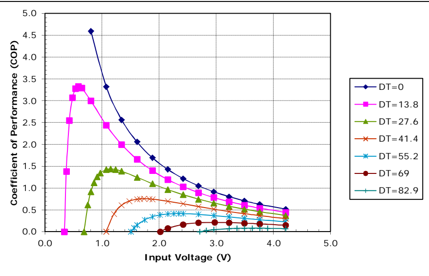
Potted TE-2-(31-12)-1.2 at a hot-side temperature of 50 °C
