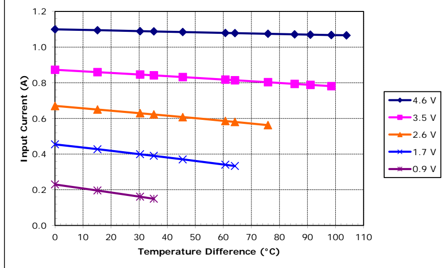
Potted TE-2-(31-12)-1.2 at a hot-side temperature of 70 °C
