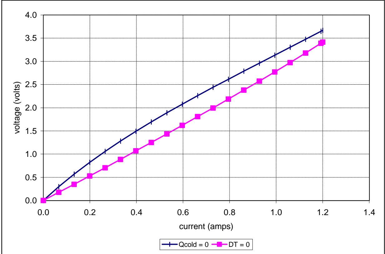
Unpotted TE-2-(31-12)-1.2 at a hot-side temperature of 25 °C
