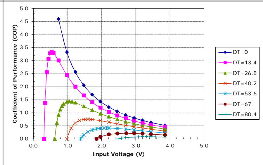
Unpotted TE-2-(31-12)-1.2 at a hot-side temperature of 30 °C
