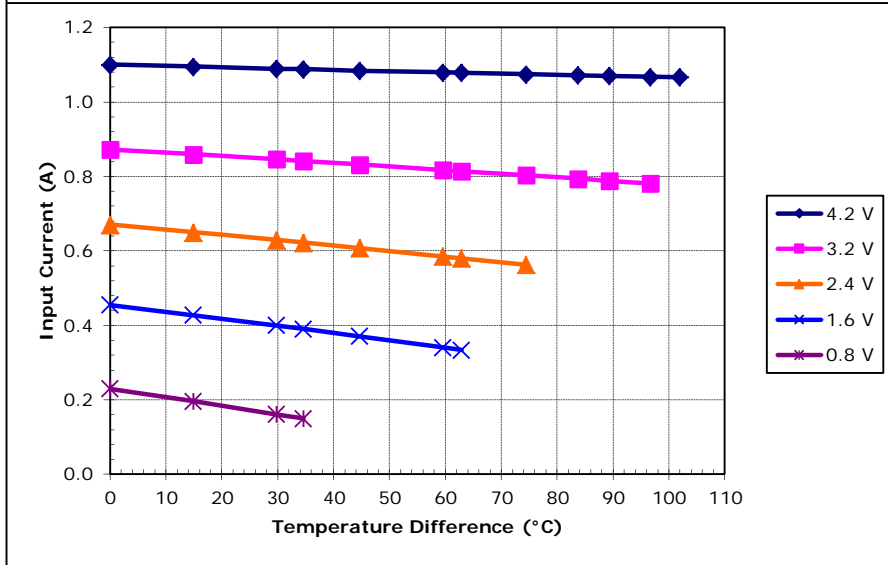
Unpotted TE-2-(31-12)-1.2 at a hot-side temperature of 50 °C
