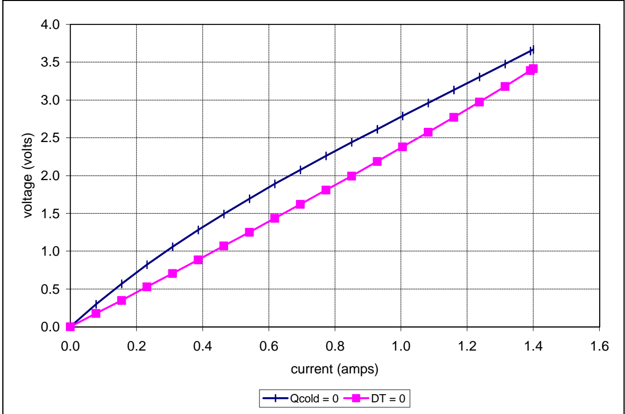
Unpotted TE-2-(31-12)-1.0 at a hot-side temperature of 25 °C
