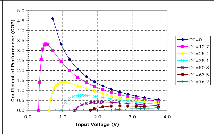
Potted TE-2-(31-12)-1.0 at a hot-side temperature of 30 °C
