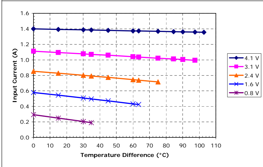
Unpotted TE-2-(31-12)-1.0 at a hot-side temperature of 50 °C
