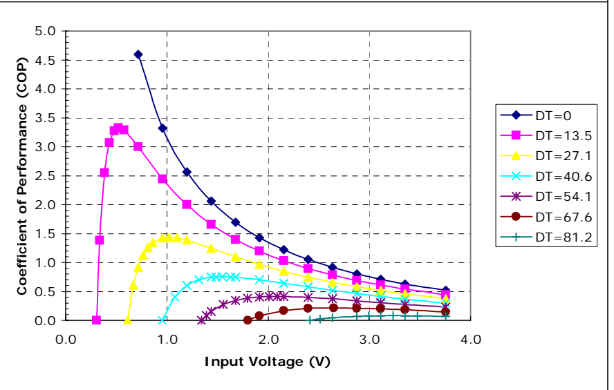
Unpotted TE-2-(31-12)-1.0 at a hot-side temperature of 30 °C
