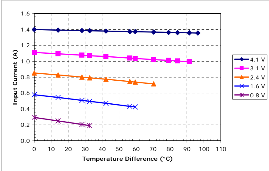
Potted TE-2-(31-12)-1.0 at a hot-side temperature of 50 °C
