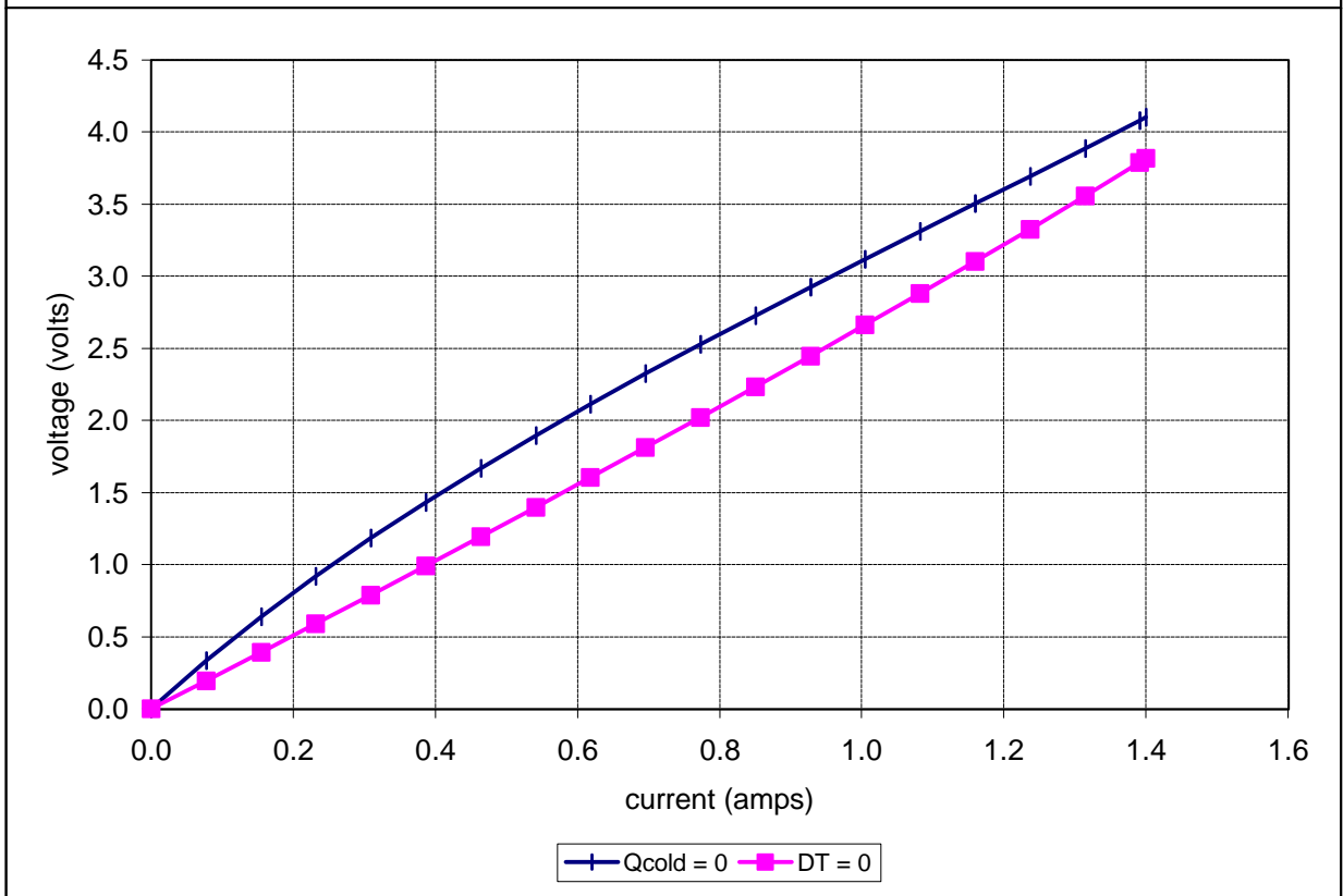
Unpowered TE-2-(31-12)-1.0 at a hot-side temperature of 50 °C
