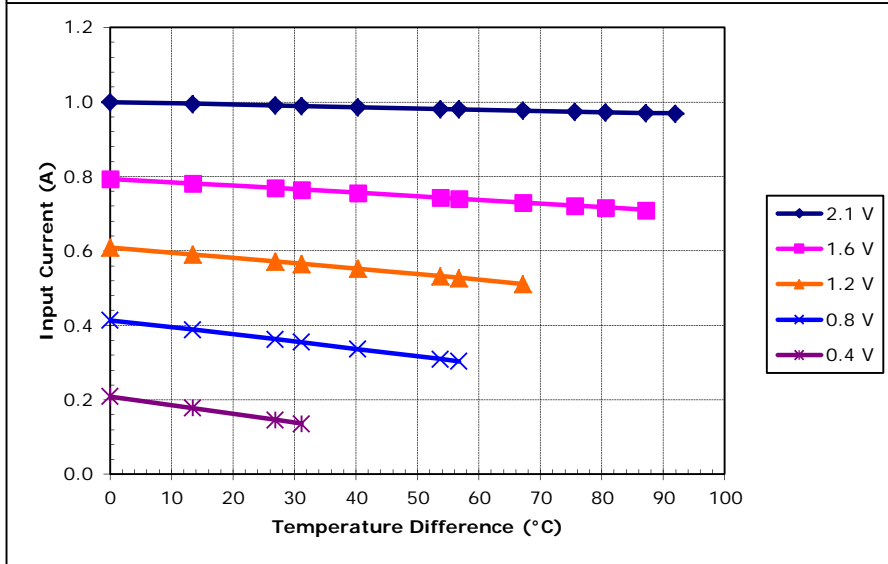
Potted TE-2-(17-4)-1.5 at a hot-side temperature of 30 °C
