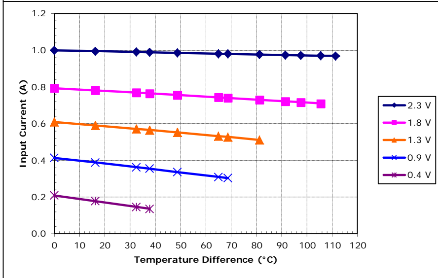
Unpotted TE-2-(17-4)-1.5 at a hot-side temperature of 50 °C
