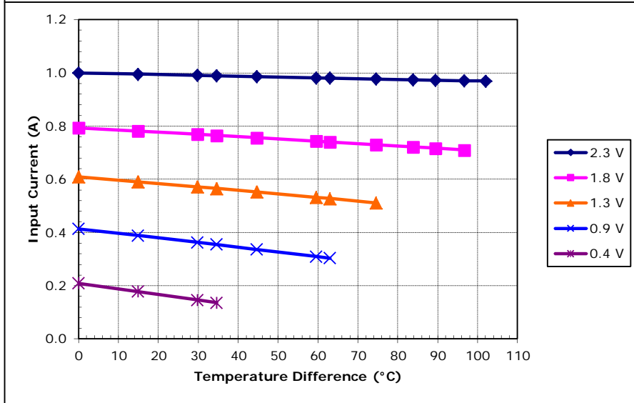
Potted TE-2-(17-4)-1.5 at a hot-side temperature of 50 °C
