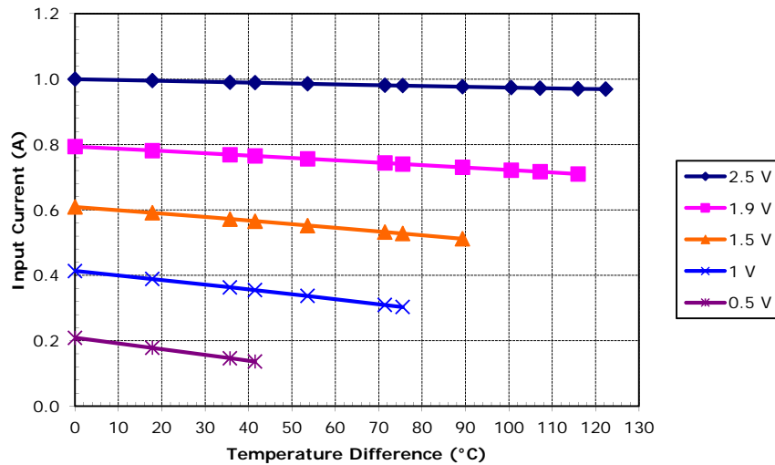
Unpotted TE-2-(17-4)-1.5 at a hot-side temperature of 70 °C
