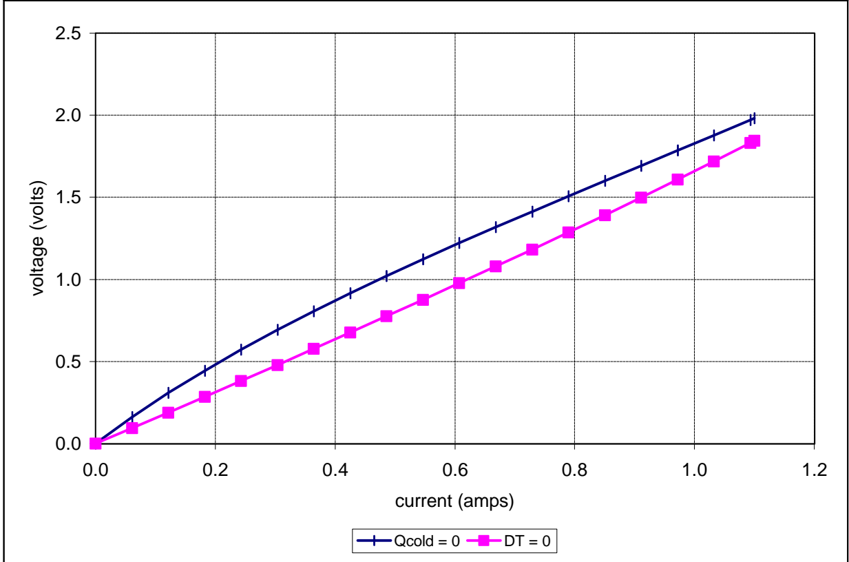
Unpotted TE-2-(17-4)-1.5 at a hot-side temperature of 25 °C
