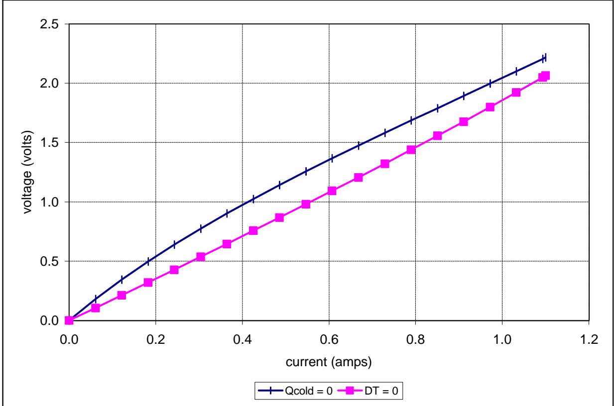
Unpotted TE-2-(17-4)-1.5 at a hot-side temperature of 50 °C
