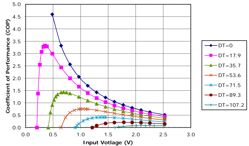
Unpotted TE-2-(17-4)-1.5 at a hot-side temperature of 70 °C
