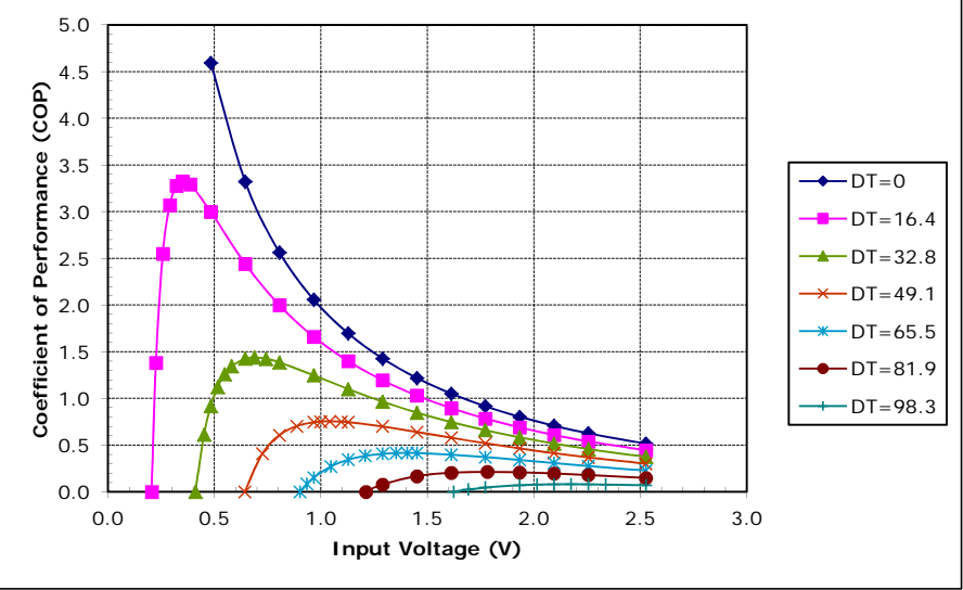
Potted TE-2-(17-4)-1.5 at a hot-side temperature of 70 °C
