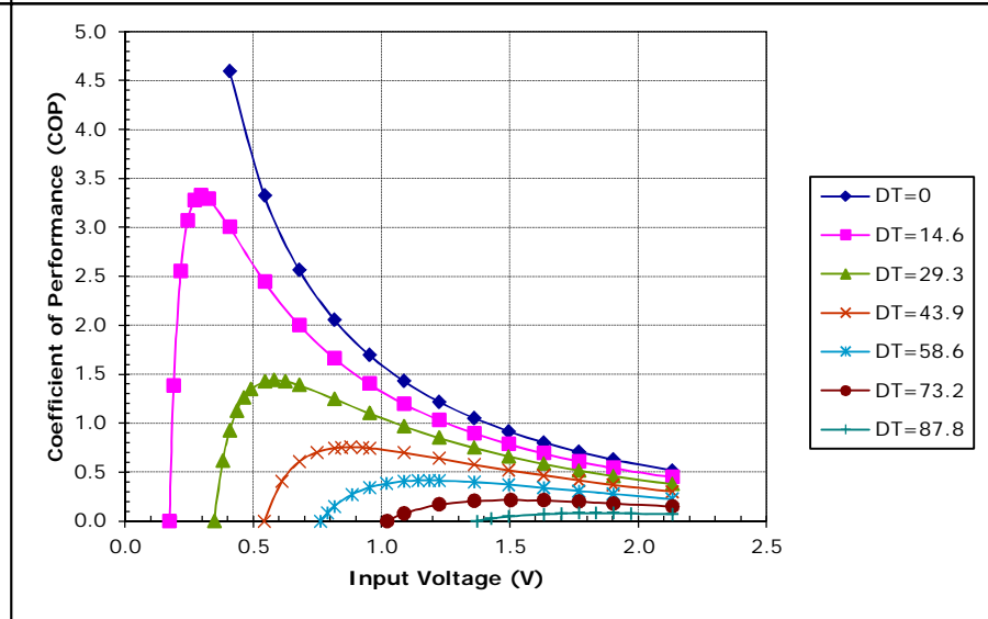
Unpotted TE-2-(17-4)-1.5 at a hot-side temperature of 30 °C
