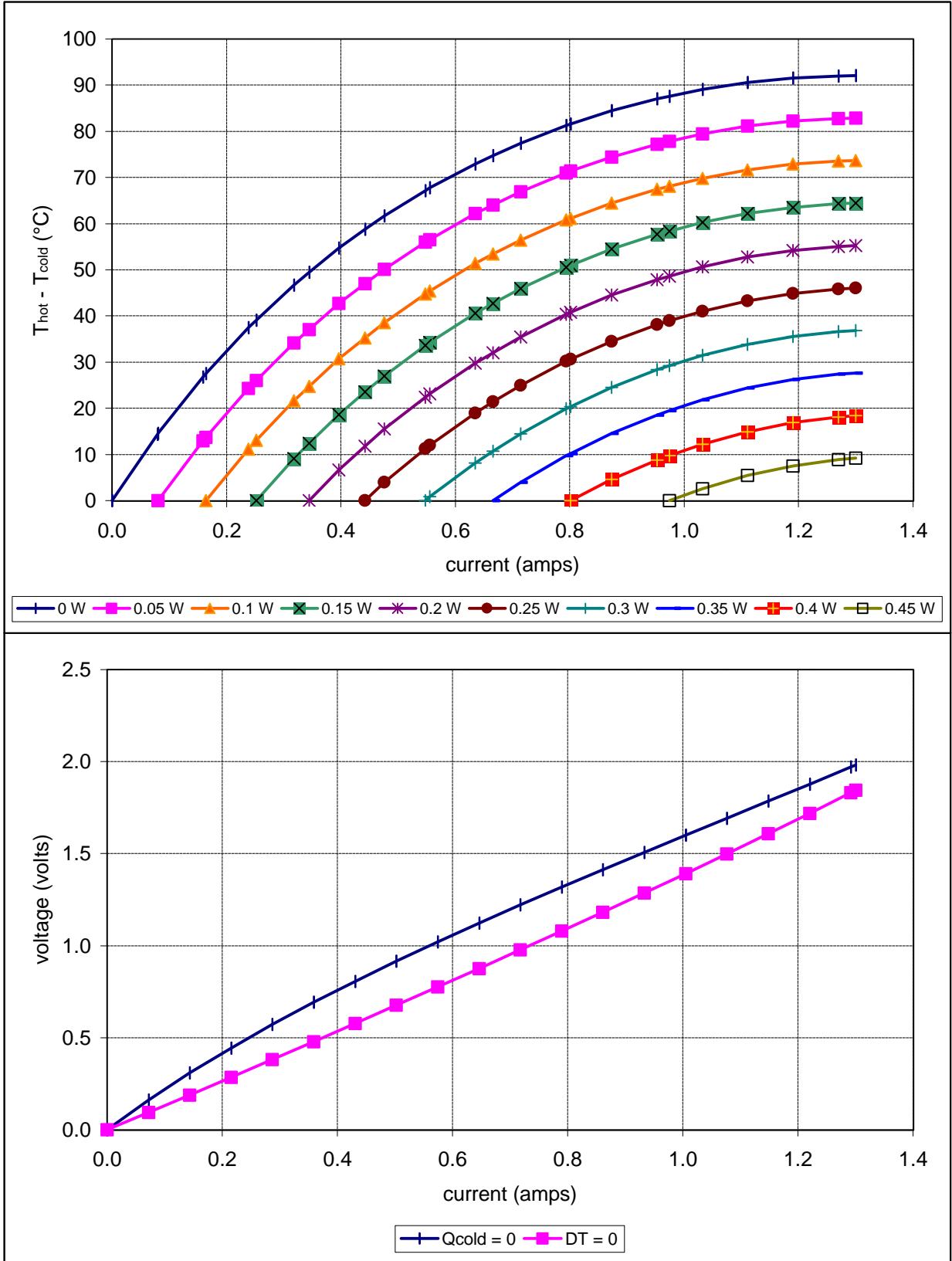
Unpotted TE-2-(17-4)-1.2 at a hot-side temperature of 25 °C
