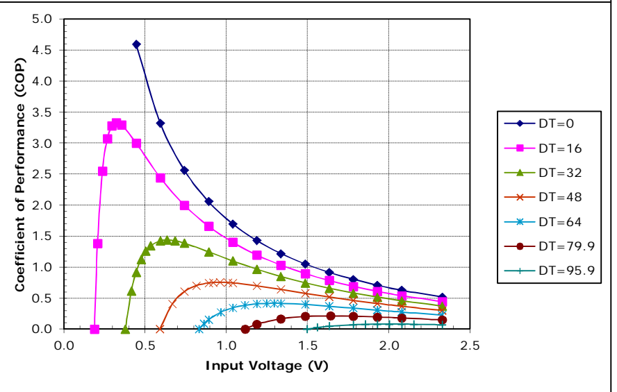
Unpotted TE-2-(17-4)-1.2 at a hot-side temperature of 50 °C
