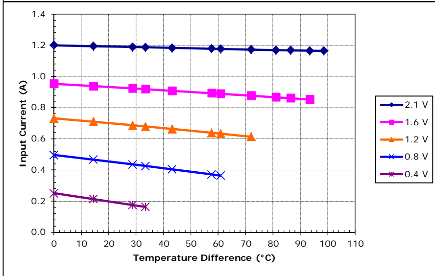
Unpotted TE-2-(17-4)-1.2 at a hot-side temperature of 30 °C
