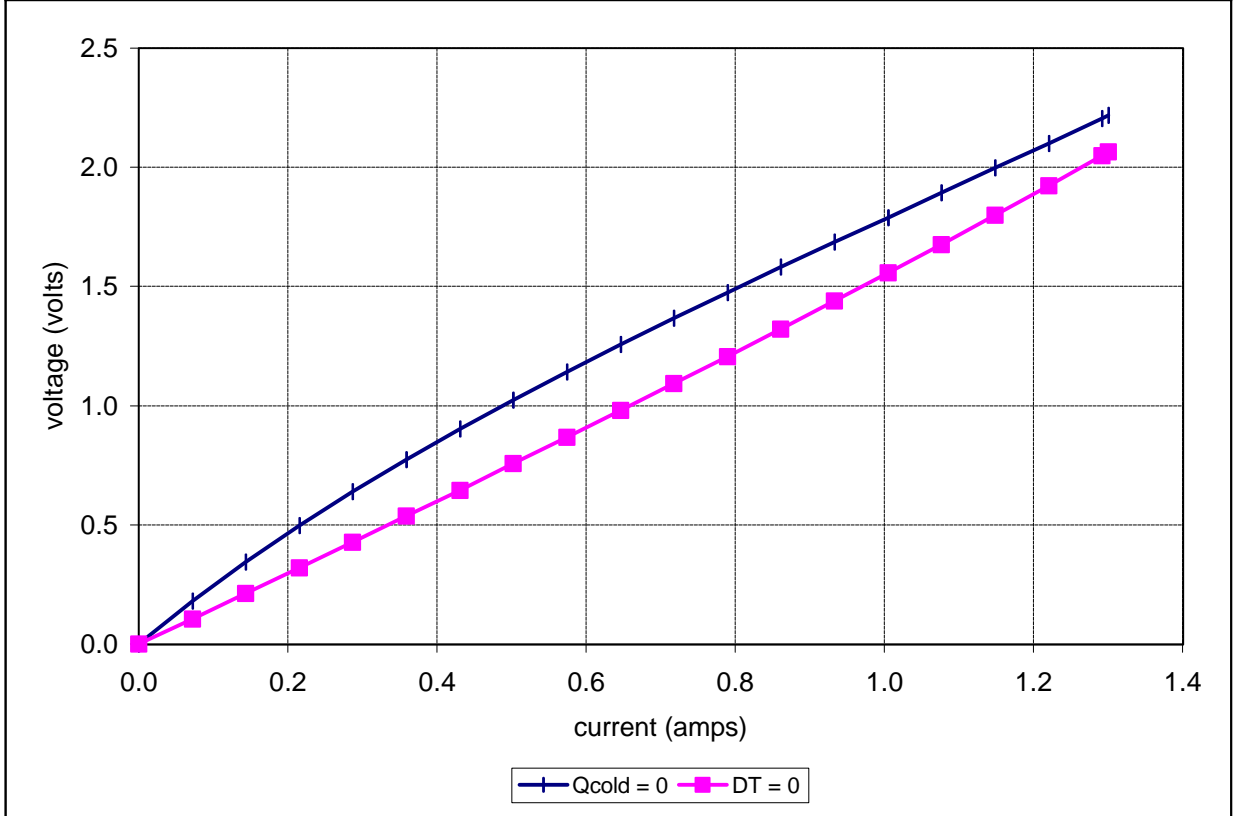
Unpotted TE-2-(17-4)-1.2 at a hot-side temperature of 50 °C
