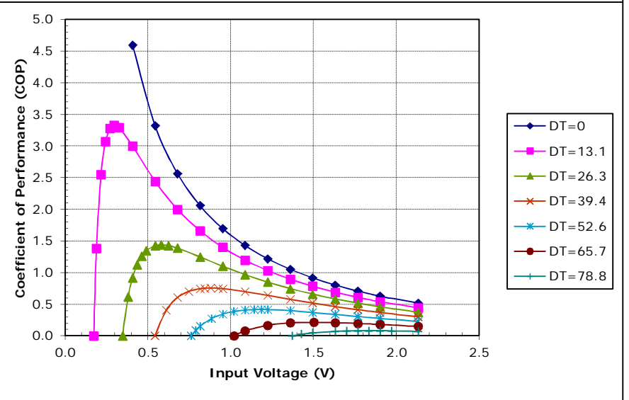
Potted TE-2-(17-4)-1.2 at a hot-side temperature of 30 °C
