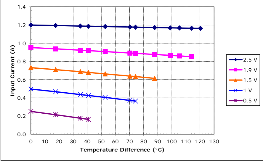
Unpotted TE-2-(17-4)-1.2 at a hot-side temperature of 70 °C
