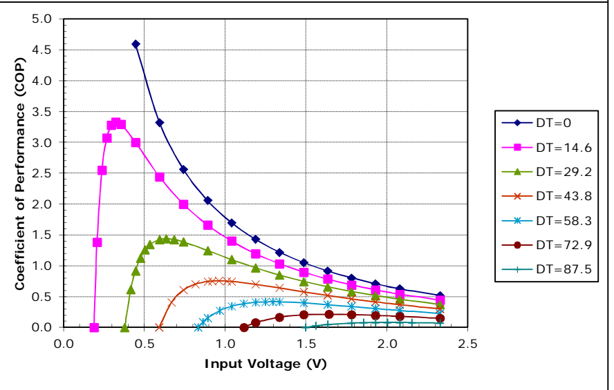
Potted TE-2-(17-4)-1.2 at a hot-side temperature of 50 °C
