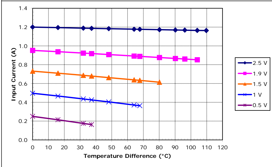
Potted TE-2-(17-4)-1.2 at a hot-side temperature of 70 °C
