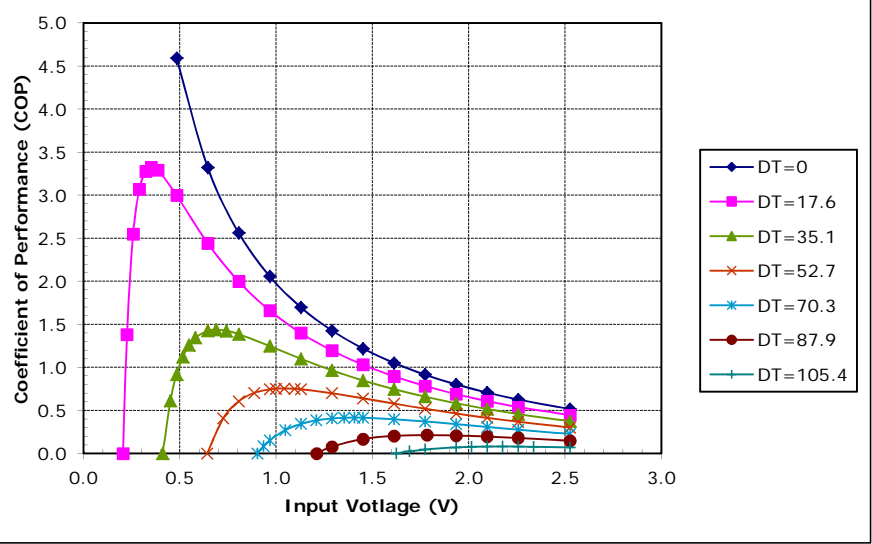
Unpotted TE-2-(17-4)-1.2 at a hot-side temperature of 70 °C
