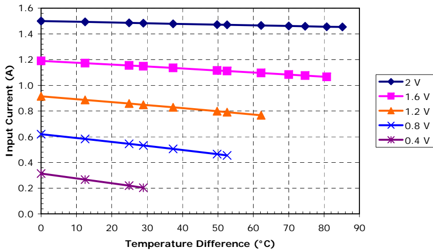
Potted TE-2-(17-4)-1.0 at a hot-side temperature of 30 °C
