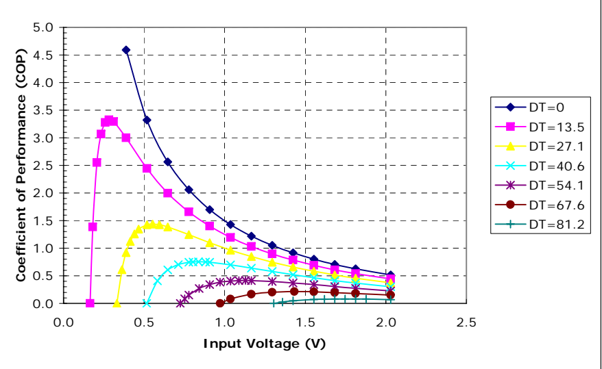
Unpotted TE-2-(17-4)-1.0 at a hot-side temperature of 30 °C
