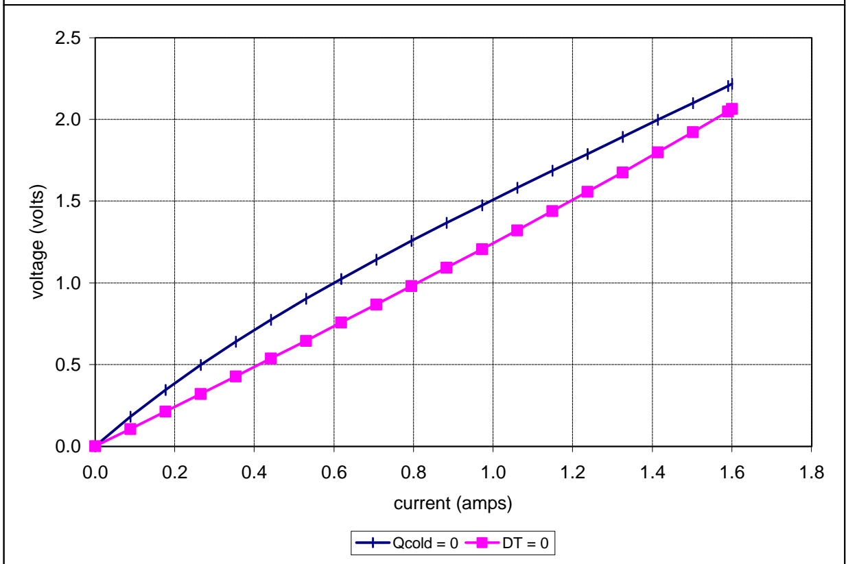
Unpotted TE-2-(17-4)-1.0 at a hot-side temperature of 50 °C
