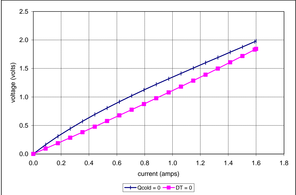
Unpotted TE-2-(17-4)-1.0 at a hot-side temperature of 25 °C
