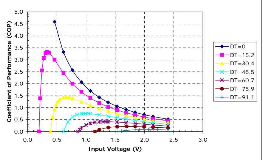
Potted TE-2-(17-4)-1.0 at a hot-side temperature of 70 °C
