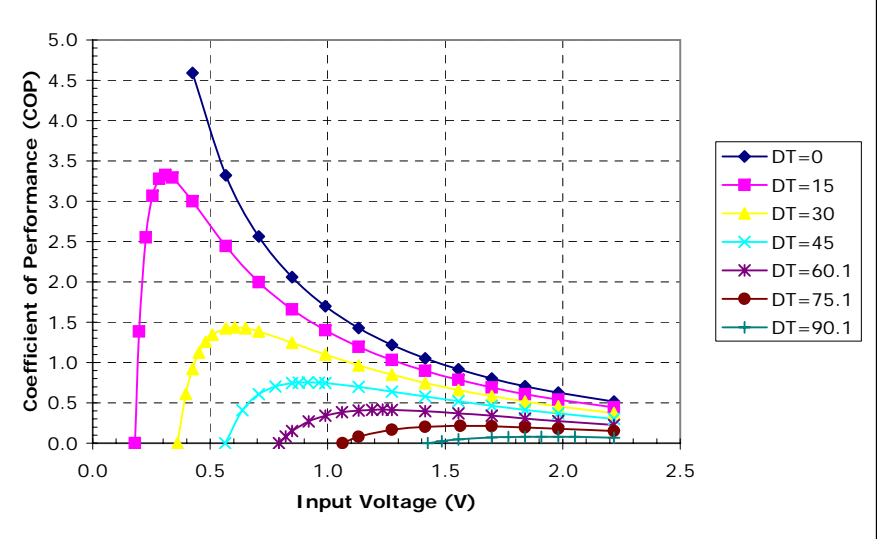
Unpotted TE-2-(17-4)-1.0 at a hot-side temperature of 50 °C
