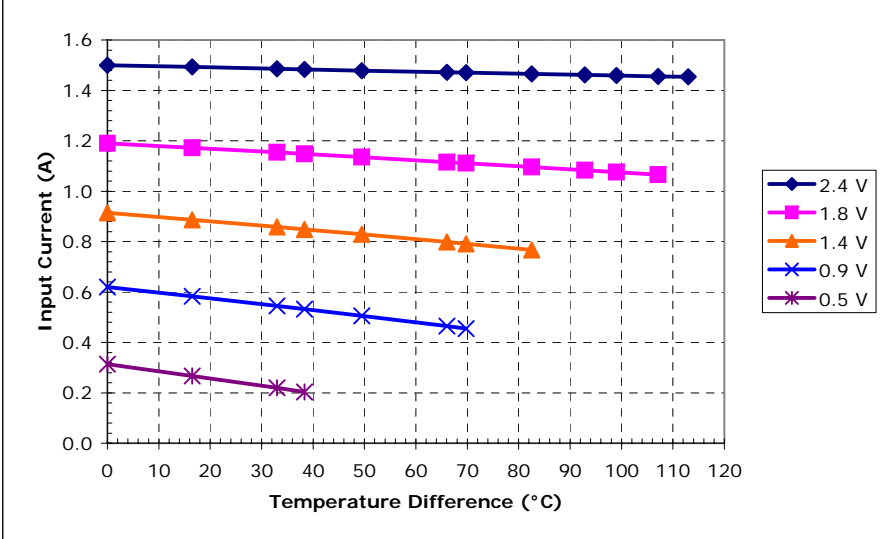
Unpotted TE-2-(17-4)-1.0 at a hot-side temperature of 70 °C
