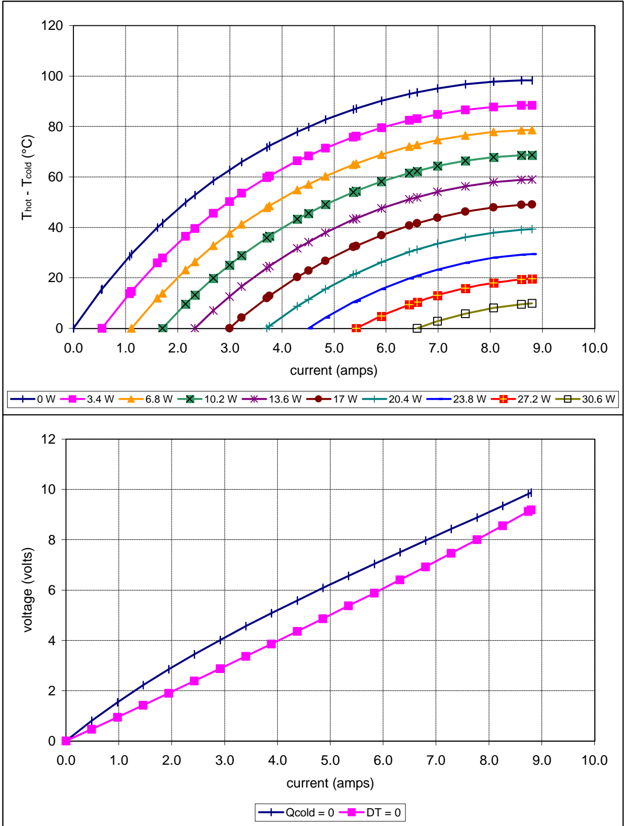
Unpotted TE-2-(127-127)-2.5 at a hot-side temperature of 50 °C
