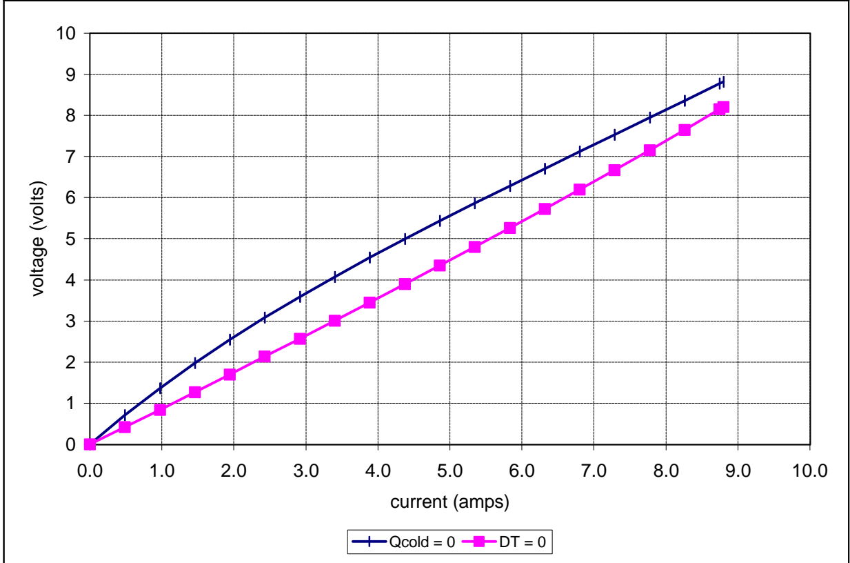
Unpotted TE-2-(127-127)-2.5 at a hot-side temperature of 25 °C
