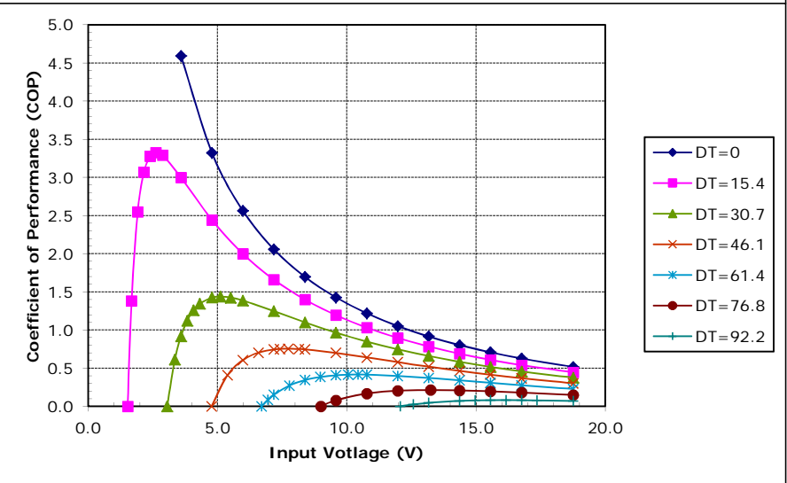
Unpotted TE-2-(127-127)-1.3 at a hot-side temperature of 70 °C
