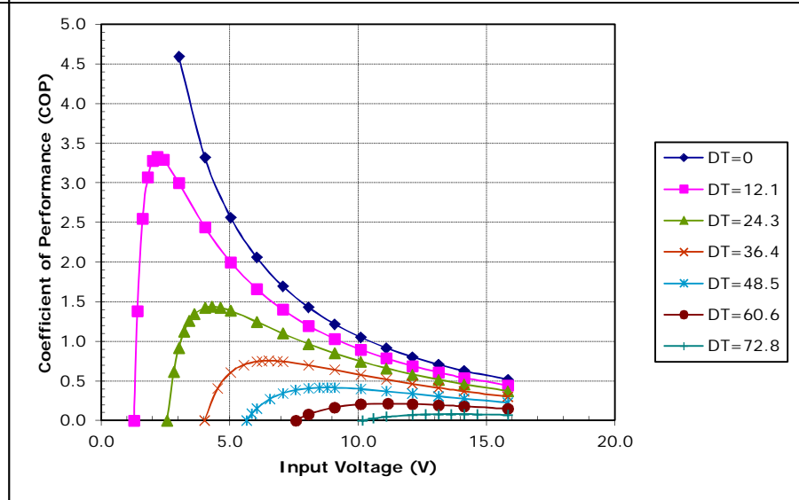
Potted TE-2-(127-127)-1.3 at a hot-side temperature of 30 °C
