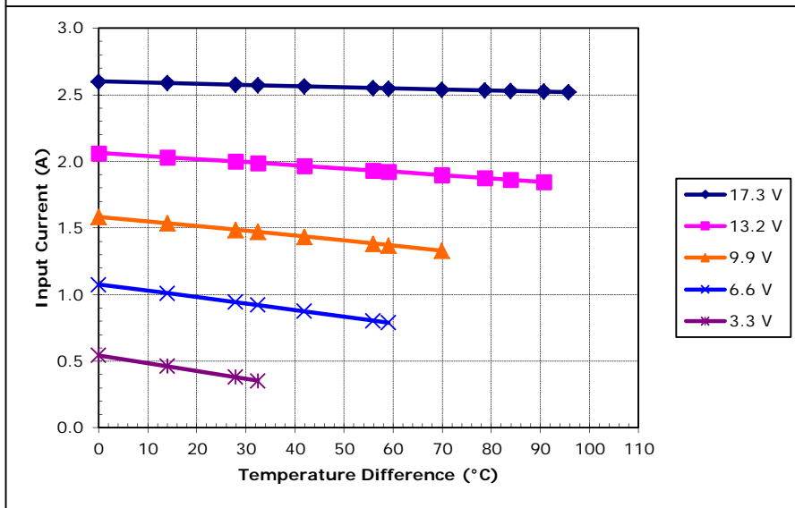
Unpotted TE-2-(127-127)-1.3 at a hot-side temperature of 50 °C
