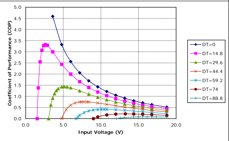
Potted TE-2-(127-127)-1.3 at a hot-side temperature of 70 °C
