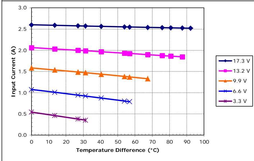
Potted TE-2-(127-127)-1.3 at a hot-side temperature of 50 °C
