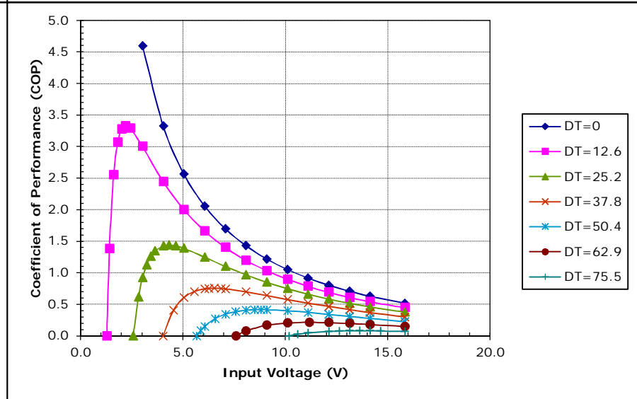
Unpotted TE-2-(127-127)-1.3 at a hot-side temperature of 30 °C
