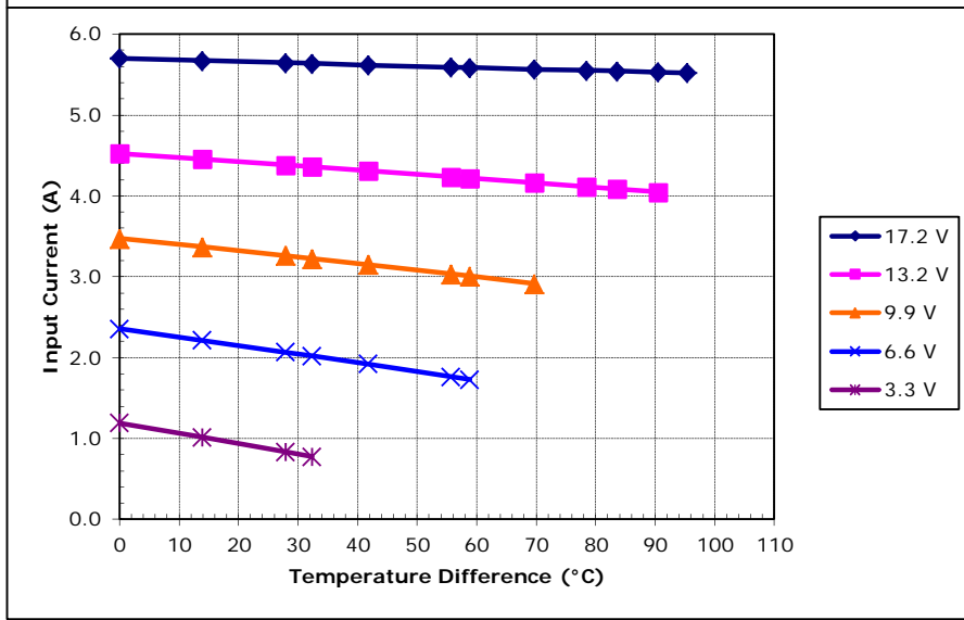
Unpotted TE-2-(127-127)-1.15 at a hot-side temperature of 50 °C
