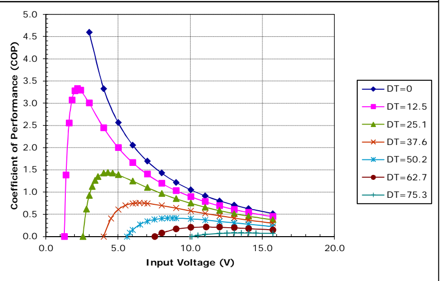
Unpotted TE-2-(127-127)-1.15 at a hot-side temperature of 30 °C
