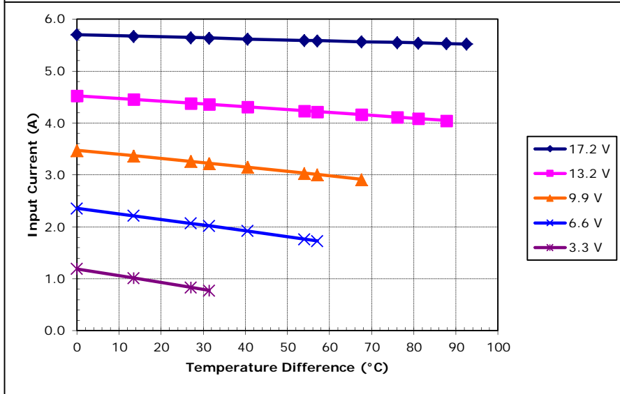
Potted TE-2-(127-127)-1.15 at a hot-side temperature of 50 °C
