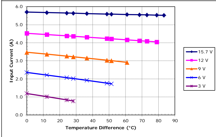
Potted TE-2-(127-127)-1.15 at a hot-side temperature of 30 °C
