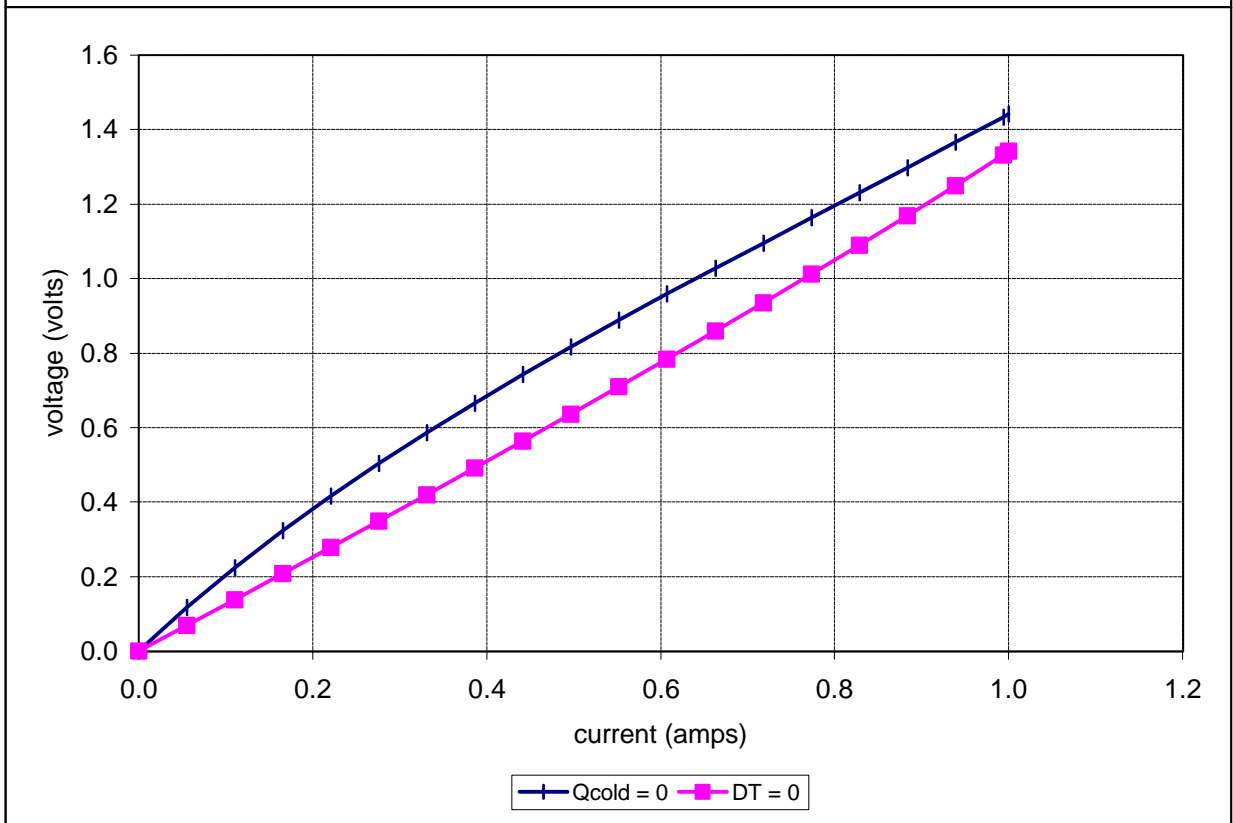
Unpotted TE-2-(11-4)-1.5 at a hot-side temperature of 50 °C
