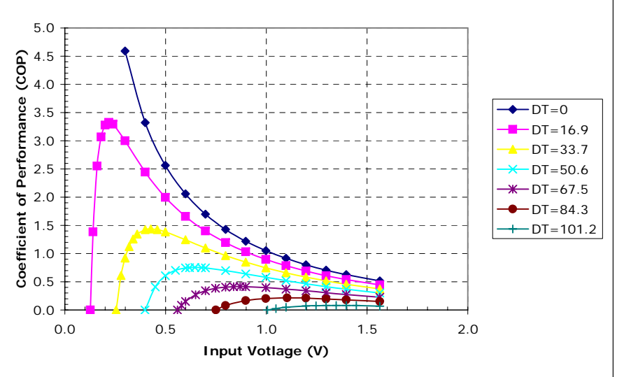
Unpotted TE-2-(11-4)-1.5 at a hot-side temperature of 70 °C
