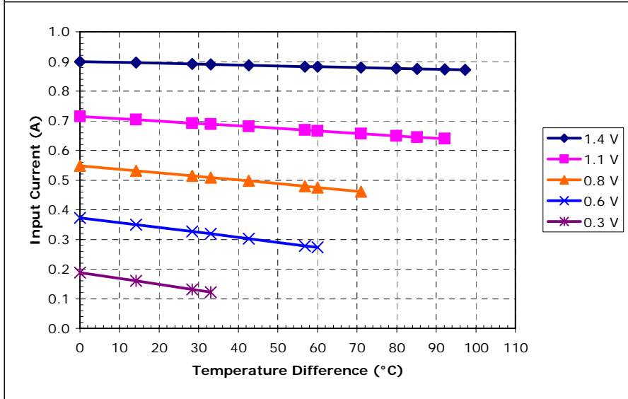
Potted TE-2-(11-4)-1.5 at a hot-side temperature of 50 °C
