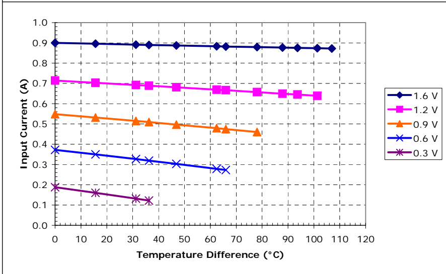
Potted TE-2-(11-4)-1.5 at a hot-side temperature of 70 °C
