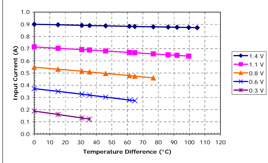
Unpotted TE-2-(11-4)-1.5 at a hot-side temperature of 50 °C
