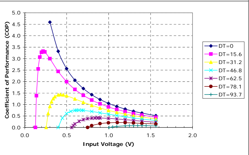
Potted TE-2-(11-4)-1.5 at a hot-side temperature of 70 °C
