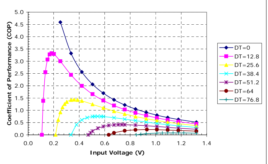
Potted TE-2-(11-4)-1.5 at a hot-side temperature of 30 °C
