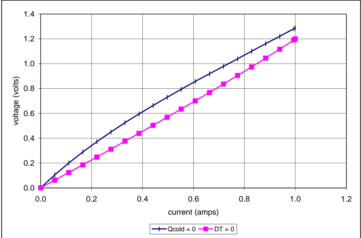
Unpotted TE-2-(11-4)-1.5 at a hot-side temperature of 25 °C
