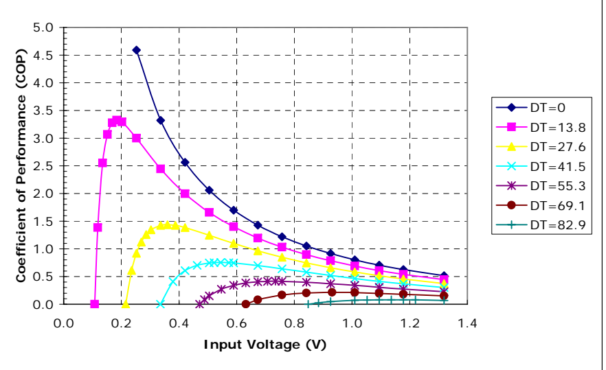
Unpotted TE-2-(11-4)-1.5 at a hot-side temperature of 30 °C
