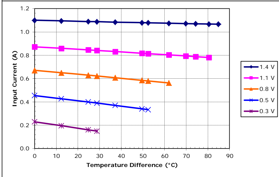
Potted TE-2-(11-4)-1.2 at a hot-side temperature of 30 °C
