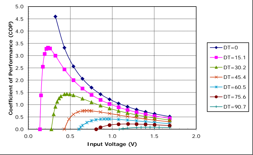
Potted TE-2-(11-4)-1.2 at a hot-side temperature of 70 °C
