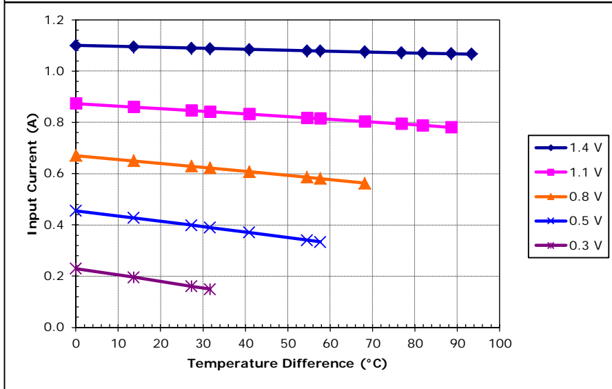
Unpotted TE-2-(11-4)-1.2 at a hot-side temperature of 30 °C
