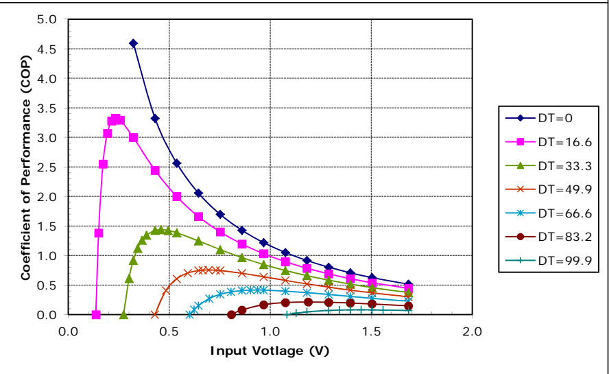
Unpotted TE-2-(11-4)-1.2 at a hot-side temperature of 70 °C
