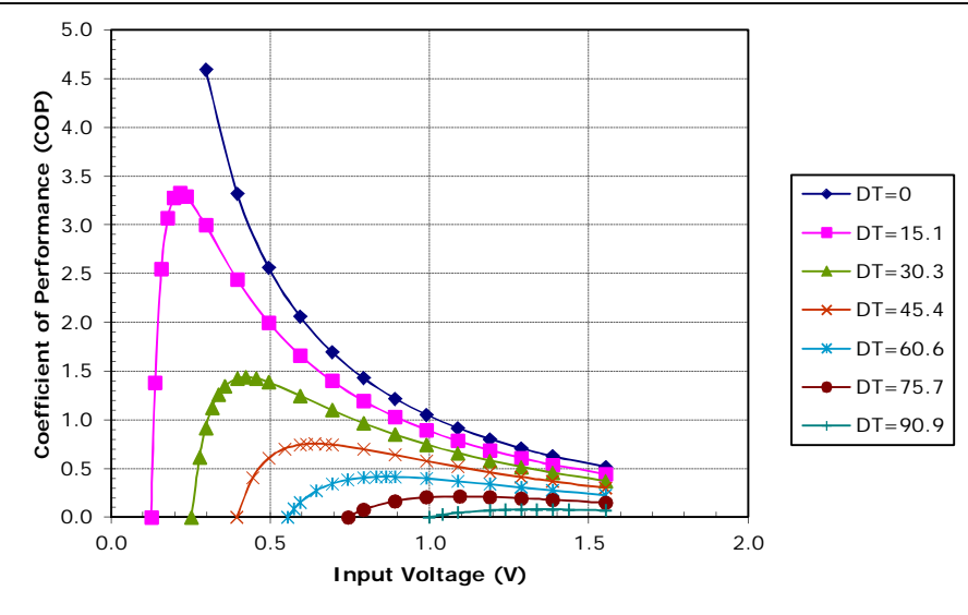
Unpotted TE-2-(11-4)-1.2 at a hot-side temperature of 50 °C
