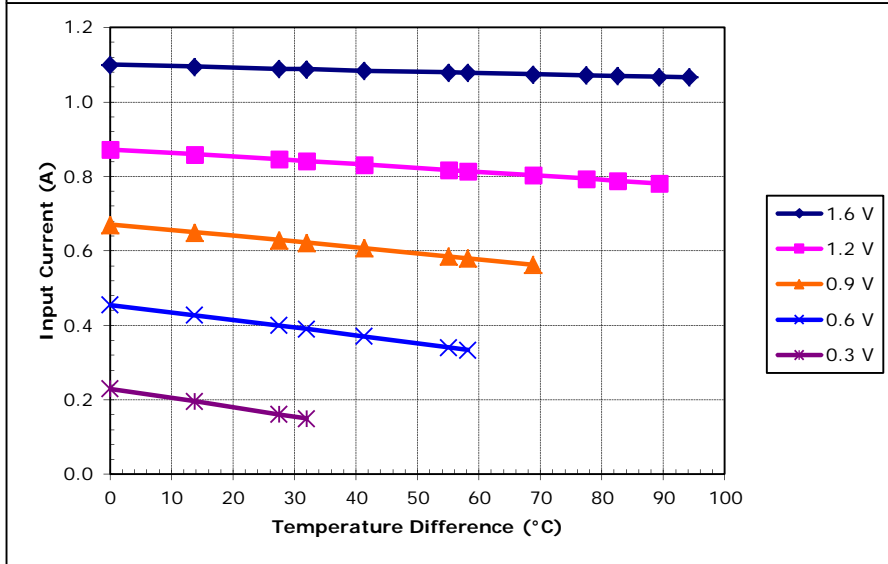
Potted TE-2-(11-4)-1.2 at a hot-side temperature of 50 °C
