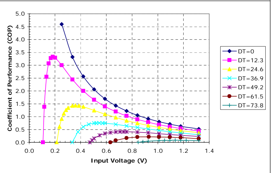
Potted TE-2-(11-4)-1.0 at a hot-side temperature of 30 °C
