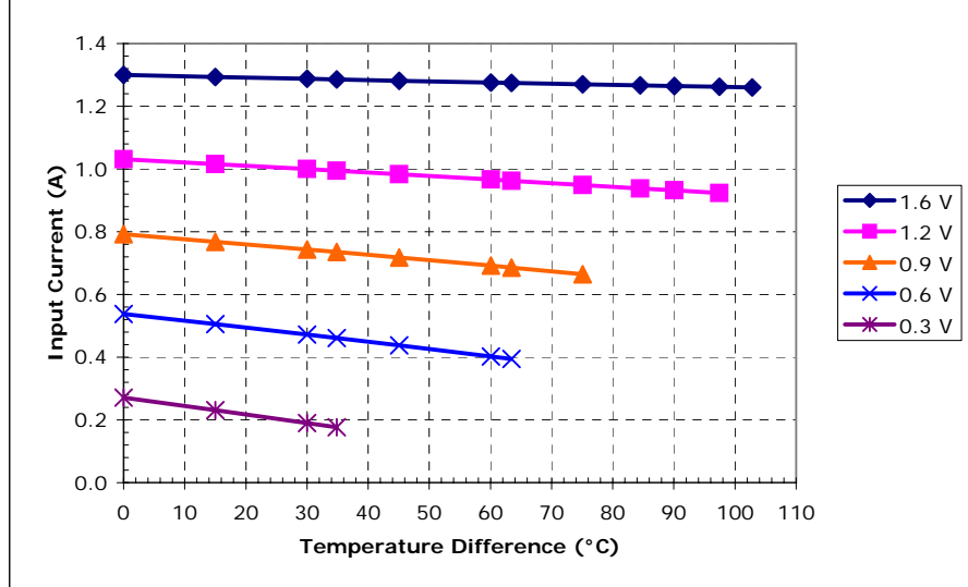
Potted TE-2-(11-4)-1.0 at a hot-side temperature of 70 °C
