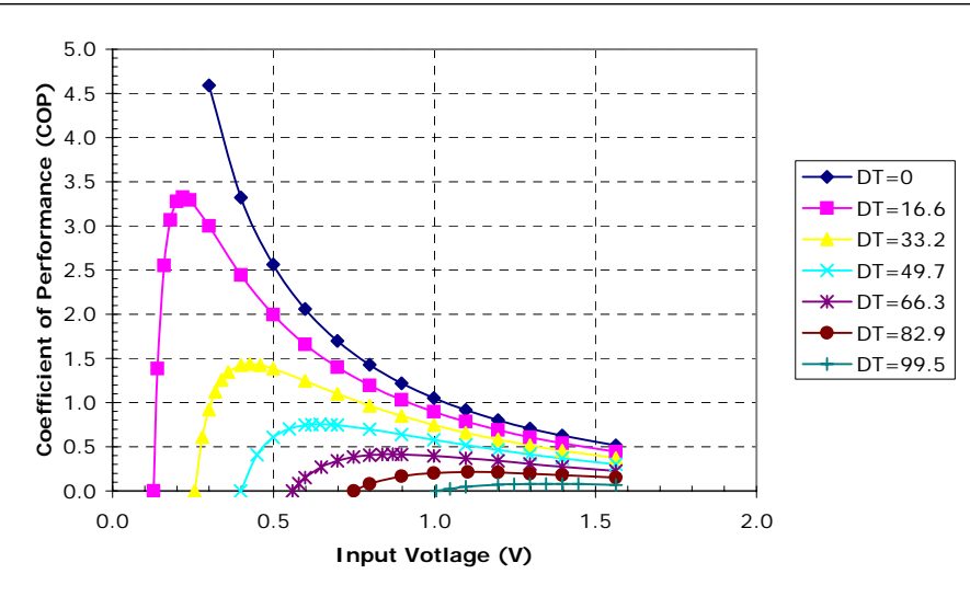
Unpotted TE-2-(11-4)-1.0 at a hot-side temperature of 70 °C
