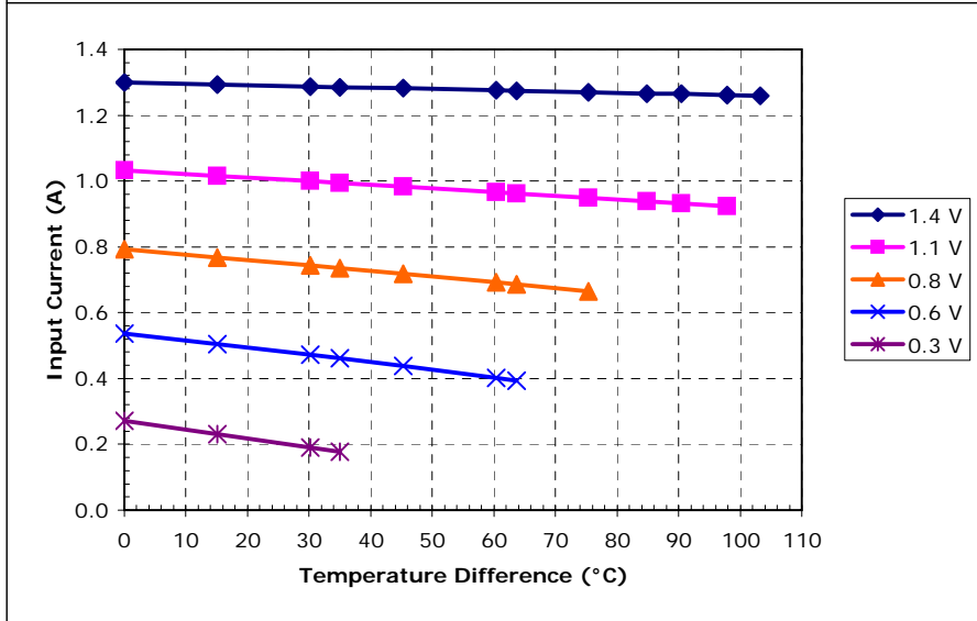
Unpotted TE-2-(11-4)-1.0 at a hot-side temperature of 50 °C
