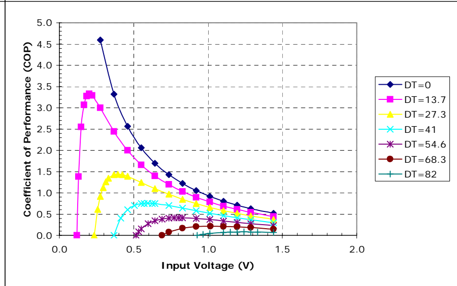
Potted TE-2-(11-4)-1.0 at a hot-side temperature of 50 °C
