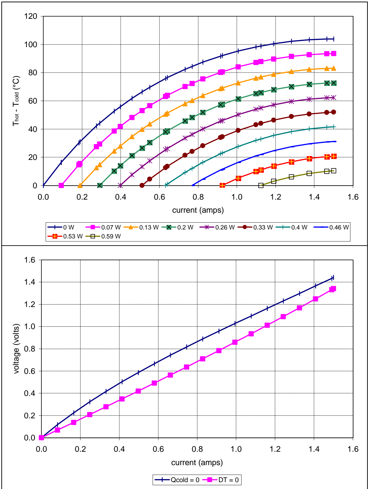
Unpowered TE-2-(11-4)-1.0 at a hot-side temperature of 50 °C
