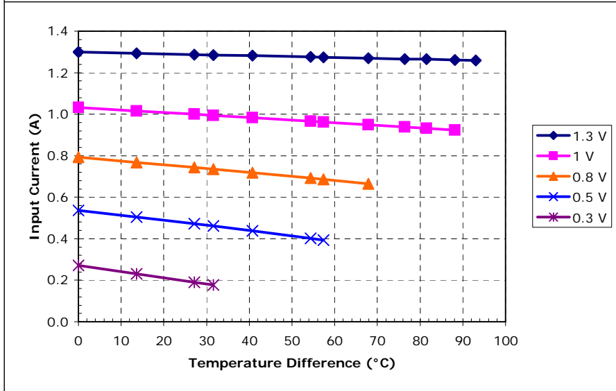
Unpotted TE-2-(11-4)-1.0 at a hot-side temperature of 30 °C
