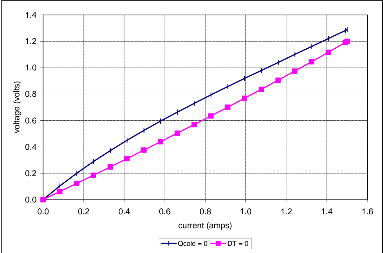
Unpotted TE-2-(11-4)-1.0 at a hot-side temperature of 25 °C
