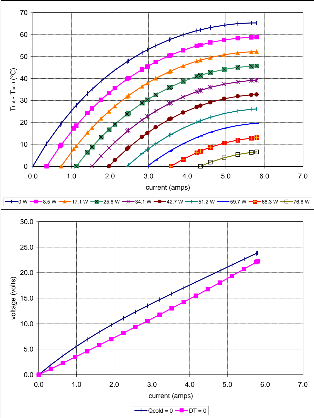
Potted TE-195-1.0-0.8 at a hot-side temperature of 25 °C
