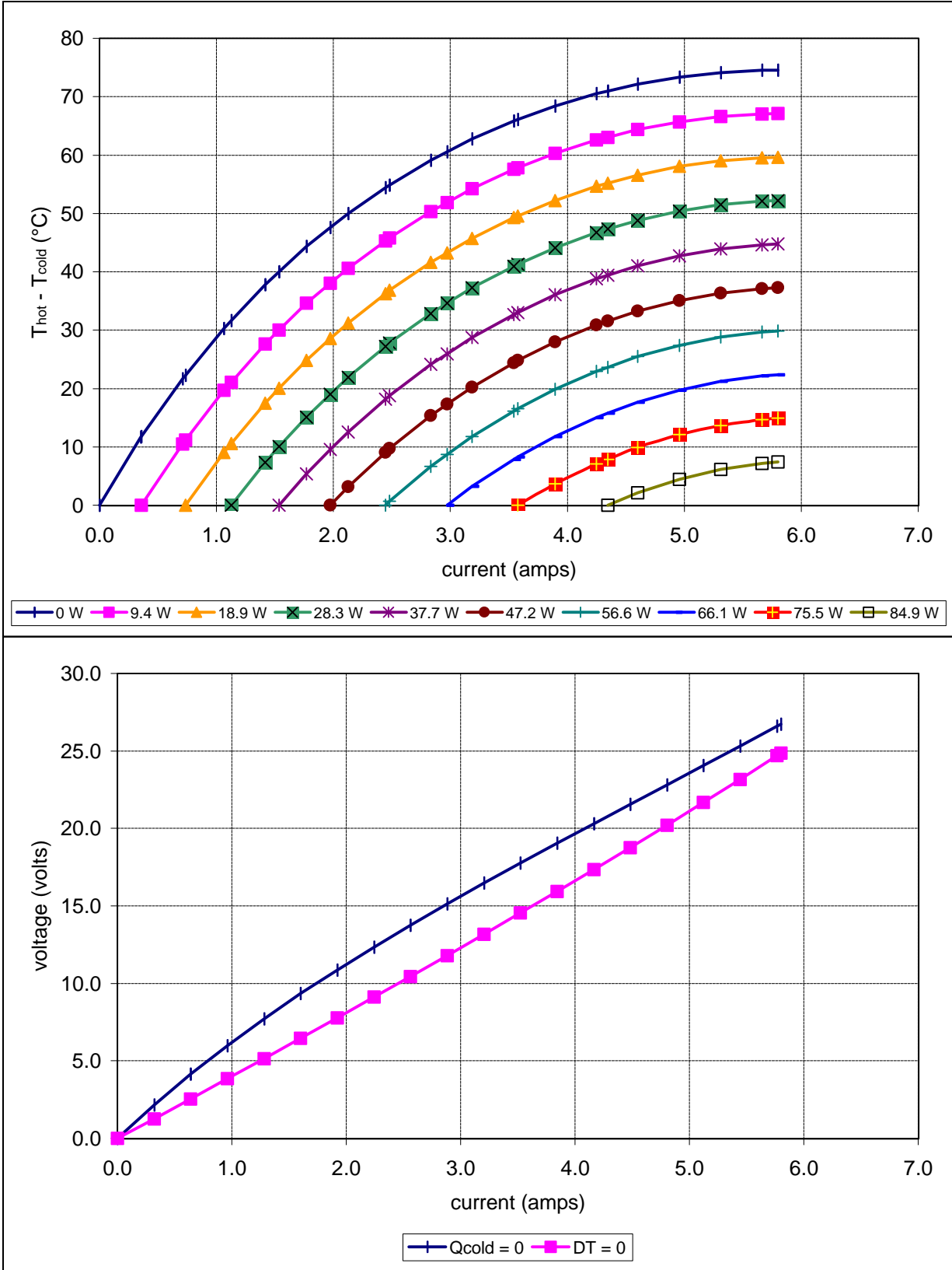
Potted TE-195-1.0-0.8 at a hot-side temperature of 50 °C
