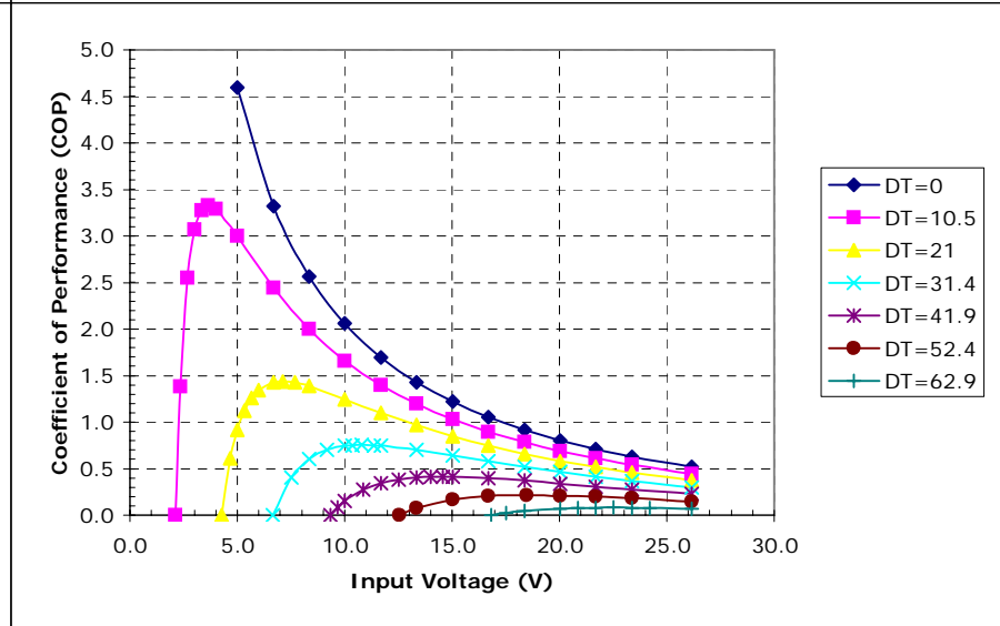
Potted TE-195-1.0-0.8 at a hot-side temperature of 50 °C
