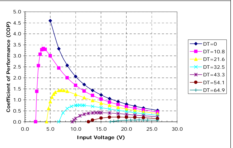
Unpotted TE-195-1.0-0.8 at a hot-side temperature of 50 °C
