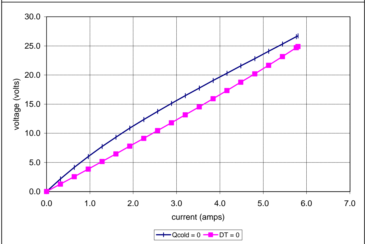
Unpotted TE-195-1.0-0.8 at a hot-side temperature of 50 °C
