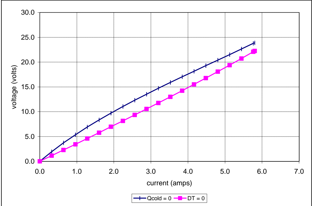
Unpotted TE-195-1.0-0.8 at a hot-side temperature of 25 °C
