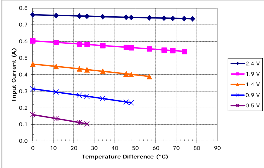
Unpotted TE-18-0.45-1.3 at a hot-side temperature of 50 °C
