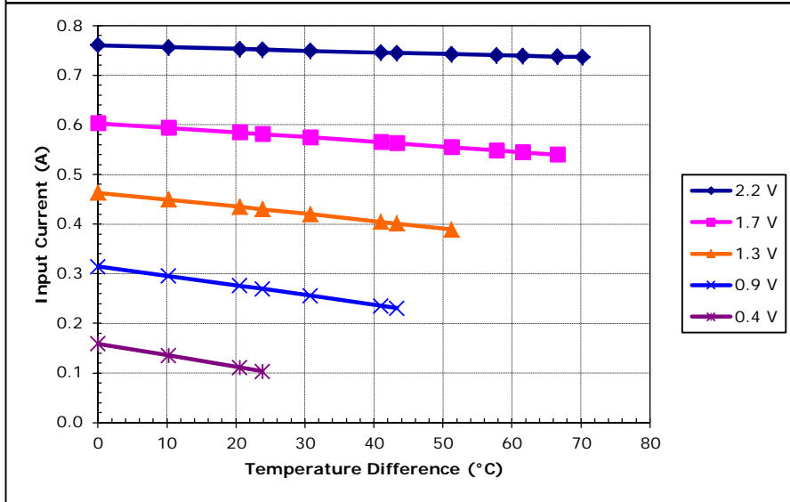
Unpotted TE-18-0.45-1.3 at a hot-side temperature of 30 °C
