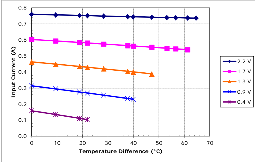
Potted TE-18-0.45-1.3 at a hot-side temperature of 30 °C
