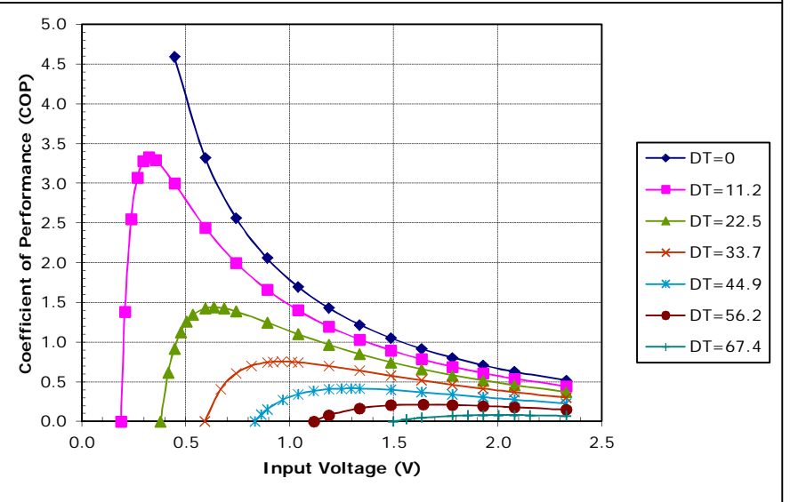
Unpotted TE-17-2.0-2.5 at a hot-side temperature of 50 °C
