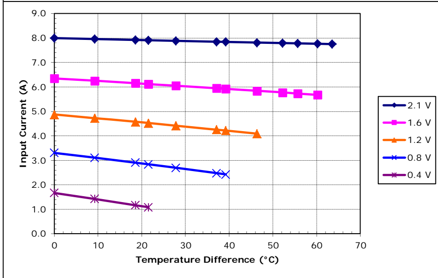
Potted TE-17-2.0-2.5 at a hot-side temperature of 30 °C
