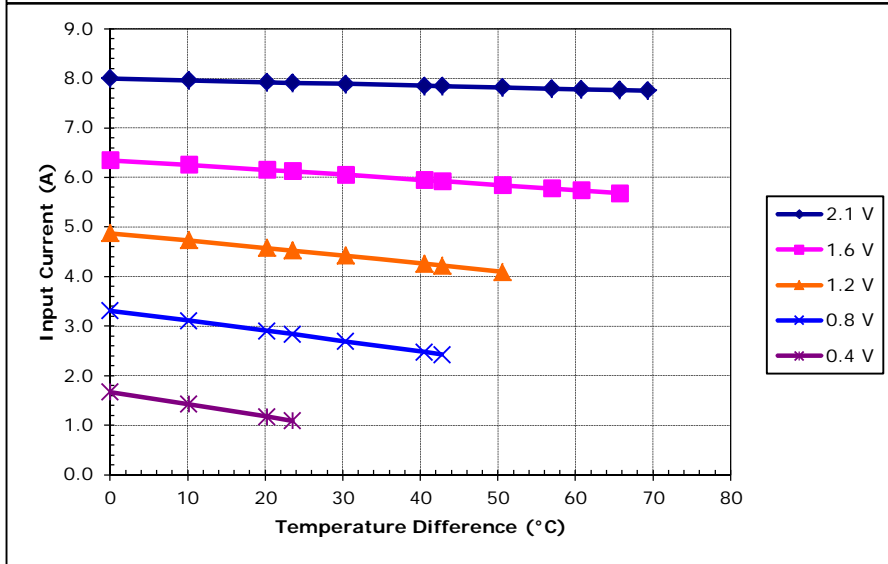
Unpotted TE-17-2.0-2.5 at a hot-side temperature of 30 °C
