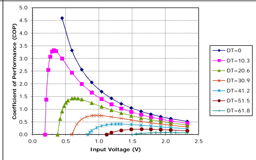
Potted TE-17-2.0-2.5 at a hot-side temperature of 50 °C
