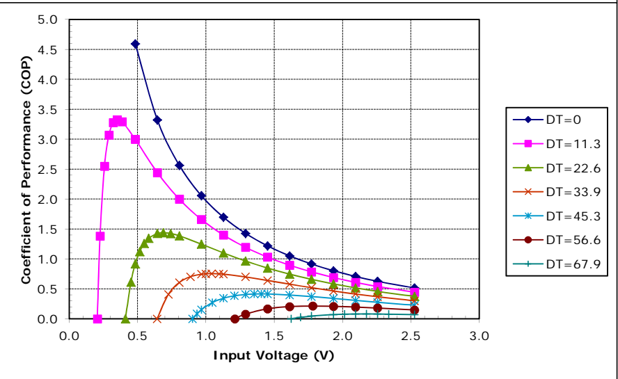
Potted TE-17-2.0-2.5 at a hot-side temperature of 70 °C
