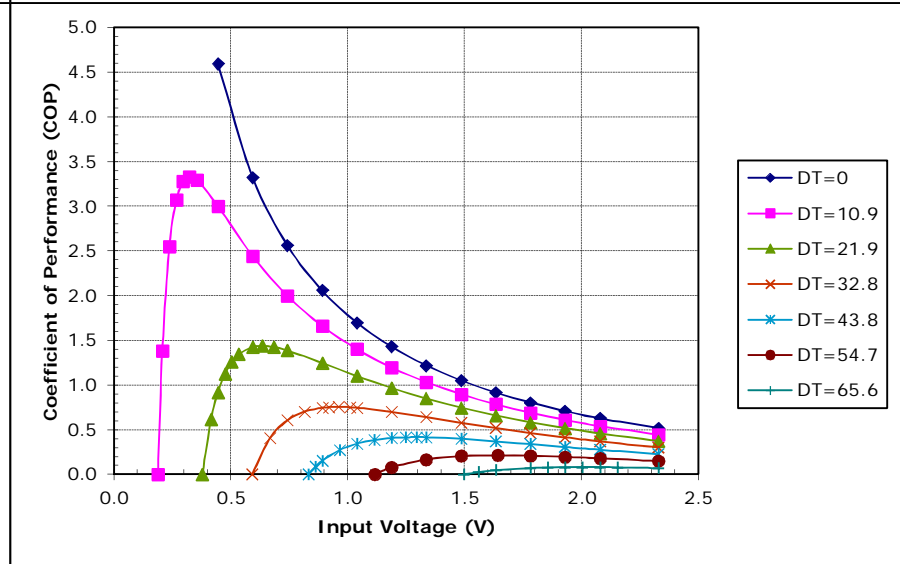
Unpotted TE-17-1.4-1.15 at a hot-side temperature of 50 °C
