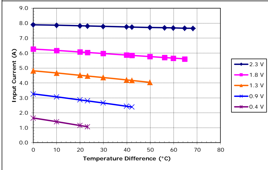
Potted TE-17-1.4-1.15 at a hot-side temperature of 50 °C
