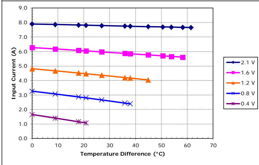
Potted TE-17-1.4-1.15 at a hot-side temperature of 30 °C
