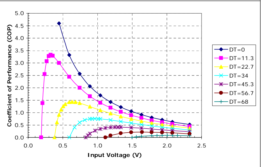
Unpotted TE-17-1.0-2.5 at a hot-side temperature of 50 °C
