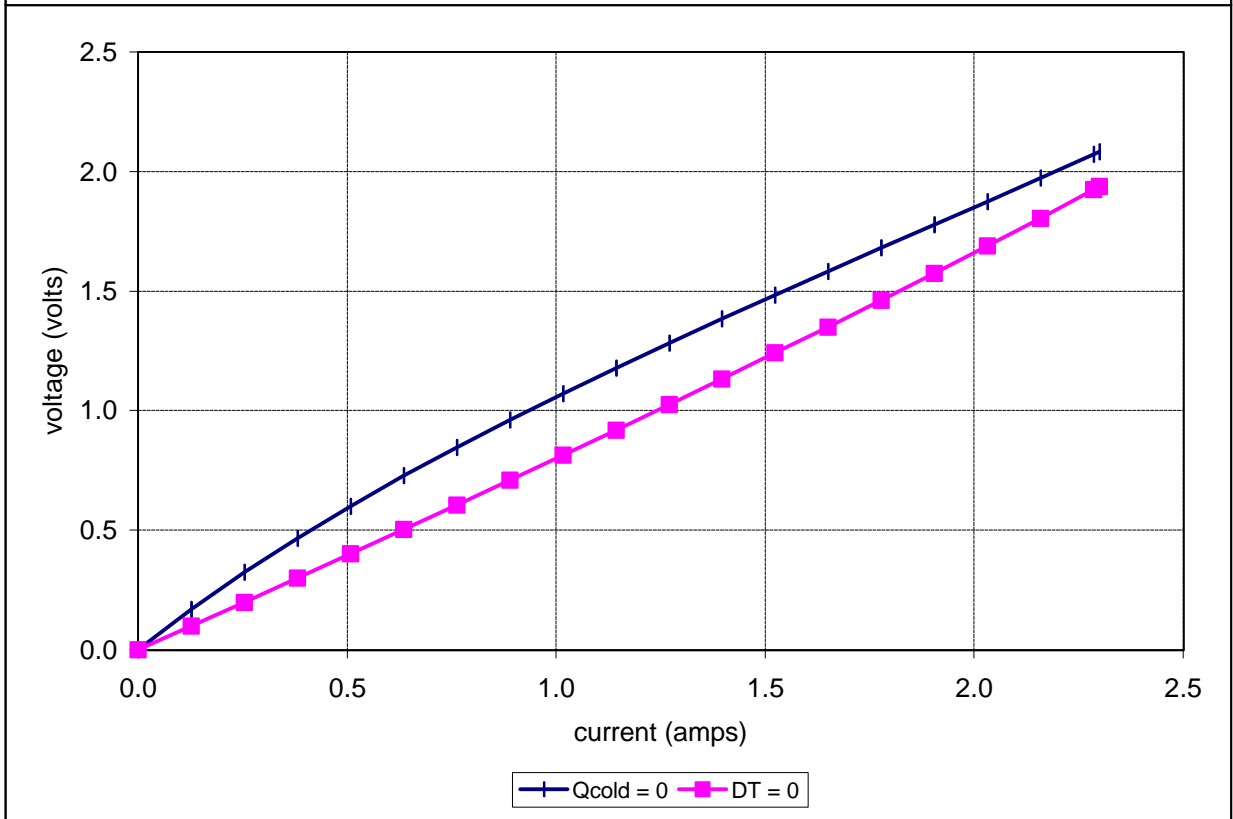
Potted TE-17-1.0-2.0 at a hot-side temperature of 25 °C
