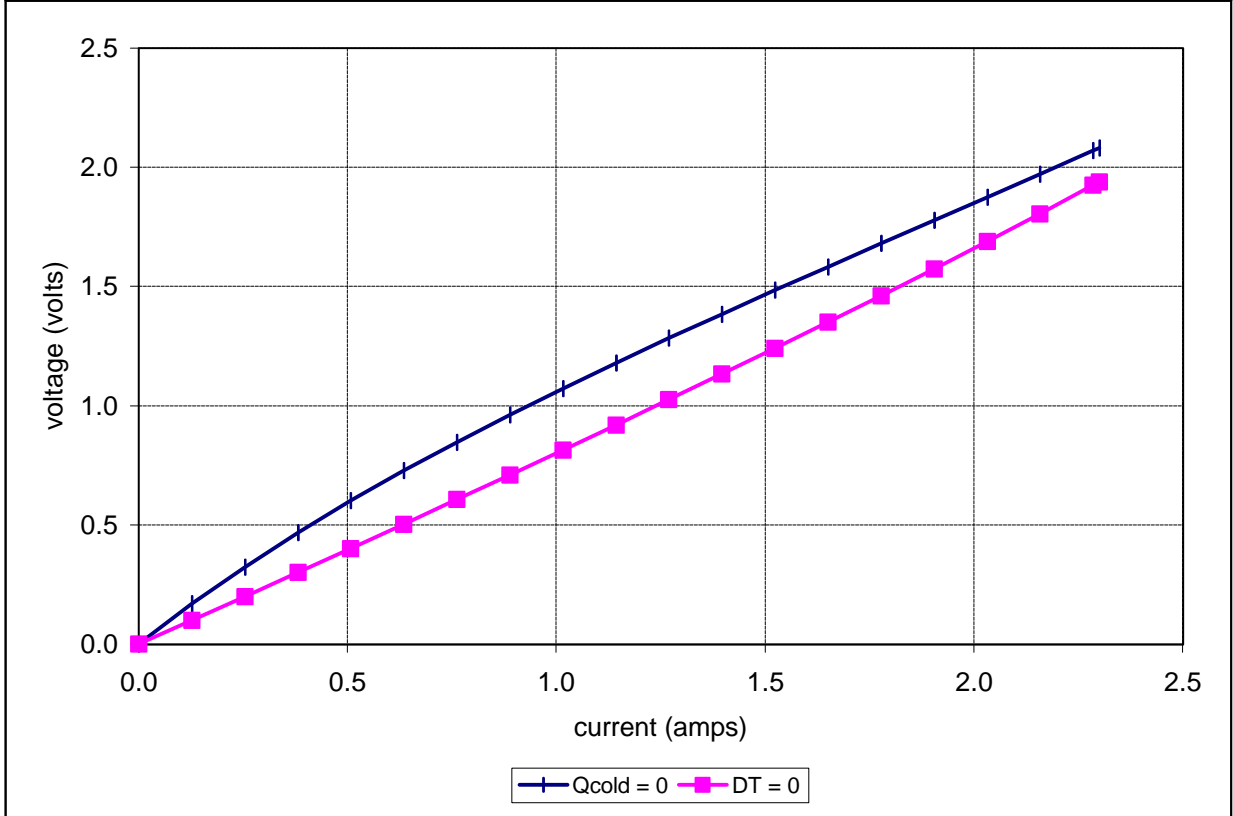
Unpotted TE-17-1.0-2.0 at a hot-side temperature of 25 °C
