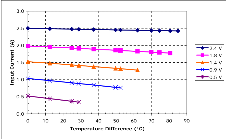
Unpotted TE-17-1.0-2.0 at a hot-side temperature of 70 °C
