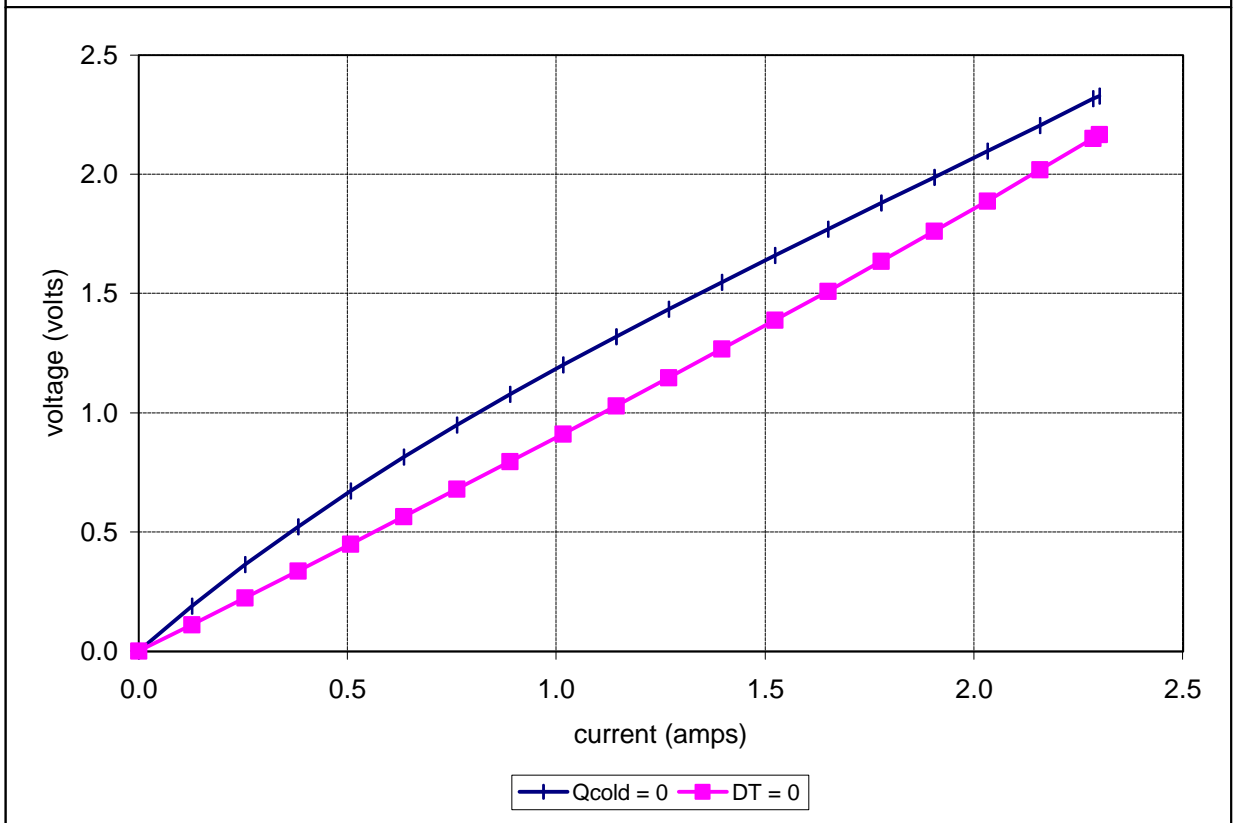
Unpotted TE-17-1.0-2.0 at a hot-side temperature of 50 °C
