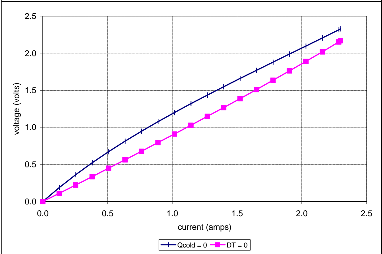
Potted TE-17-1.0-2.0 at a hot-side temperature of 50 °C
