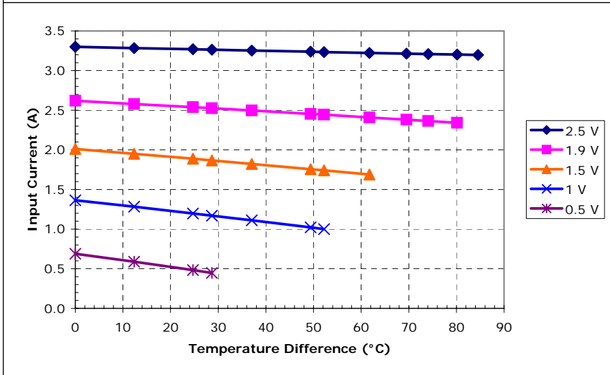
Unpotted TE-17-1.0-1.5 at a hot-side temperature of 70 °C
