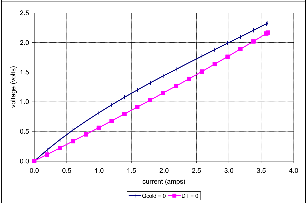
Potted TE-17-1.0-1.3 at a hot-side temperature of 50 °C
