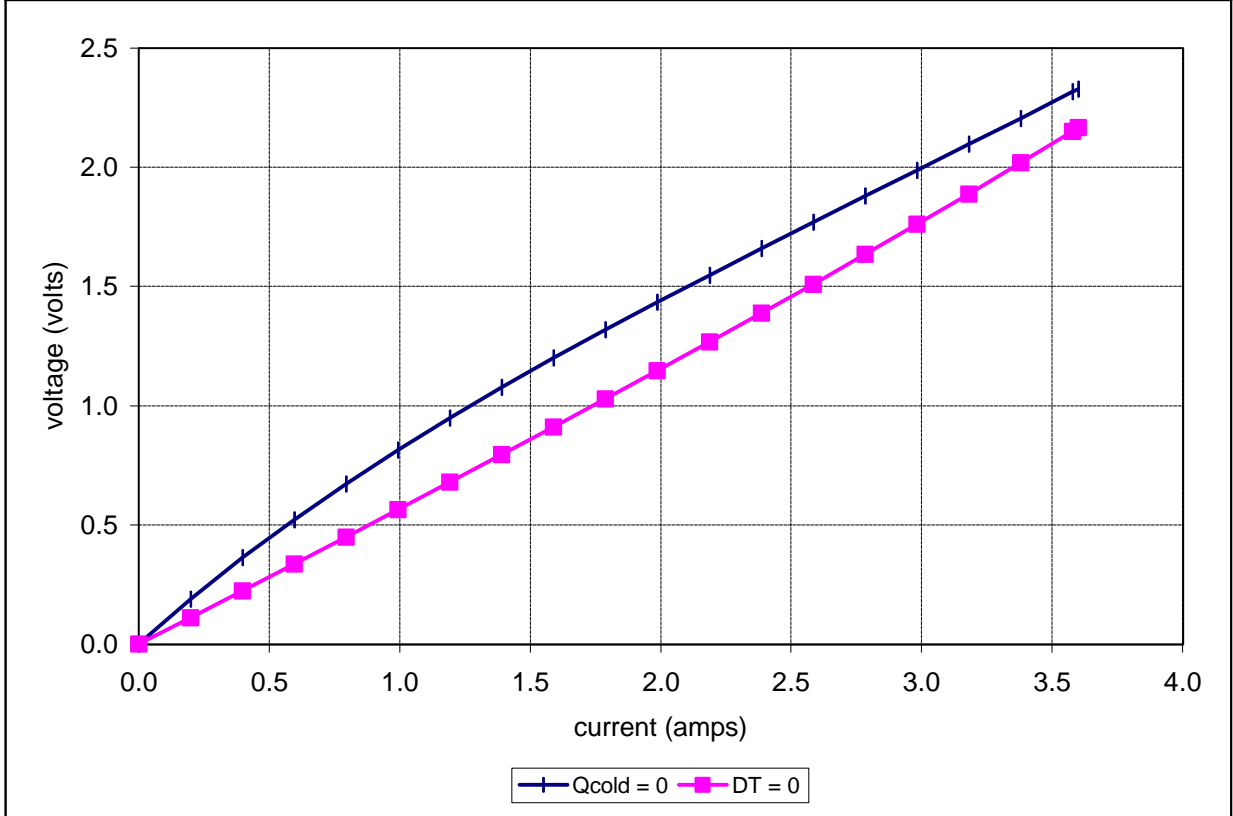
Unpotted TE-17-1.0-1.3 at a hot-side temperature of 50 °C
