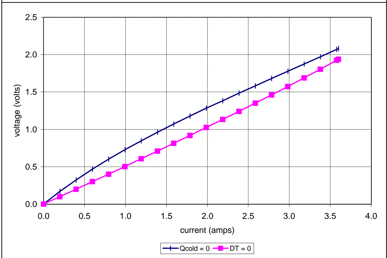
Unpotted TE-17-1.0-1.3 at a hot-side temperature of 25 °C
