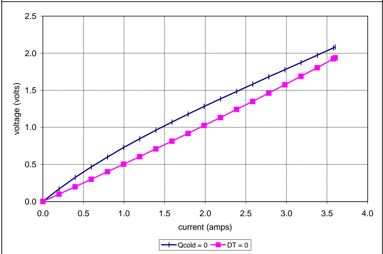
Potted TE-17-1.0-1.3 at a hot-side temperature of 25 °C
