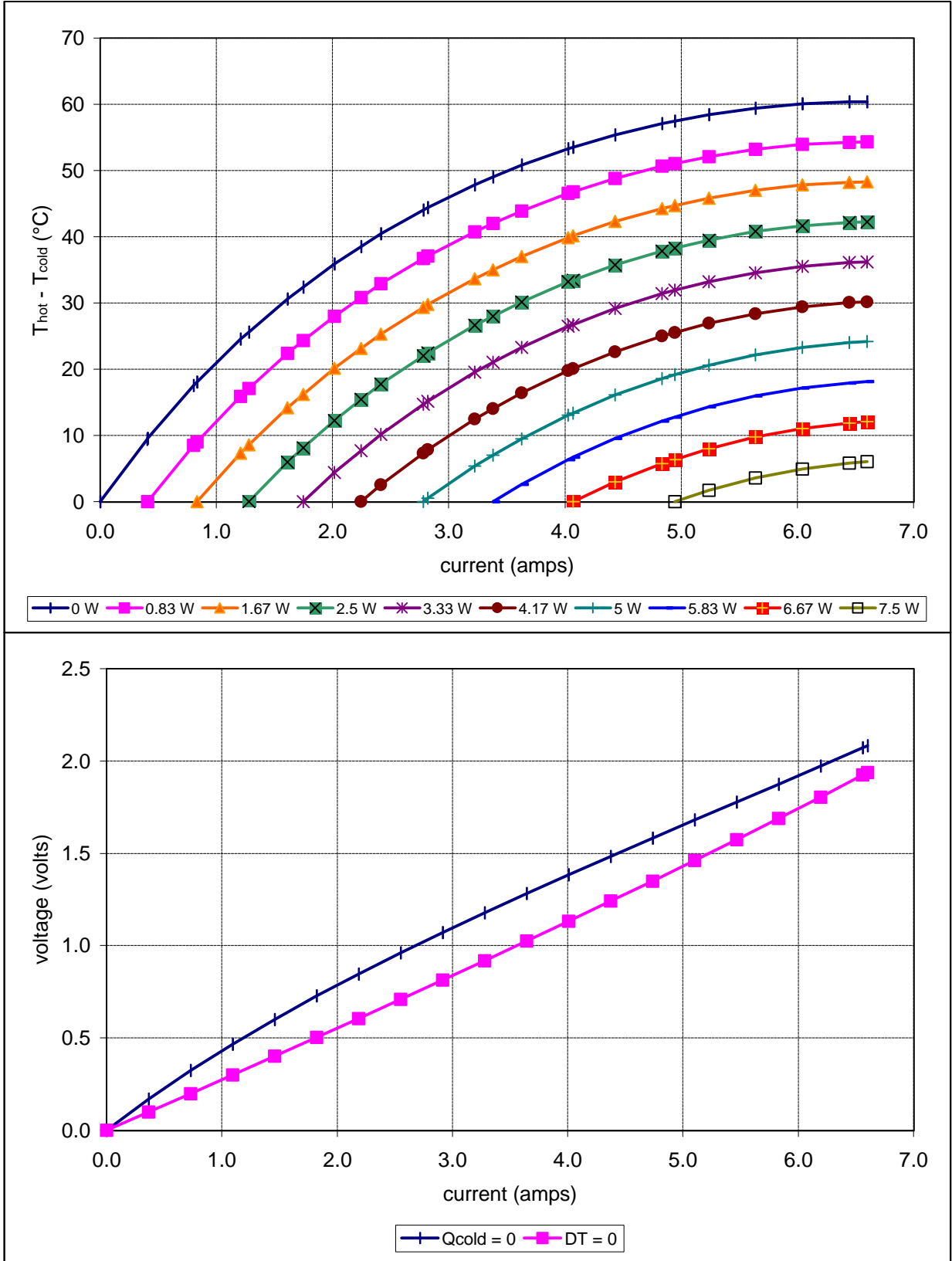
Potted TE-17-1.0-0.7 at a hot-side temperature of 25 °C
