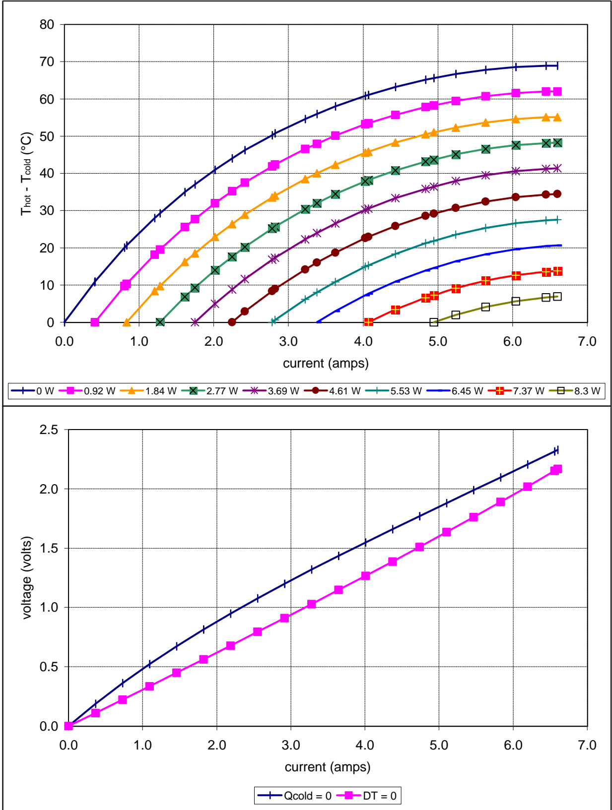
Potted TE-17-1.0-0.7 at a hot-side temperature of 50 °C
