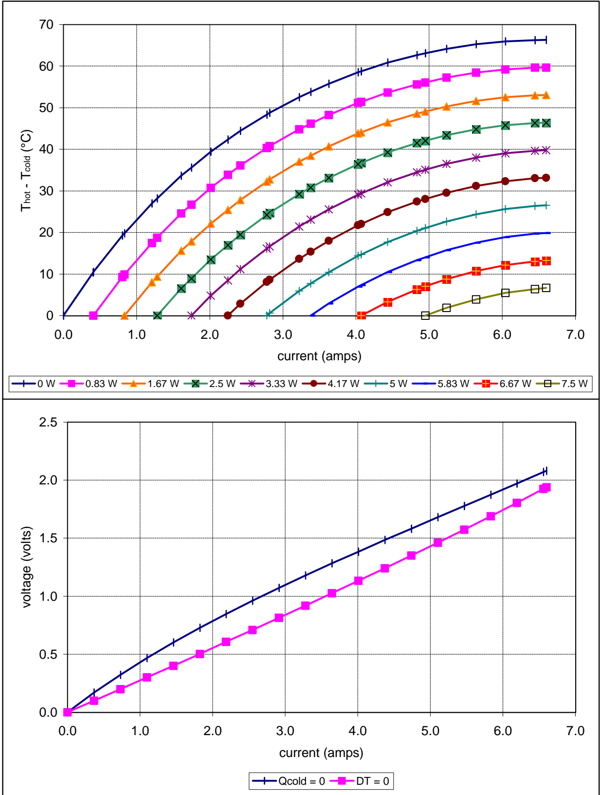
Unpotted TE-17-1.0-0.7 at a hot-side temperature of 25 °C
