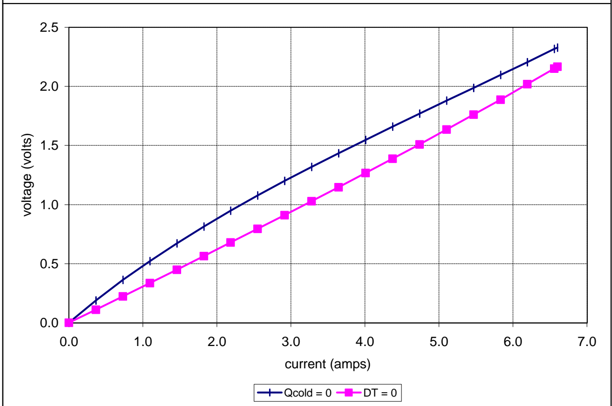
Unpotted TE-17-1.0-0.7 at a hot-side temperature of 50 °C
