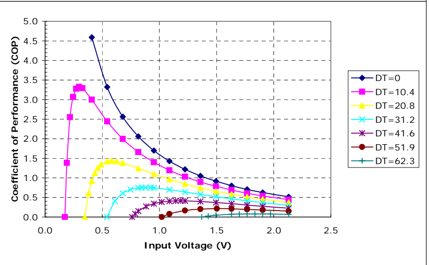
Unpotted TE-17-0.6-1.5 at a hot-side temperature of 30 °C
