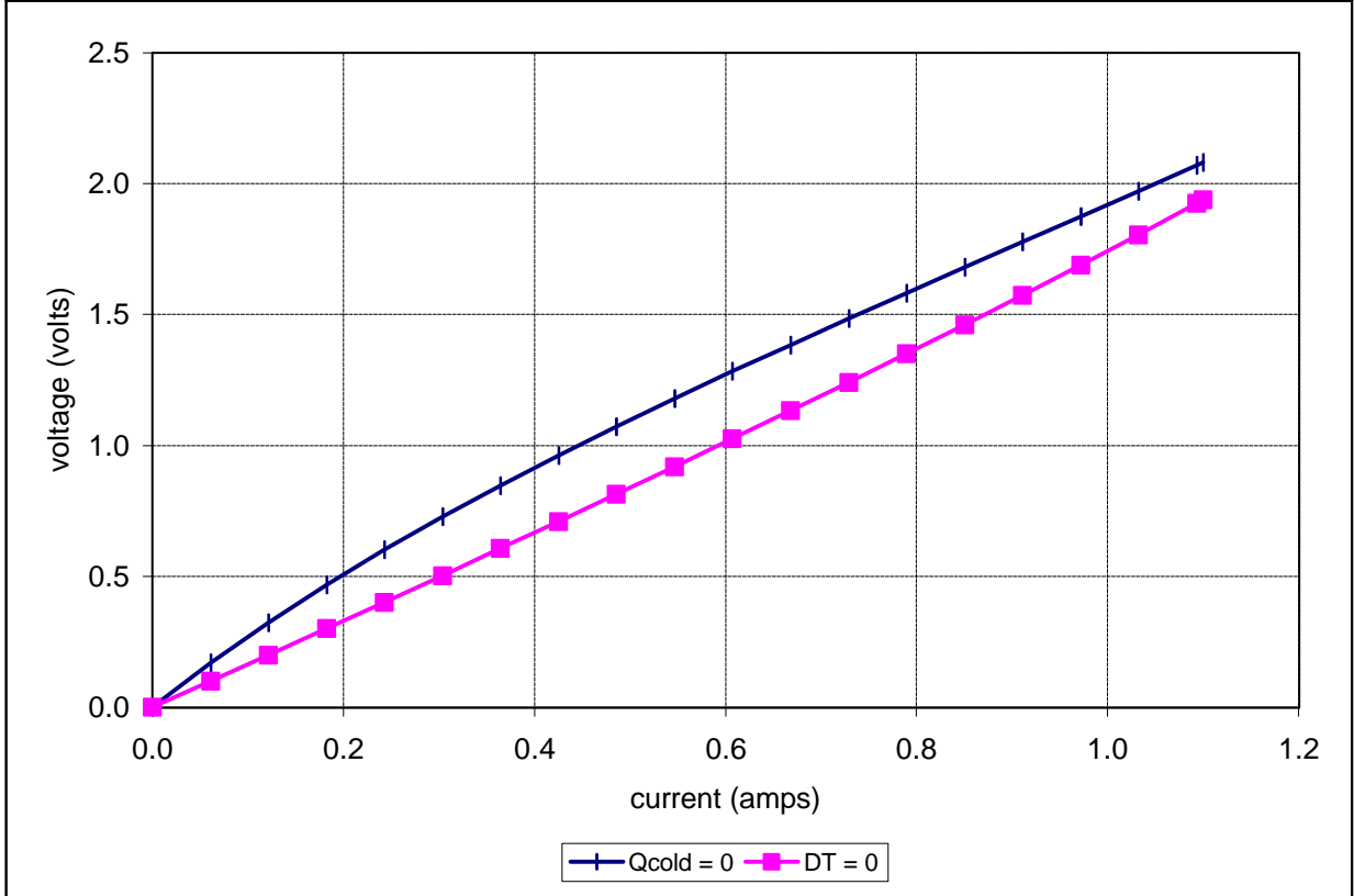
Unpotted TE-17-0.6-1.5 at a hot-side temperature of 25 °C
