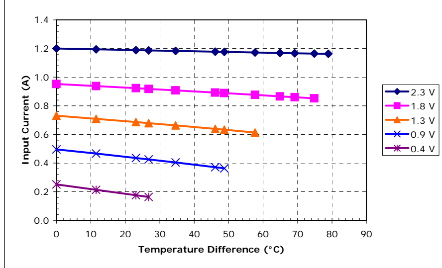
Unpotted TE-17-0.6-1.5 at a hot-side temperature of 50 °C
