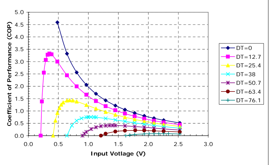
Unpotted TE-17-0.6-1.5 at a hot-side temperature of 70 °C
