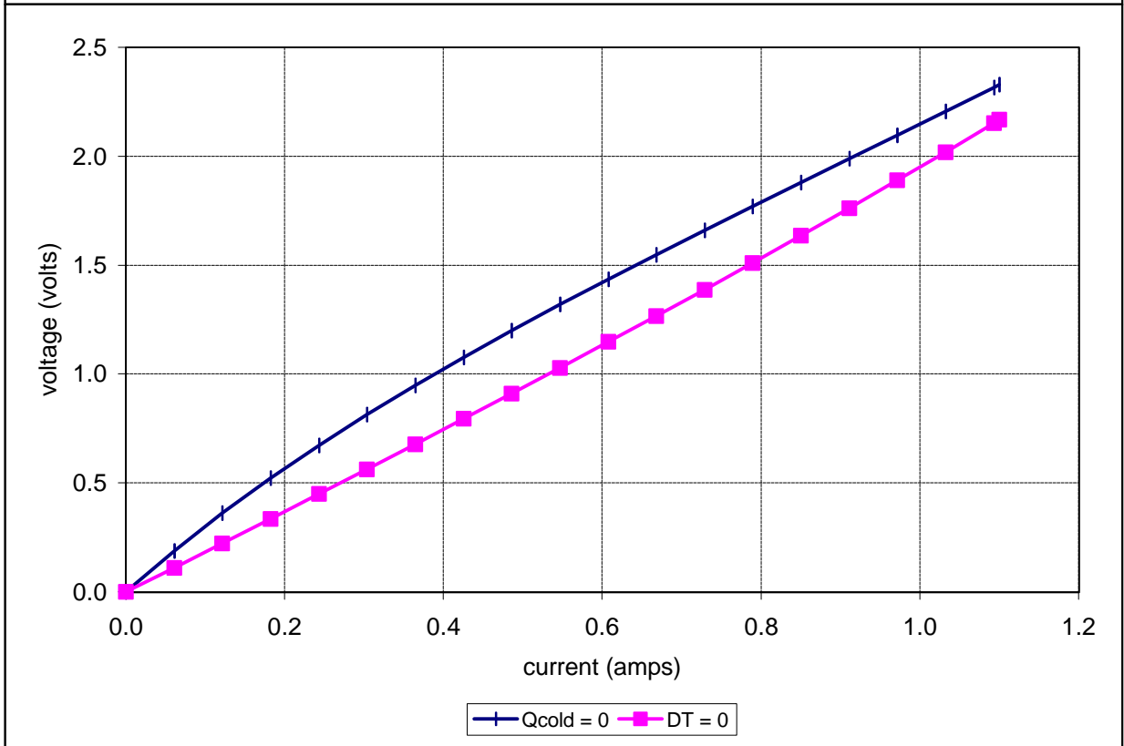
Potted TE-17-0.6-1.5 at a hot-side temperature of 50 °C
