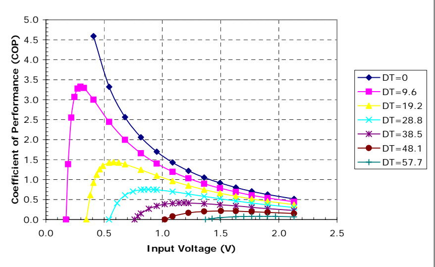
Potted TE-17-0.6-1.5 at a hot-side temperature of 30 °C
