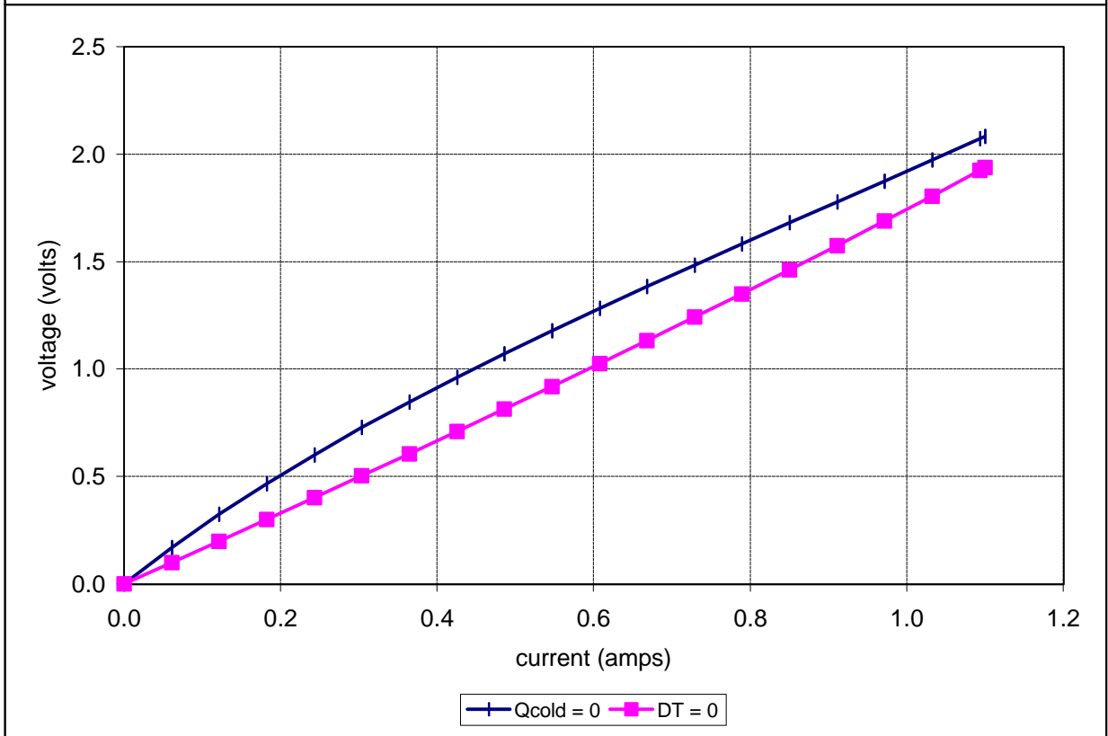
Potted TE-17-0.6-1.5 at a hot-side temperature of 25 °C
