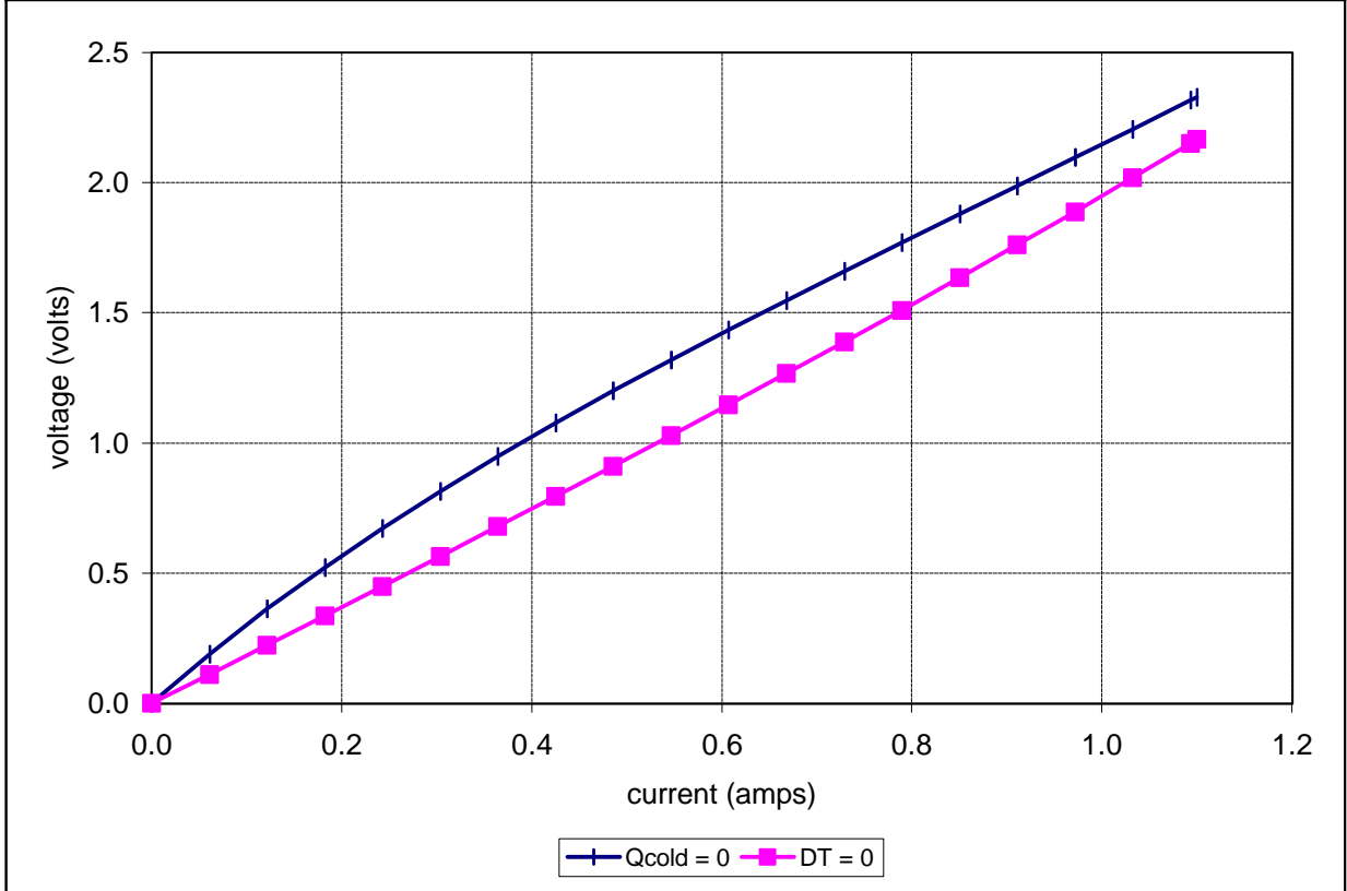
Unpotted TE-17-0.6-1.5 at a hot-side temperature of 50 °C
