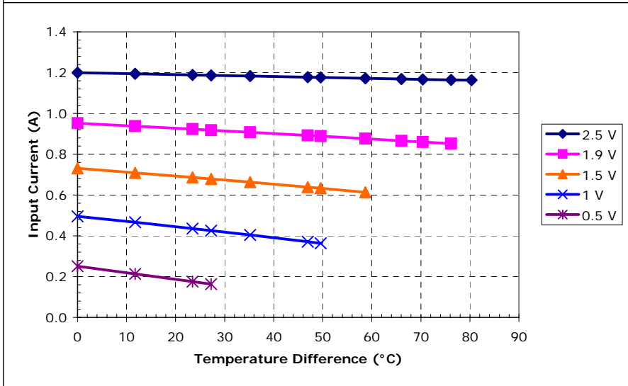
Potted TE-17-0.6-1.5 at a hot-side temperature of 70 °C
