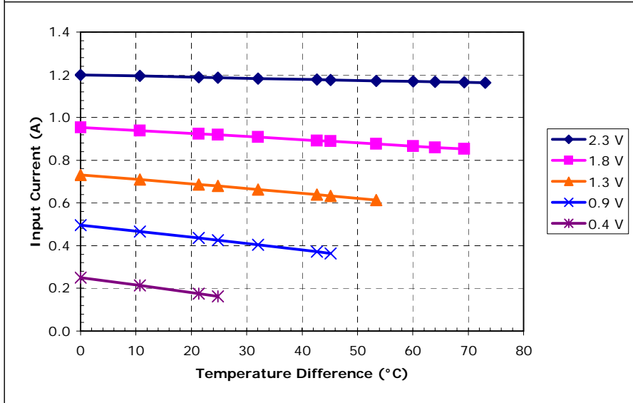
Potted TE-17-0.6-1.5 at a hot-side temperature of 50 °C
