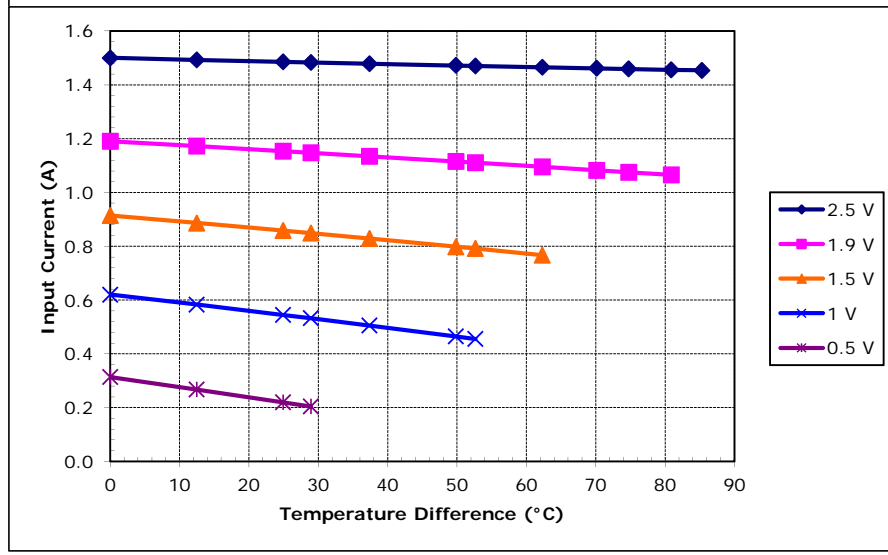
Unpotted TE-17-0.6-1.2 at a hot-side temperature of 70 °C
