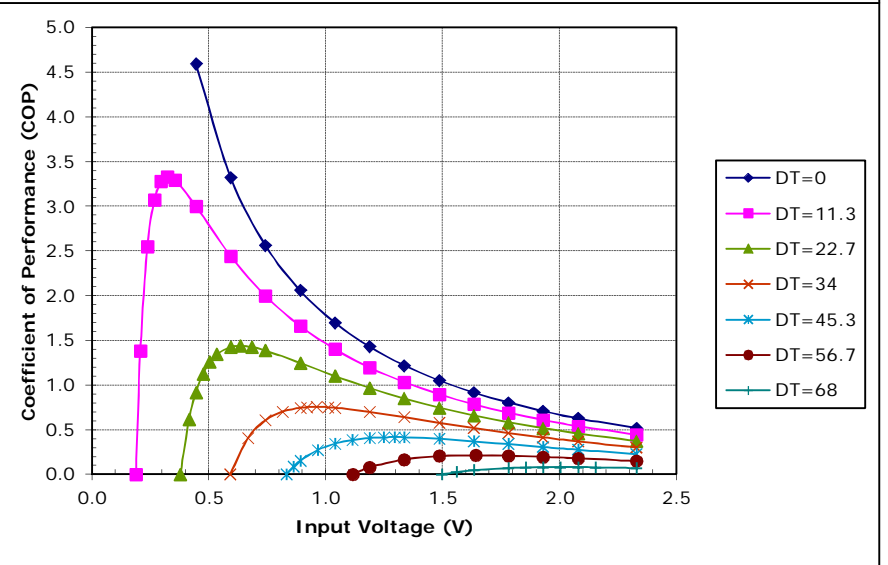
Unpotted TE-17-0.6-1.2 at a hot-side temperature of 50 °C
