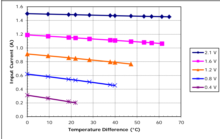
Potted TE-17-0.6-1.2 at a hot-side temperature of 30 °C
