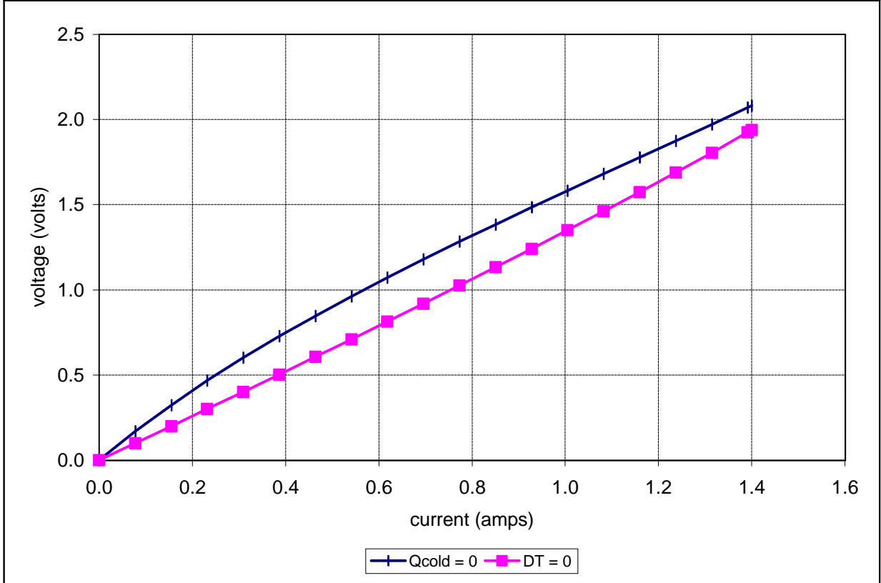
Unpotted TE-17-0.6-1.2 at a hot-side temperature of 25 °C
