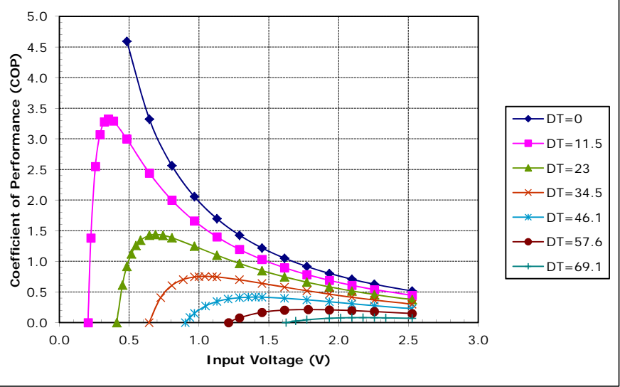
Potted TE-17-0.6-1.2 at a hot-side temperature of 70 °C
