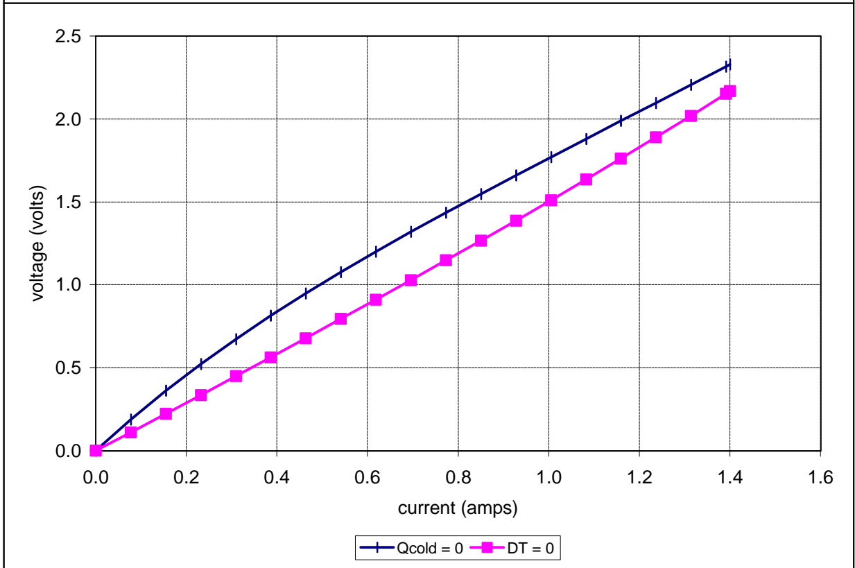
Potted TE-17-0.6-1.2 at a hot-side temperature of 50 °C
