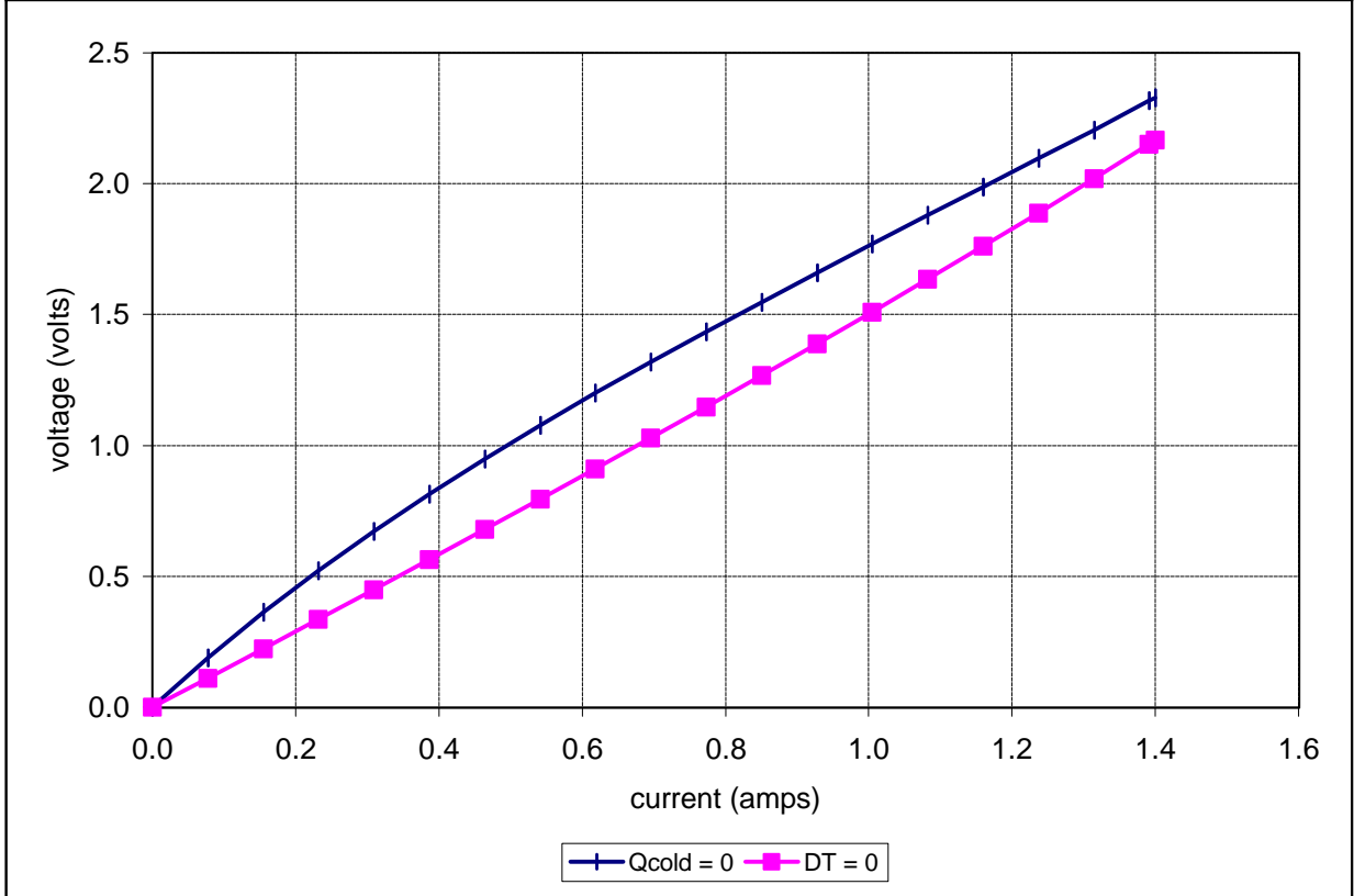
Unpotted TE-17-0.6-1.2 at a hot-side temperature of 50 °C
