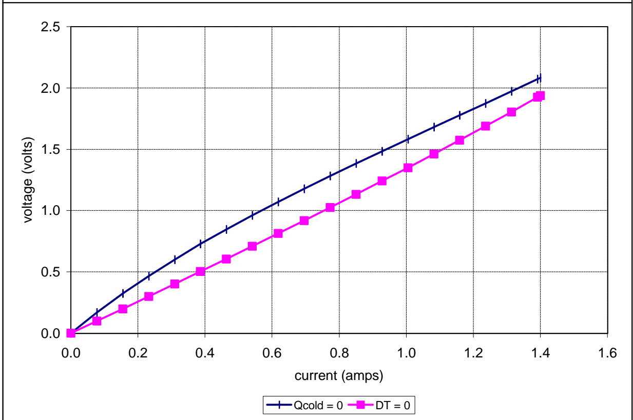
Potted TE-17-0.6-1.2 at a hot-side temperature of 25 °C
