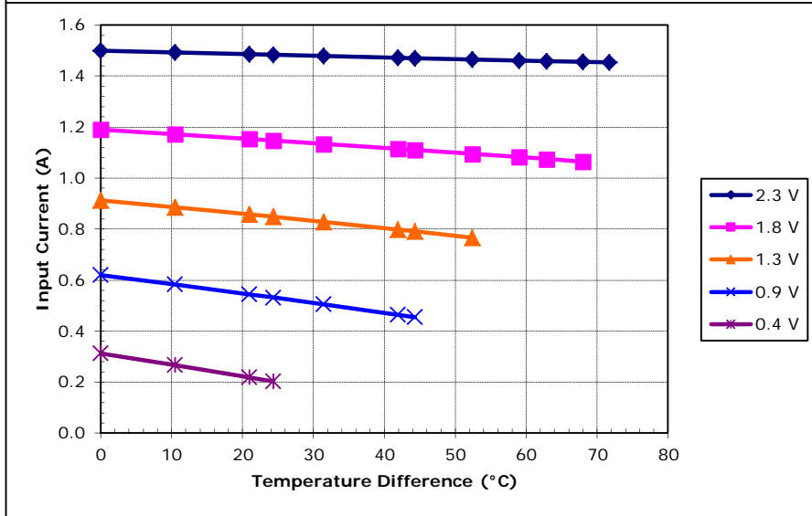
Potted TE-17-0.6-1.2 at a hot-side temperature of 50 °C
