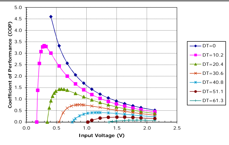
Unpotted TE-17-0.6-1.2 at a hot-side temperature of 30 °C
