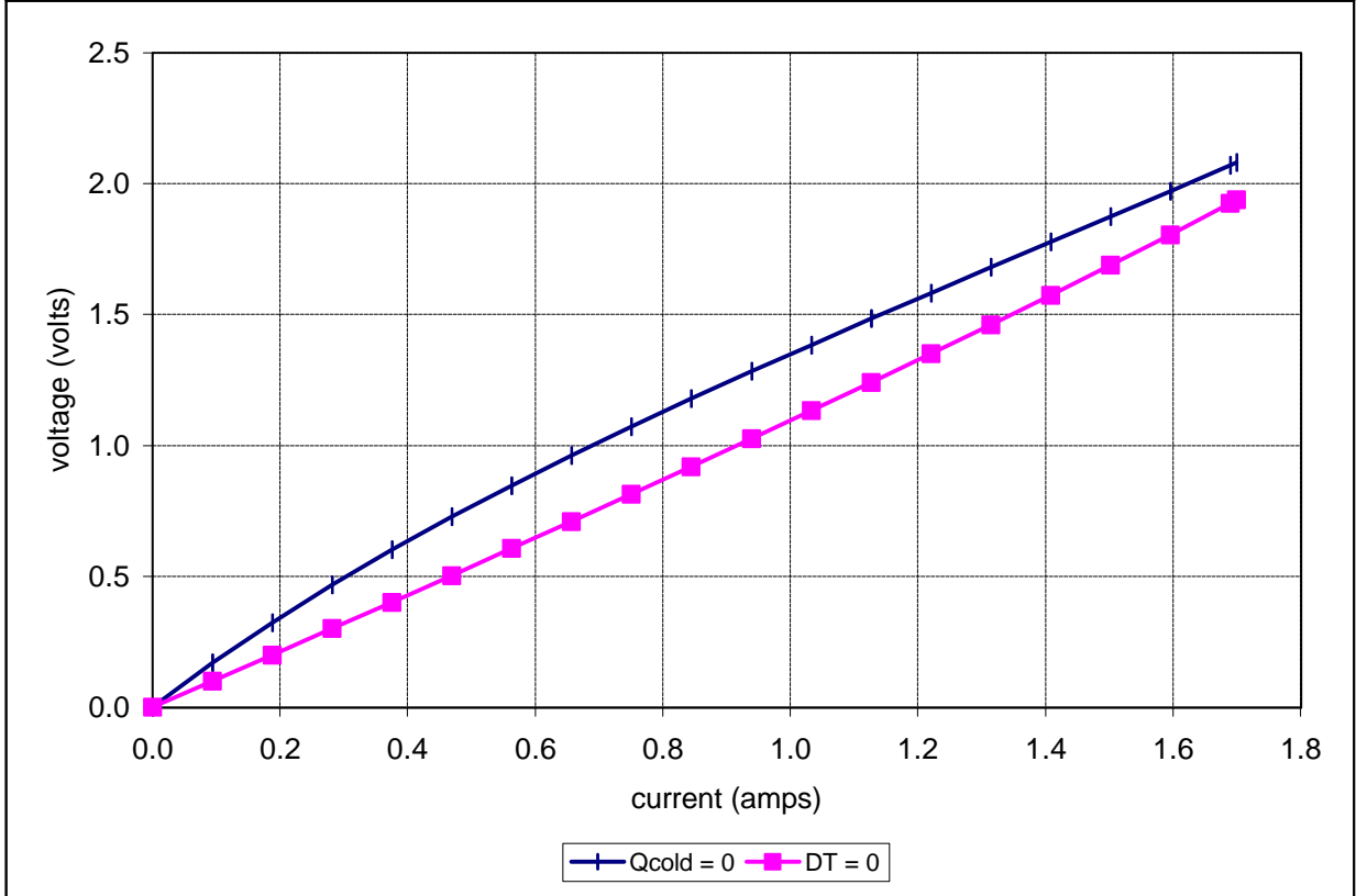
Unpotted TE-17-0.6-1.0 at a hot-side temperature of 25 °C
