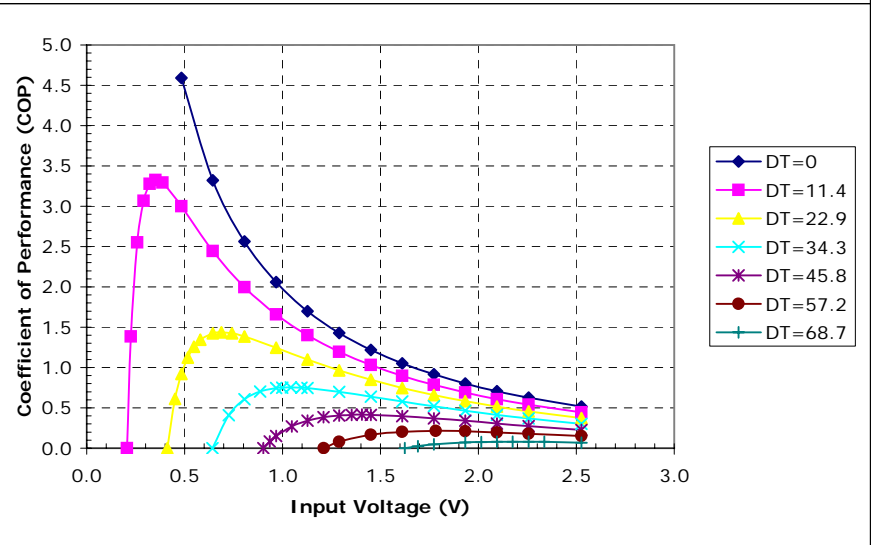
Potted TE-17-0.6-1.0 at a hot-side temperature of 70 °C
