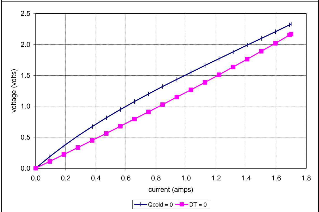
Potted TE-17-0.6-1.0 at a hot-side temperature of 50 °C
