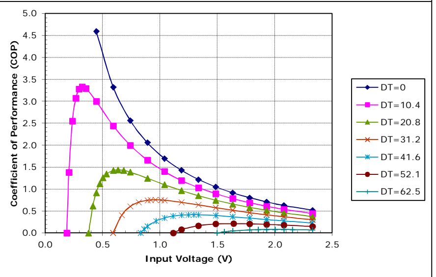
Potted TE-17-0.6-1.0 at a hot-side temperature of 50 °C
