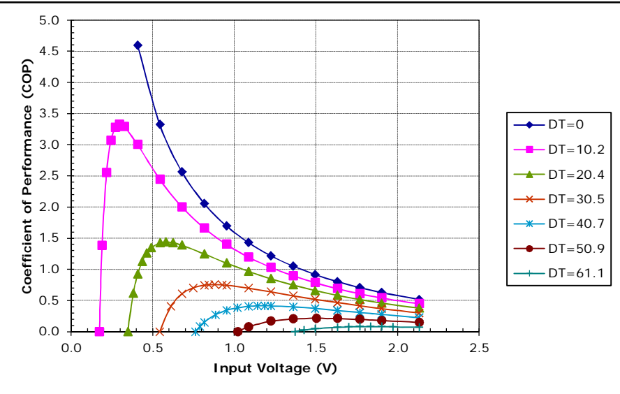
Unpotted TE-17-0.6-1.0 at a hot-side temperature of 30 °C
