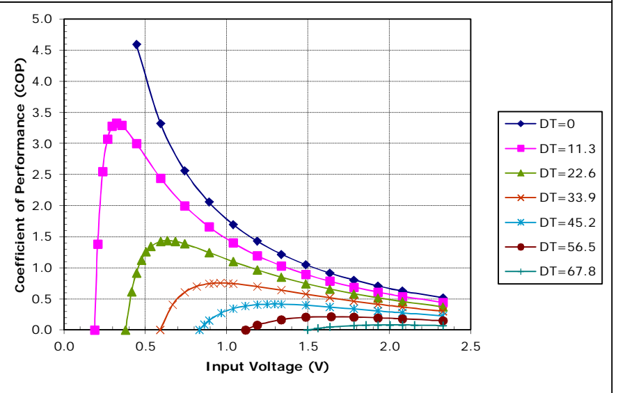
Unpotted TE-17-0.6-1.0 at a hot-side temperature of 50 °C
