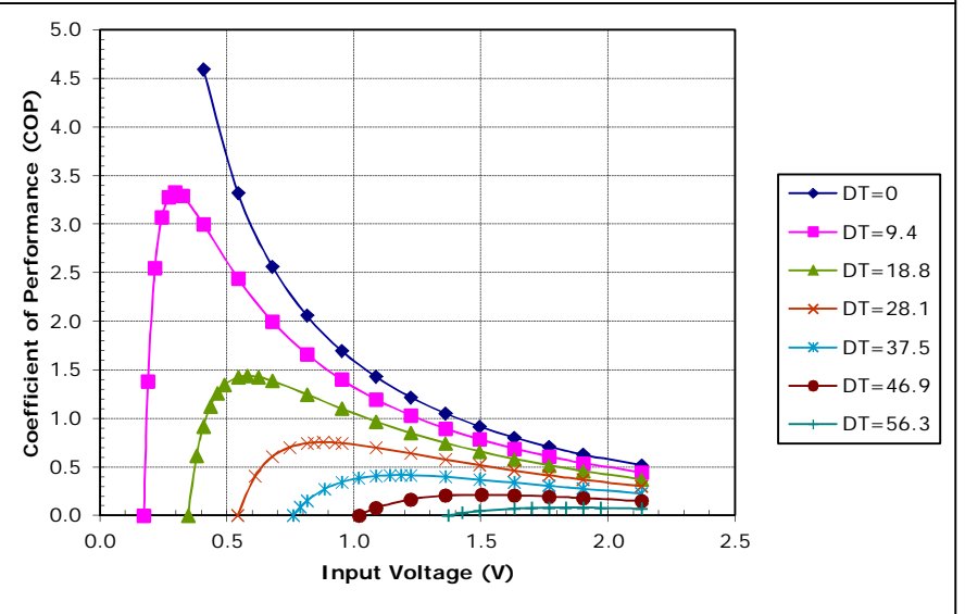
Potted TE-17-0.6-1.0 at a hot-side temperature of 30 °C
