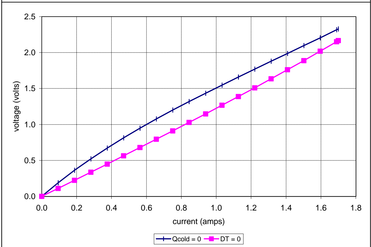
Unpotted TE-17-0.6-1.0 at a hot-side temperature of 50 °C
