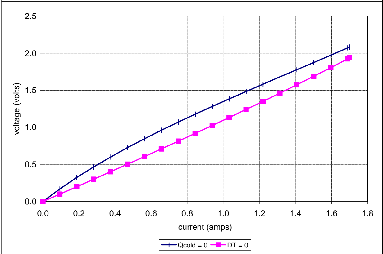
Potted TE-17-0.6-1.0 at a hot-side temperature of 25 °C
