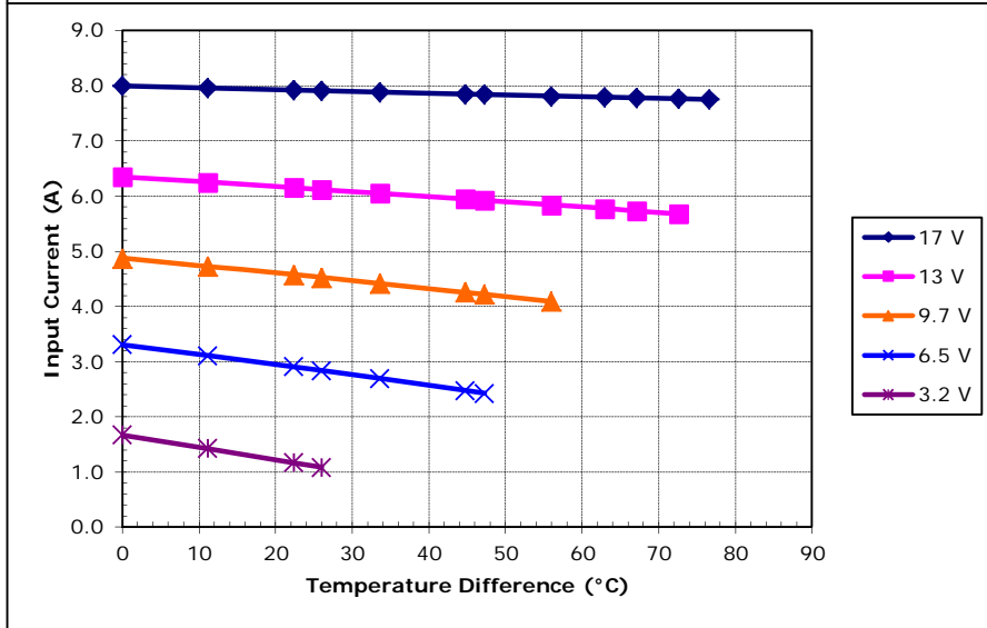
Potted TE-127-2.0-2.5 at a hot-side temperature of 50 °C
