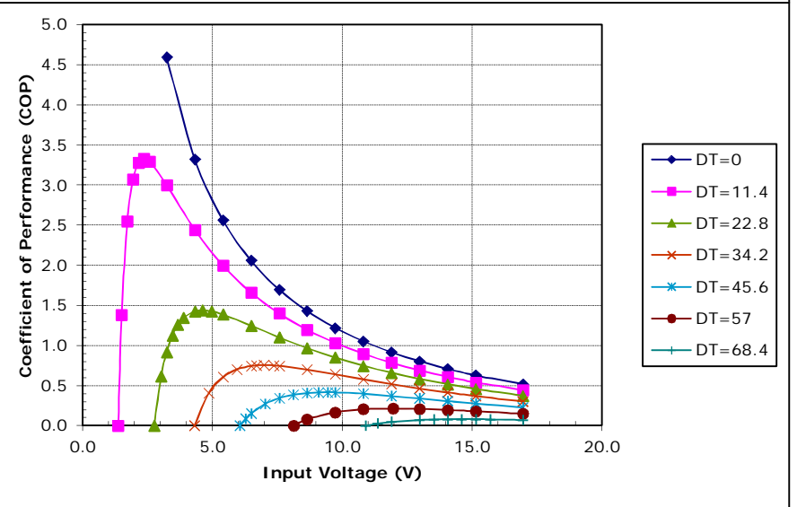
Unpotted TE-127-2.0-2.5 at a hot-side temperature of 50 °C
