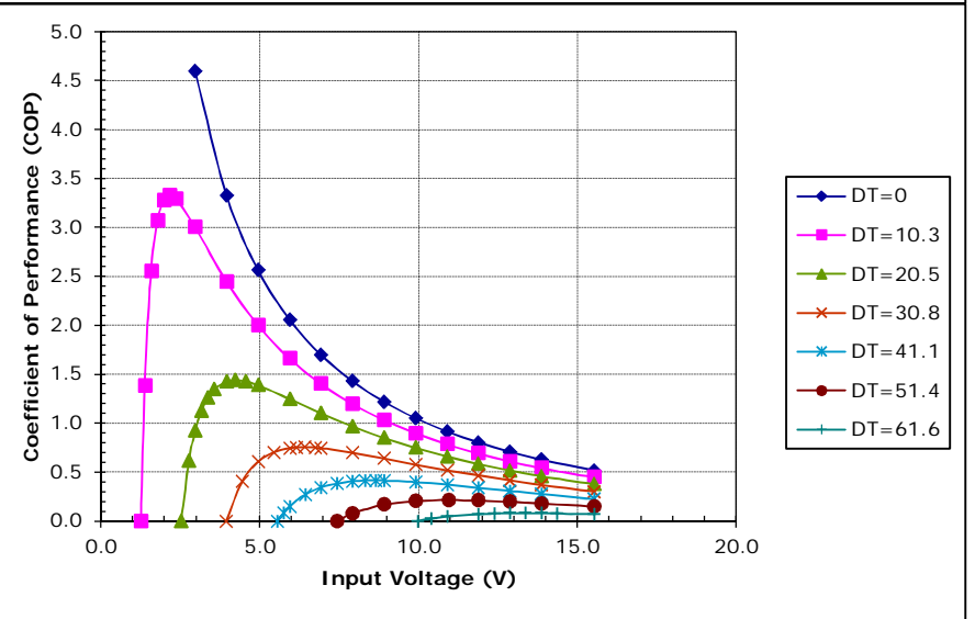
Unpotted TE-127-2.0-2.5 at a hot-side temperature of 30 °C
