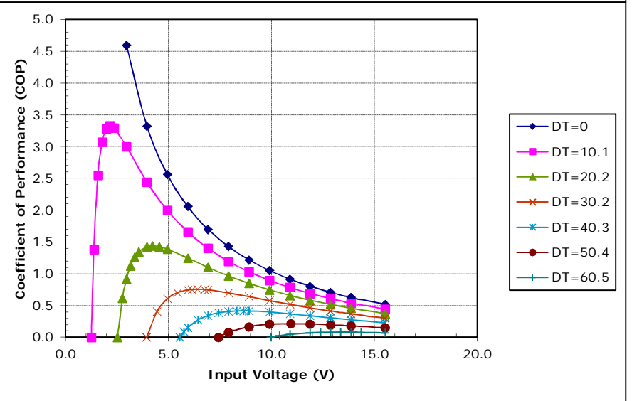
Potted TE-127-2.0-2.5 at a hot-side temperature of 30 °C
