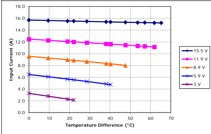
Potted TE-127-2.0-1.15 at a hot-side temperature of 30 °C
