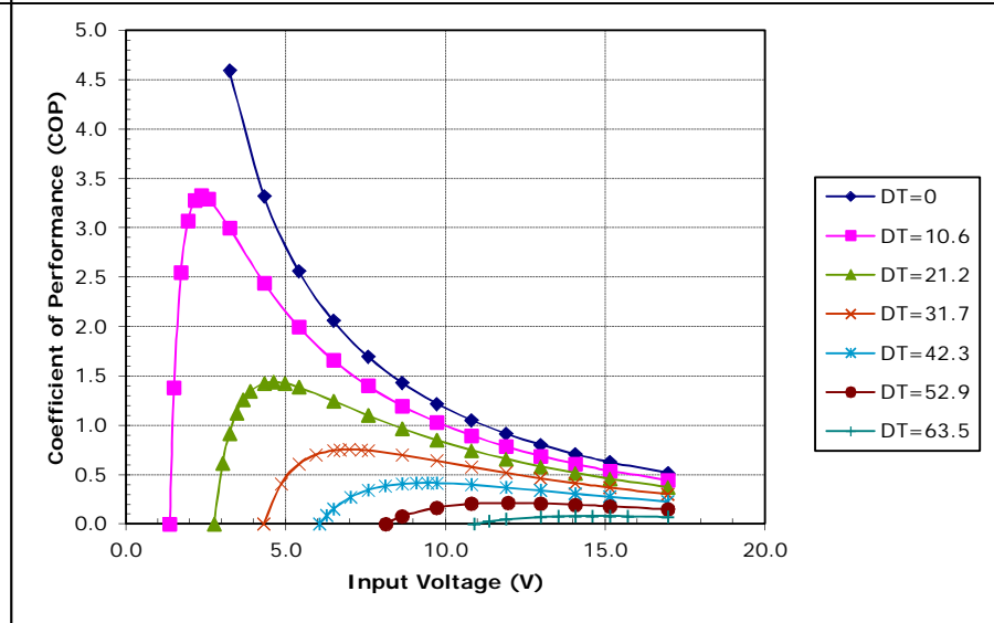
Potted TE-127-2.0-1.15 at a hot-side temperature of 50 °C
