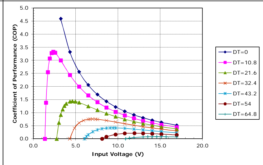
Unpotted TE-127-2.0-1.15 at a hot-side temperature of 50 °C
