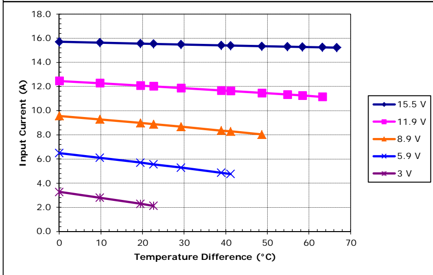
Unpotted TE-127-2.0-1.15 at a hot-side temperature of 30 °C
