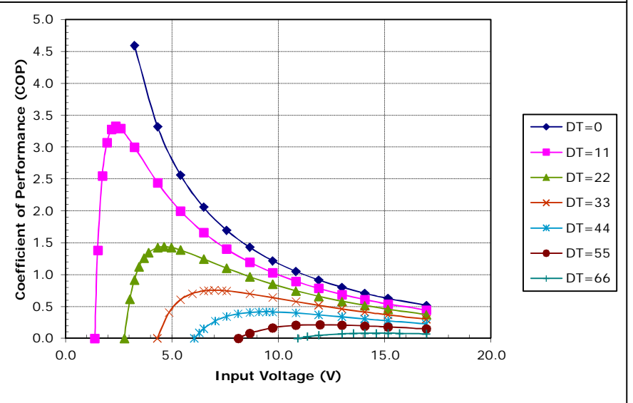
Potted TE-127-1.4-2.5 at a hot-side temperature of 50 °C
