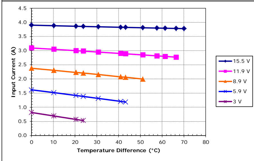
Unpotted TE-127-1.4-2.5 at a hot-side temperature of 30 °C
