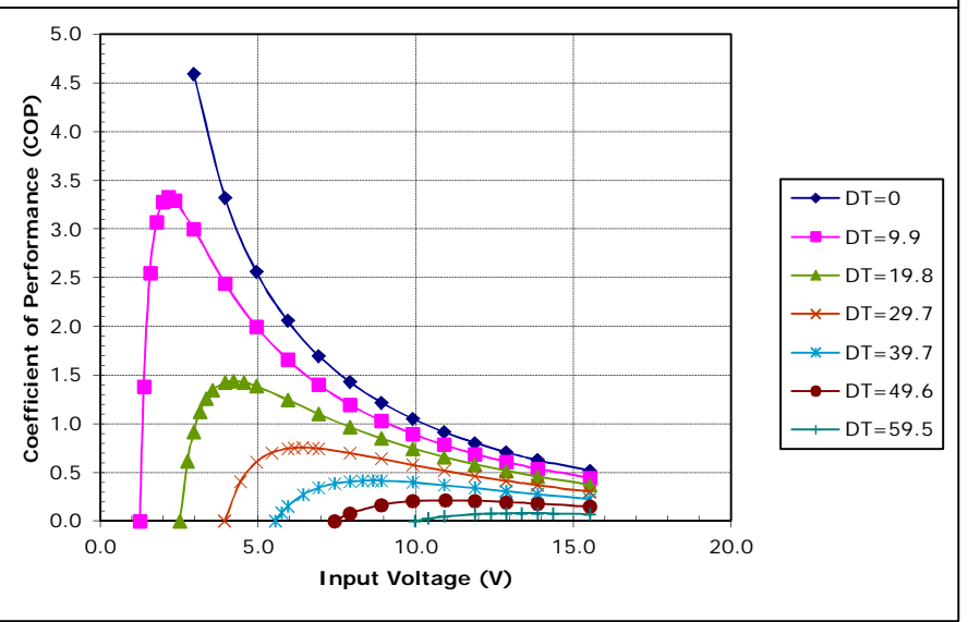
Potted TE-127-1.4-2.5 at a hot-side temperature of 30 °C
