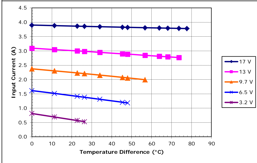
Unpotted TE-127-1.4-2.5 at a hot-side temperature of 50 °C
