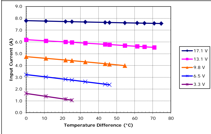
Unpotted TE-127-1.4-1.15 at a hot-side temperature of 50 °C
