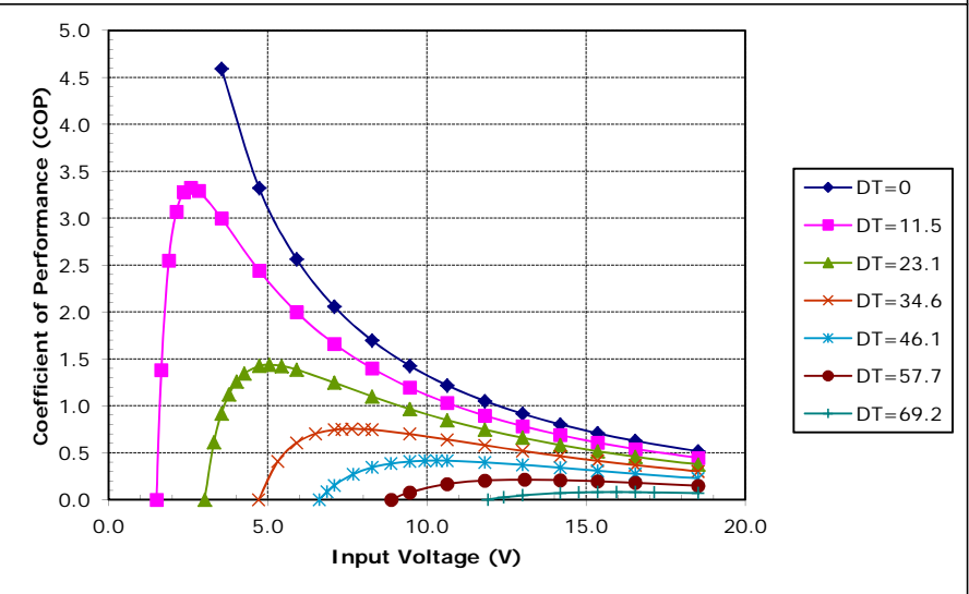
Potted TE-127-1.4-1.15 at a hot-side temperature of 70 °C
