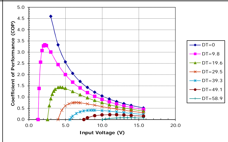
Unpotted TE-127-1.4-1.15 at a hot-side temperature of 30 °C
