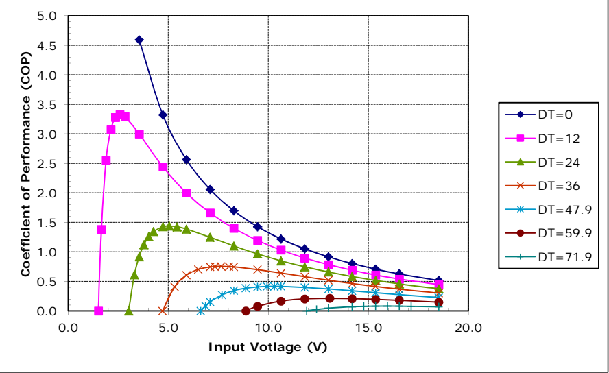
Unpotted TE-127-1.4-1.15 at a hot-side temperature of 70 °C
