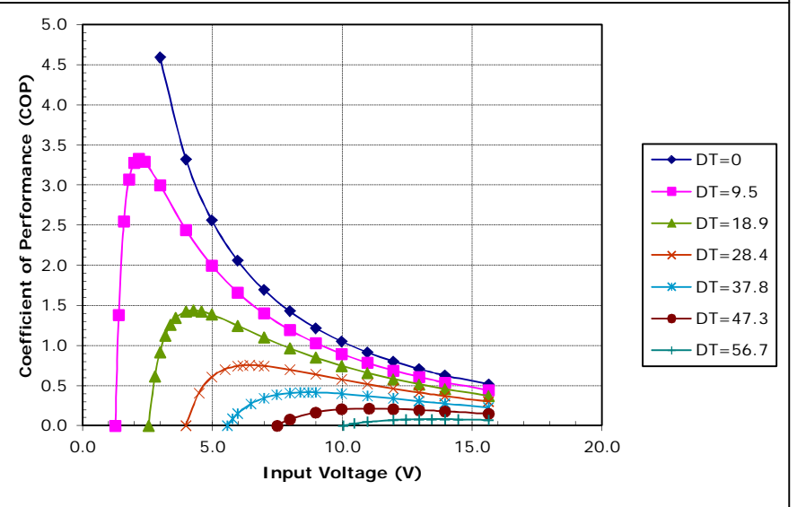
Potted TE-127-1.4-1.15 at a hot-side temperature of 30 °C
