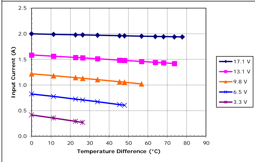
Unpotted TE-127-1.0-2.5 at a hot-side temperature of 50 °C
