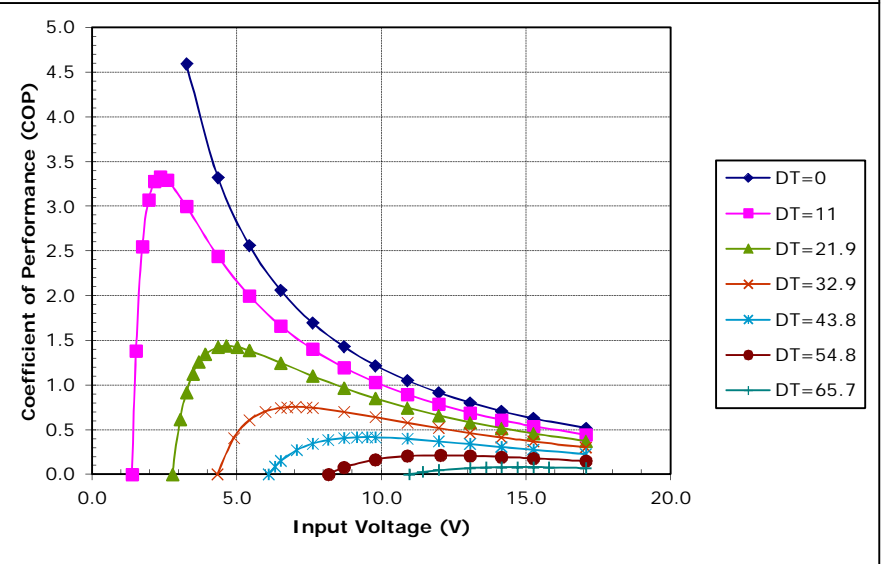
Potted TE-127-1.0-2.5 at a hot-side temperature of 50 °C
