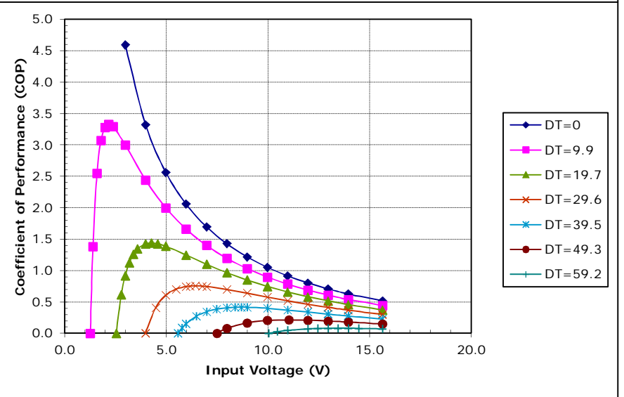
Potted TE-127-1.0-2.5 at a hot-side temperature of 30 °C
