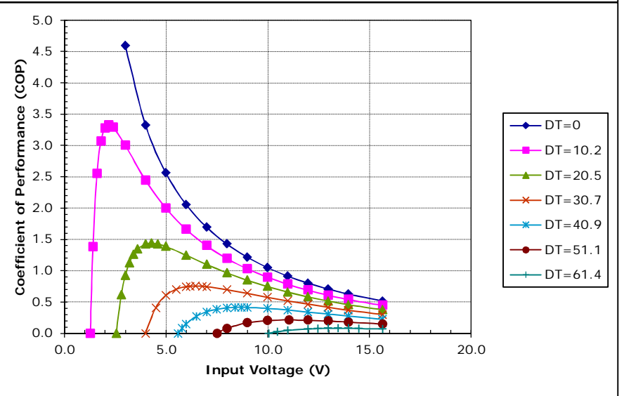
Unpotted TE-127-1.0-2.5 at a hot-side temperature of 30 °C
