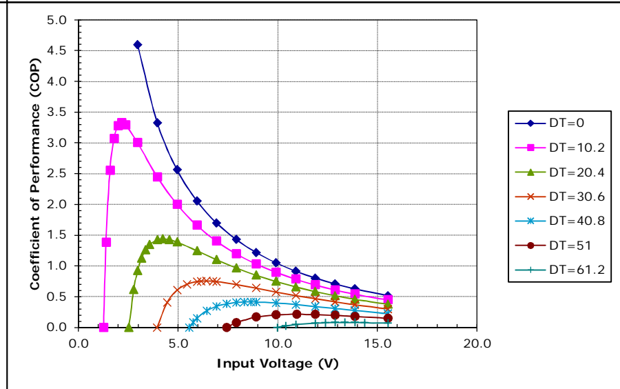
Unpotted TE-127-1.0-2.0 at a hot-side temperature of 30 °C
