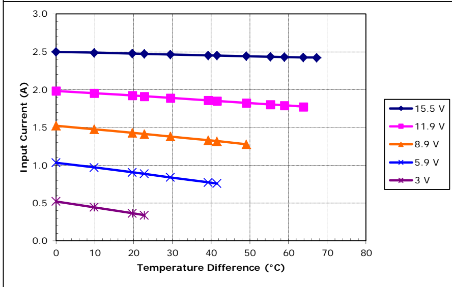
Potted TE-127-1.0-2.0 at a hot-side temperature of 30 °C
