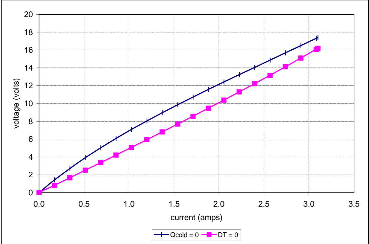
Unpotted TE-127-1.0-1.5 at a hot-side temperature of 50 °C
