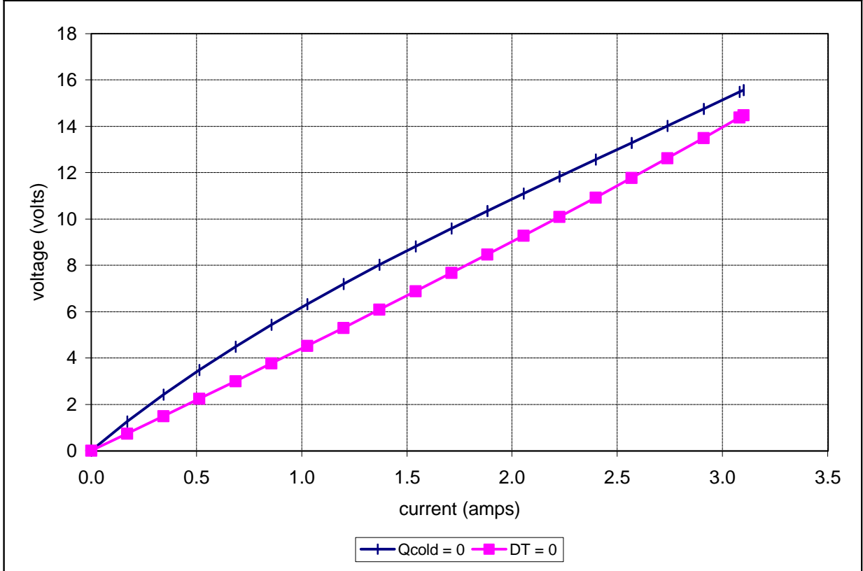
Unpotted TE-127-1.0-1.5 at a hot-side temperature of 25 °C
