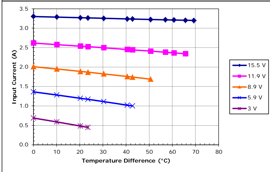
Unpotted TE-127-1.0-1.5 at a hot-side temperature of 30 °C
