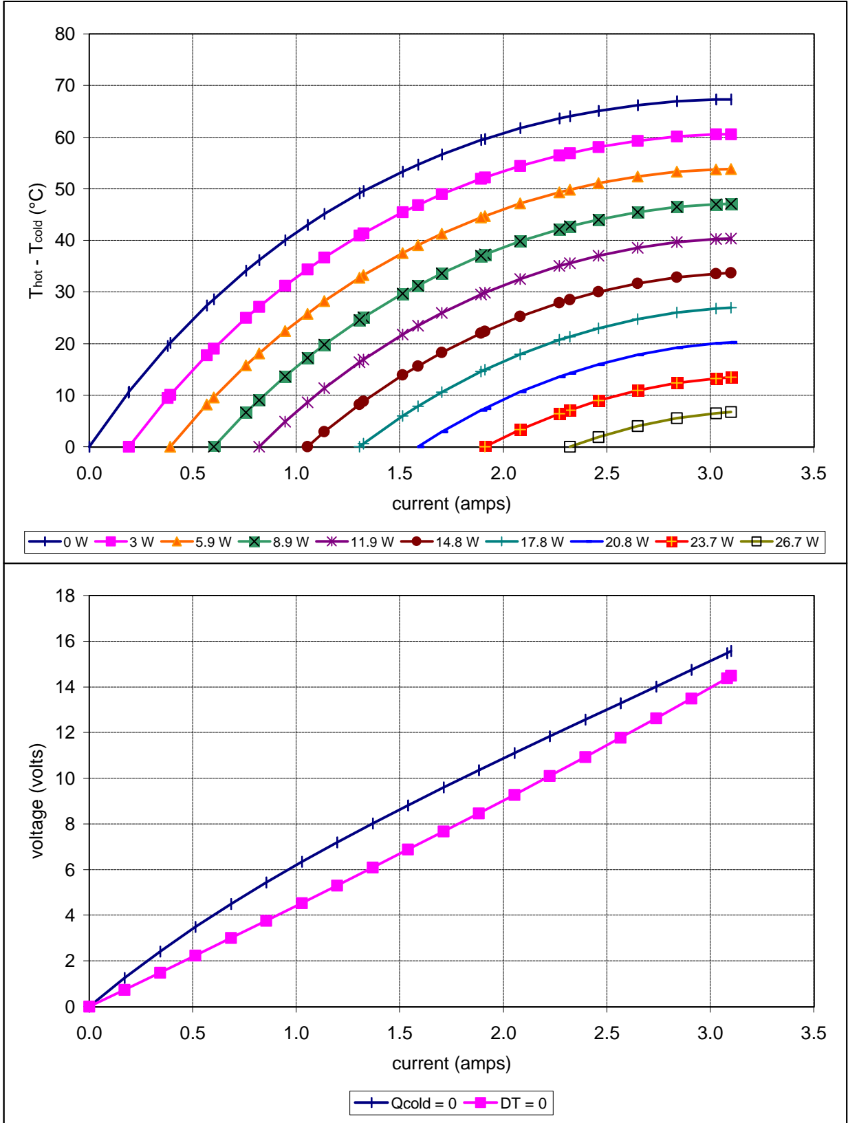
Potted TE-127-1.0-1.5 at a hot-side temperature of 25 °C
