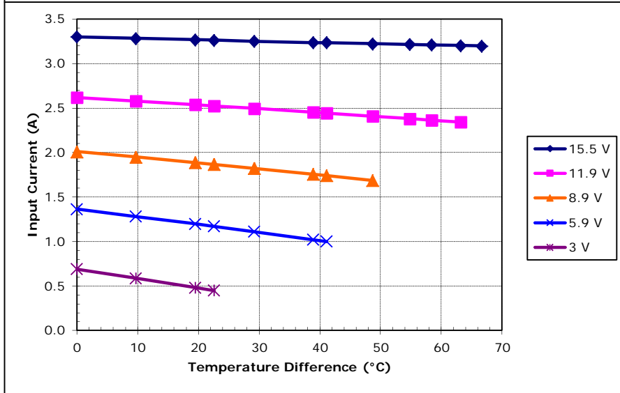
Potted TE-127-1.0-1.5 at a hot-side temperature of 30 °C
