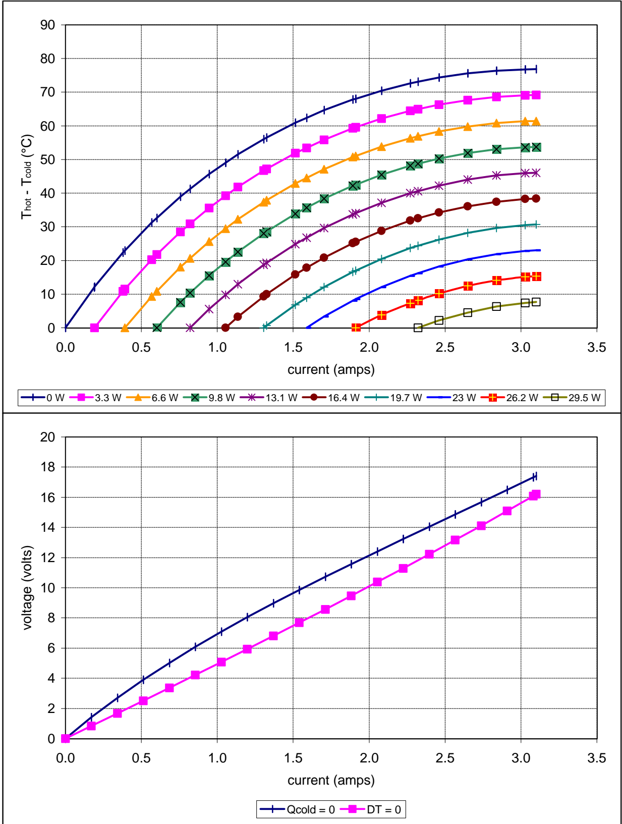
Potted TE-127-1.0-1.5 at a hot-side temperature of 50 °C
