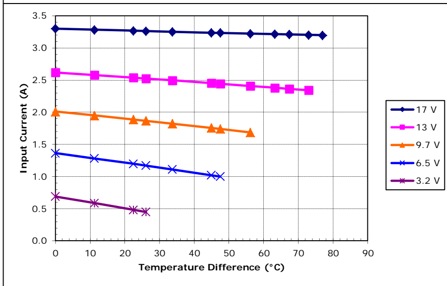
Unpotted TE-127-1.0-1.5 at a hot-side temperature of 50 °C
