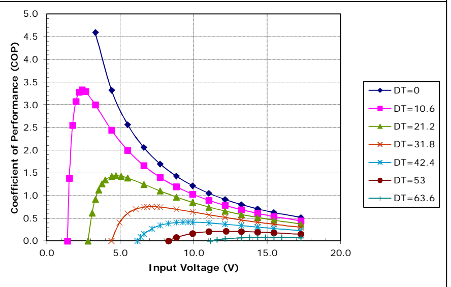
Potted TE-127-1.0-1.3 at a hot-side temperature of 50 °C
