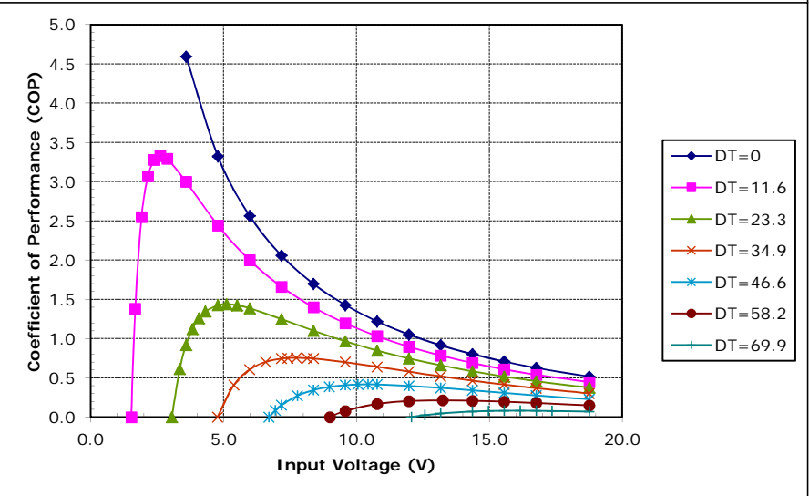
Potted TE-127-1.0-1.3 at a hot-side temperature of 70 °C
