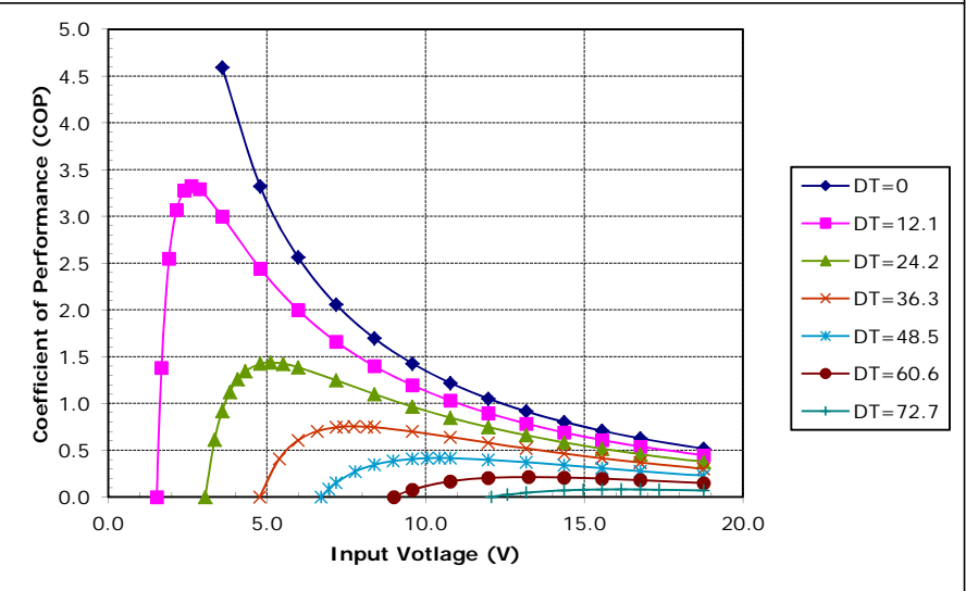
Unpotted TE-127-1.0-1.3 at a hot-side temperature of 70 °C
