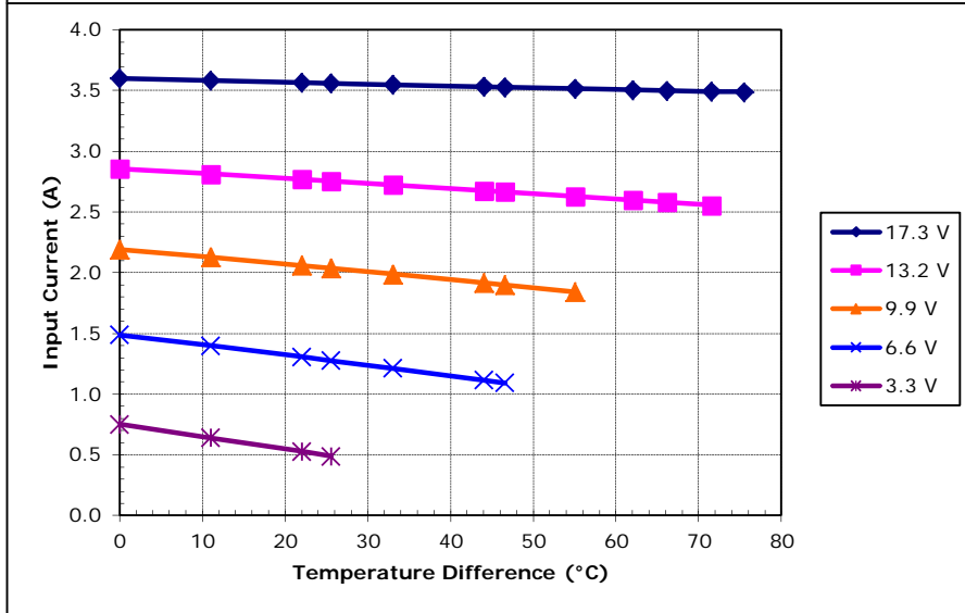
Unpotted TE-127-1.0-1.3 at a hot-side temperature of 50 °C
