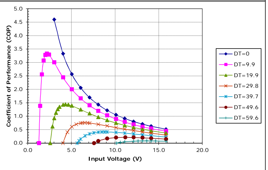
Unpotted TE-127-1.0-1.3 at a hot-side temperature of 30 °C
