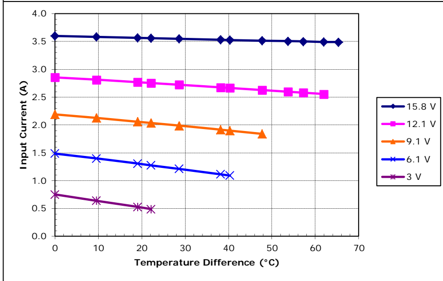
Potted TE-127-1.0-1.3 at a hot-side temperature of 30 °C
