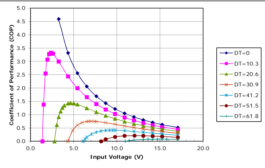
Potted TE-127-1.0-0.8 at a hot-side temperature of 50 °C
