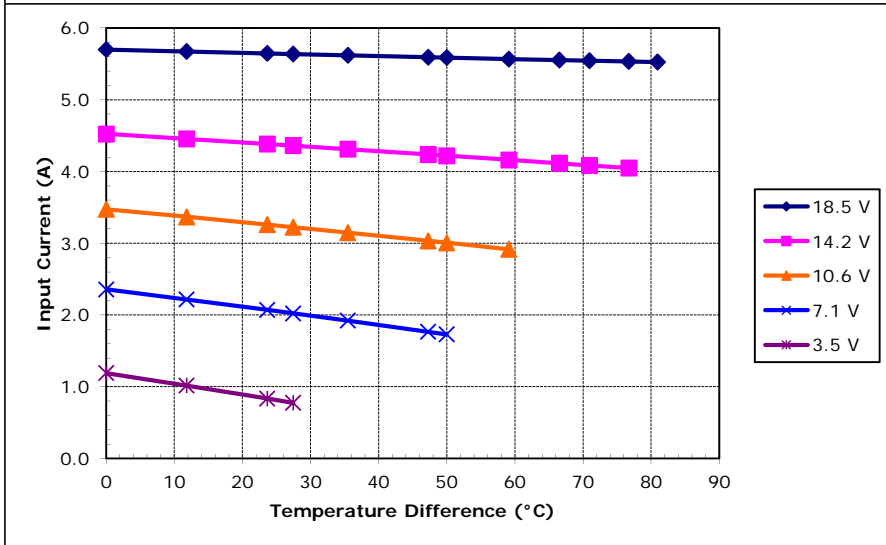
Unpotted TE-127-1.0-0.8 at a hot-side temperature of 70 °C
