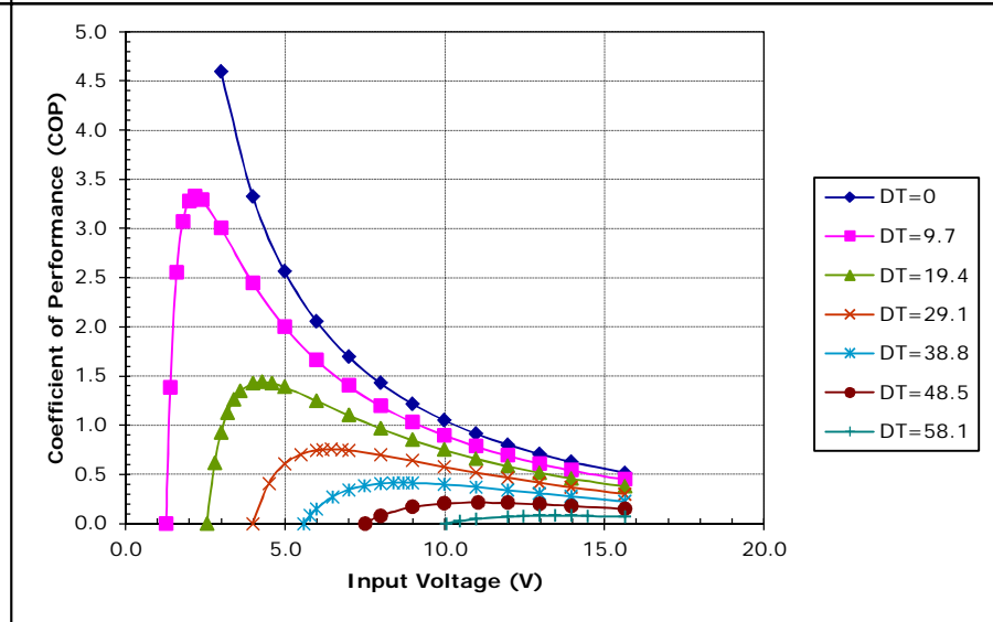
Unpotted TE-127-1.0-0.8 at a hot-side temperature of 30 °C
