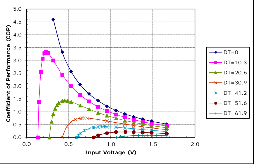
Potted TE-12-0.45-1.3 at a hot-side temperature of 50 °C
