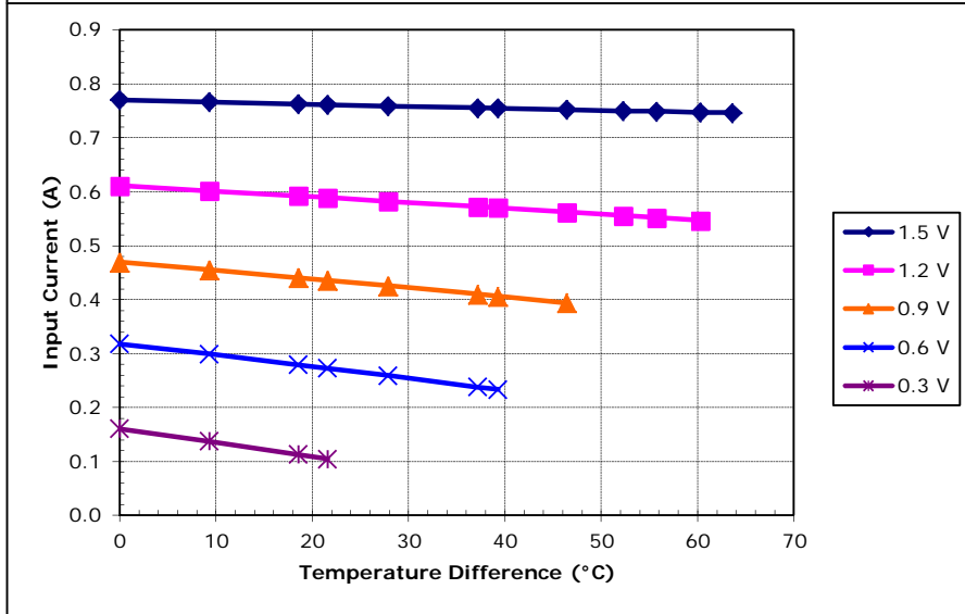
Potted TE-12-0.45-1.3 at a hot-side temperature of 30 °C
