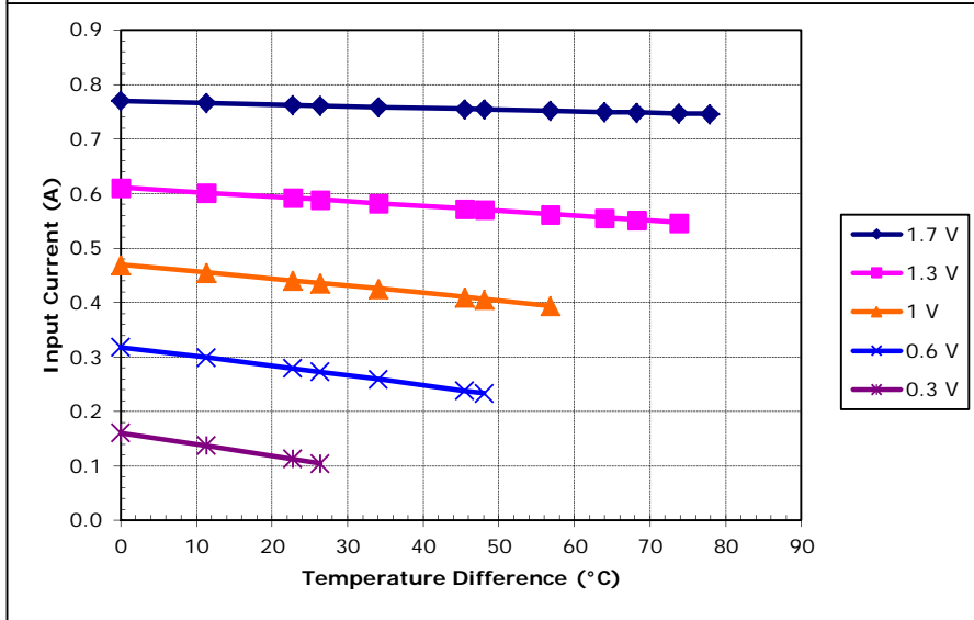
Unpotted TE-12-0.45-1.3 at a hot-side temperature of 50 °C
