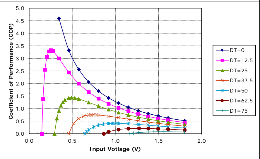
Unpotted TE-12-0.45-1.3 at a hot-side temperature of 70 °C
