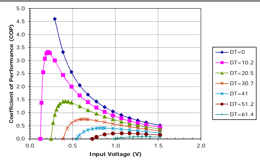
Unpotted TE-12-0.45-1.3 at a hot-side temperature of 30 °C
