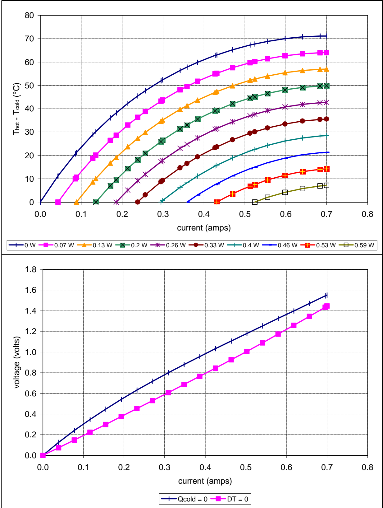
Potted TE-12-0.45-1.3 at a hot-side temperature of 50 °C
