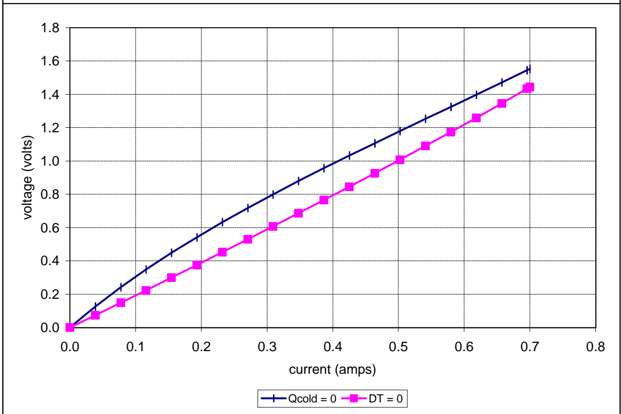
Unpotted TE-12-0.45-1.3 at a hot-side temperature of 50 °C
