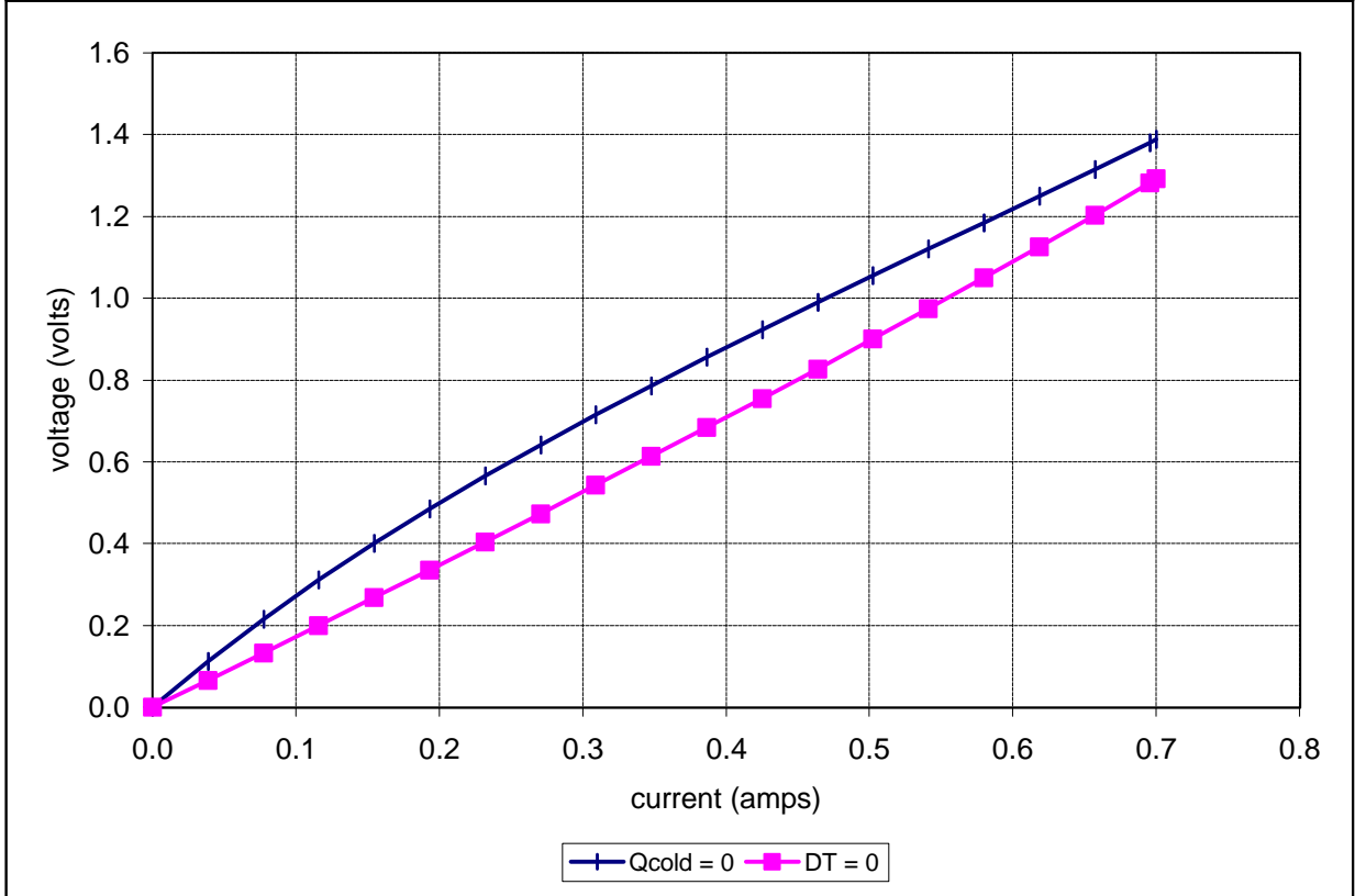
Unpotted TE-12-0.45-1.3 at a hot-side temperature of 25 °C
