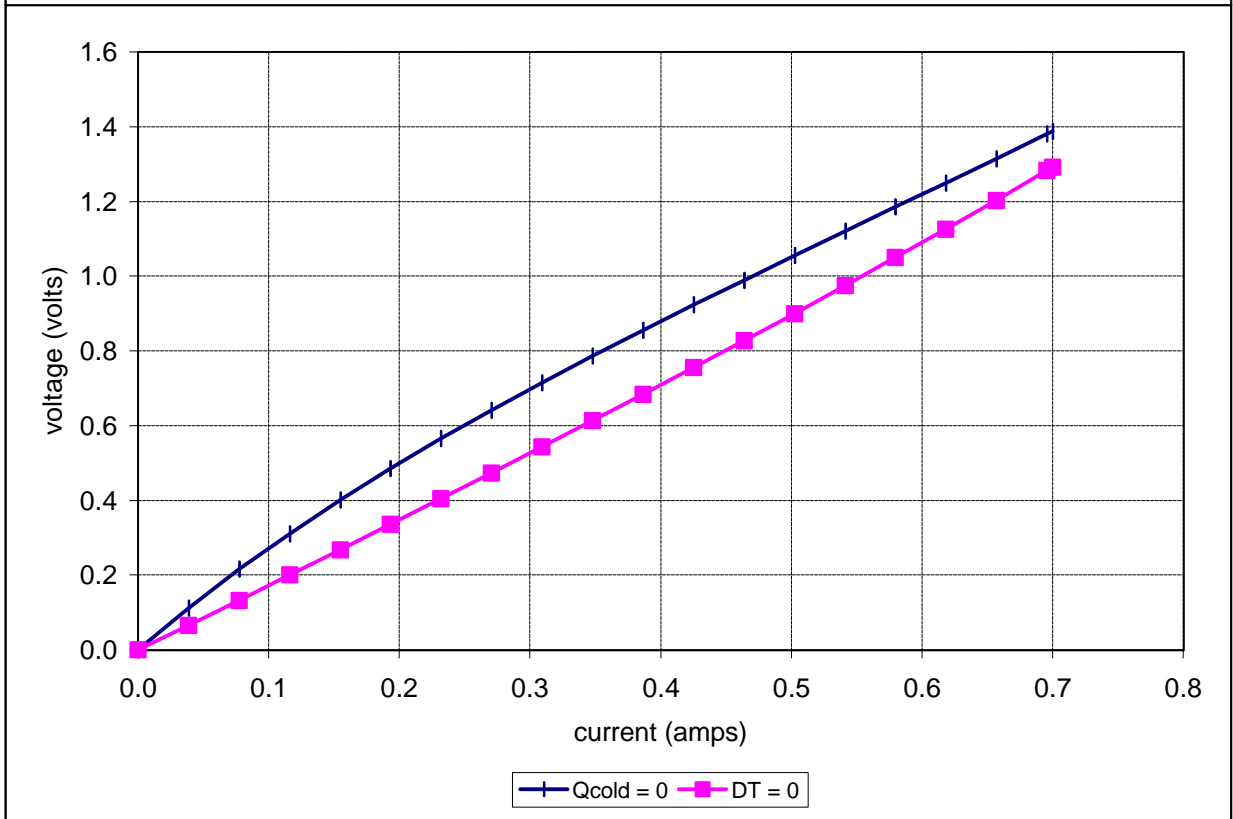
Potted TE-12-0.45-1.3 at a hot-side temperature of 25 °C
