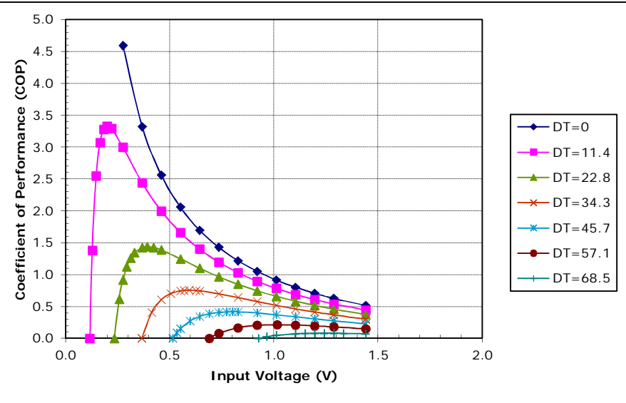
Unpotted TE-11-0.6-1.5 at a hot-side temperature of 50 °C
