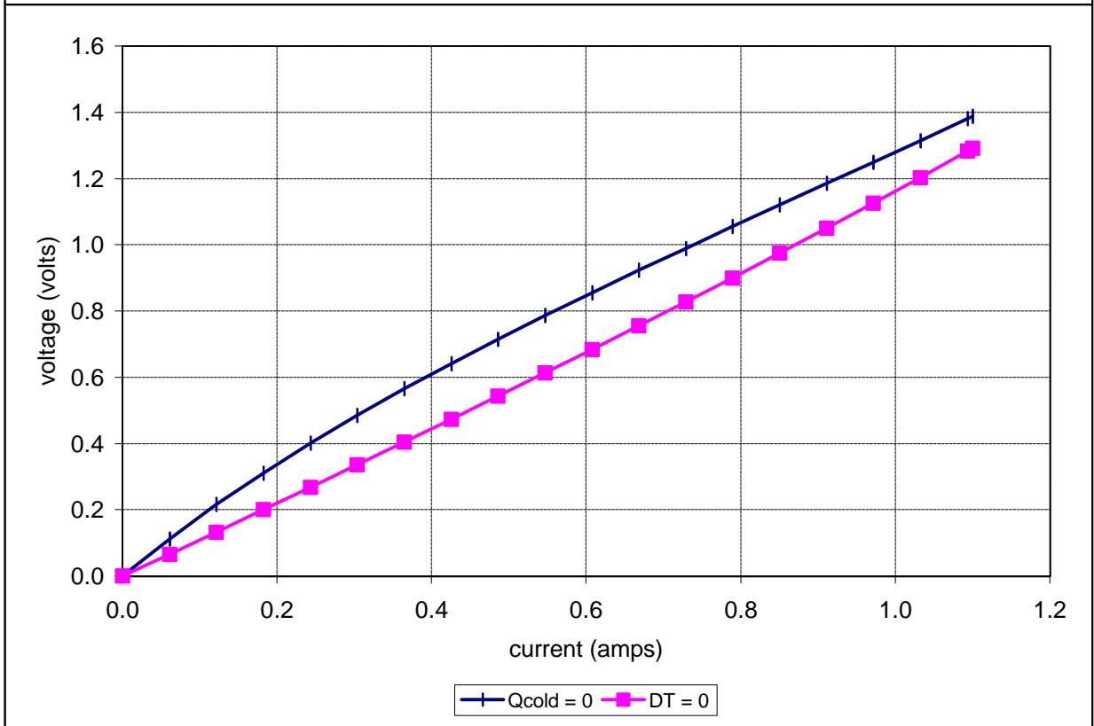
Potted TE-11-0.6-1.5 at a hot-side temperature of 25 °C
