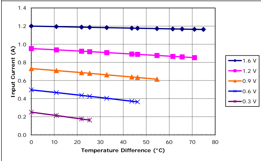
Potted TE-11-0.6-1.5 at a hot-side temperature of 70 °C
