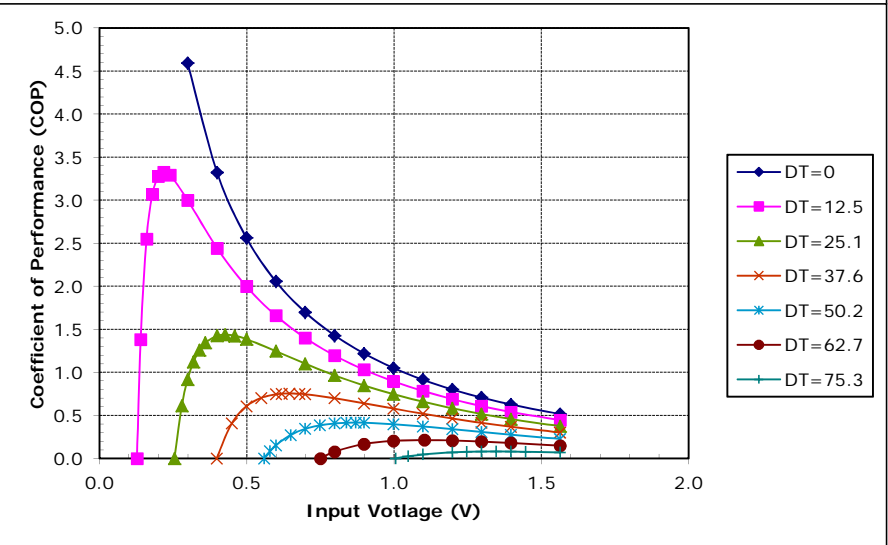
Unpotted TE-11-0.6-1.5 at a hot-side temperature of 70 °C
