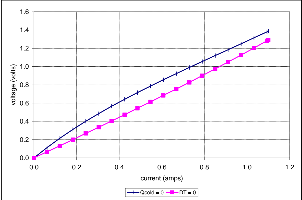
Unpotted TE-11-0.6-1.5 at a hot-side temperature of 25 °C
