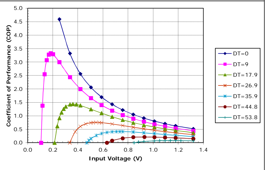
Potted TE-11-0.6-1.5 at a hot-side temperature of 30 °C
