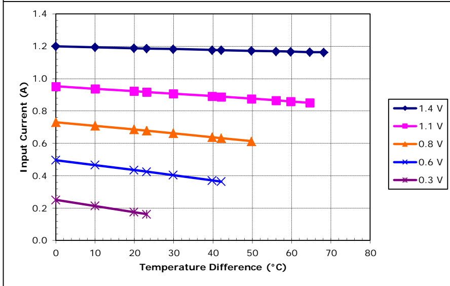
Potted TE-11-0.6-1.5 at a hot-side temperature of 50 °C
