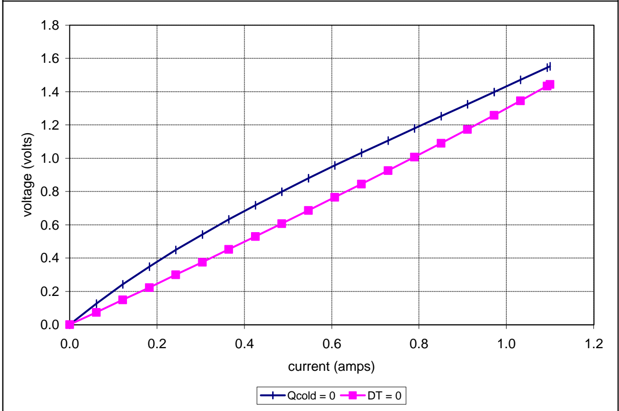
Unpotted TE-11-0.6-1.5 at a hot-side temperature of 50 °C
