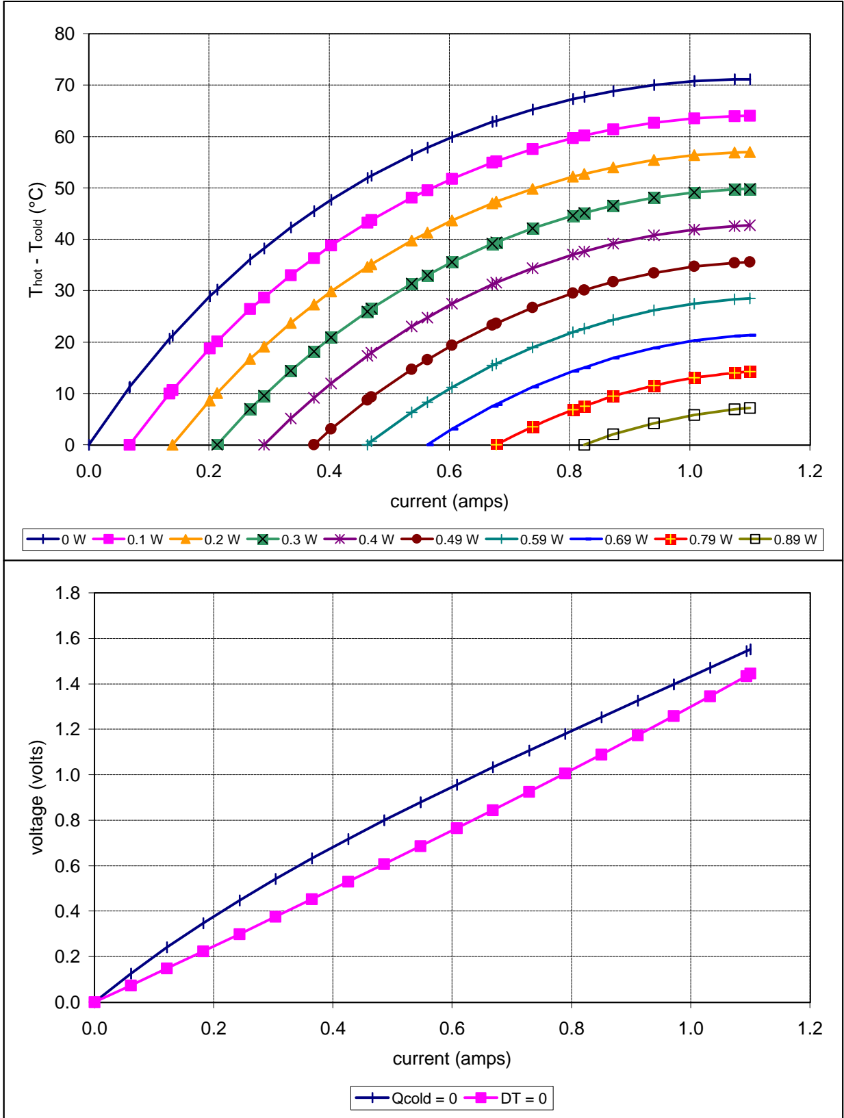
Potted TE-11-0.6-1.5 at a hot-side temperature of 50 °C
