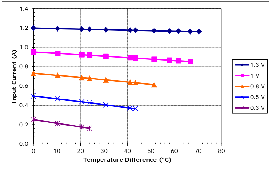
Unpotted TE-11-0.6-1.5 at a hot-side temperature of 30 °C
