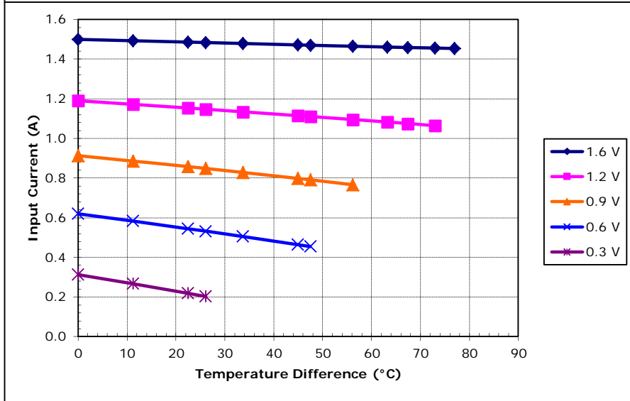
Unpotted TE-11-0.6-1.2 at a hot-side temperature of 50 °C
