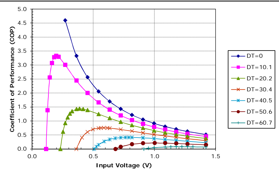
Unpotted TE-11-0.6-1.2 at a hot-side temperature of 30 °C
