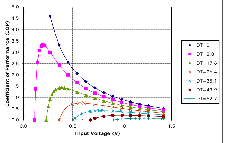
Potted TE-11-0.6-1.2 at a hot-side temperature of 30 °C
