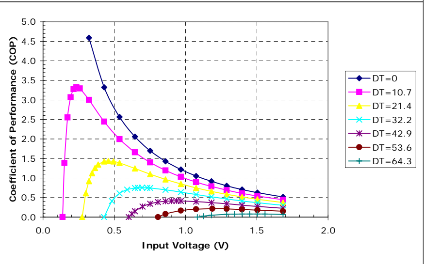
Potted TE-11-0.6-1.2 at a hot-side temperature of 70 °C
