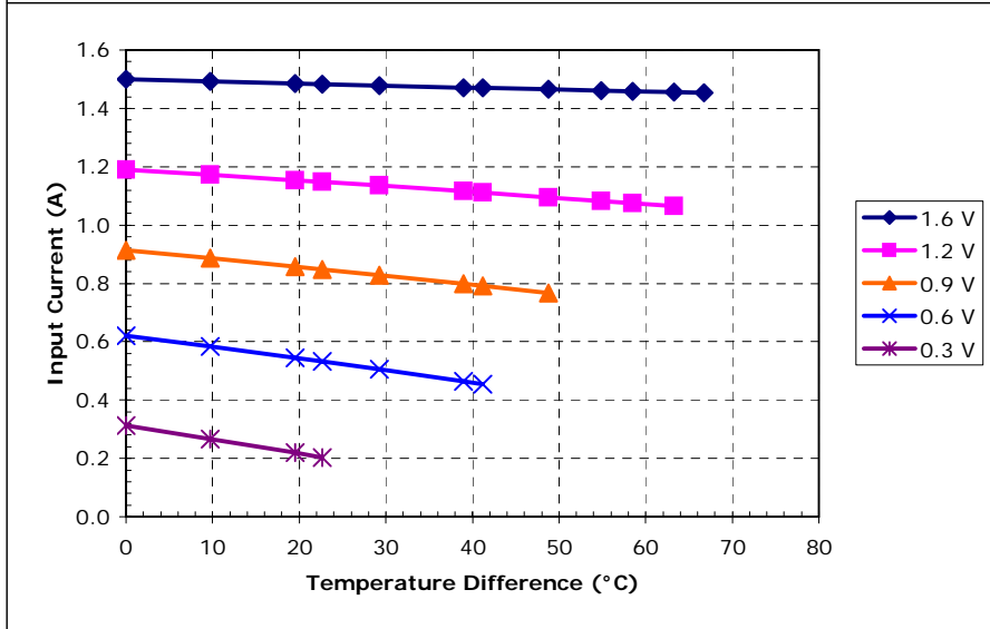
Potted TE-11-0.6-1.2 at a hot-side temperature of 50 °C
