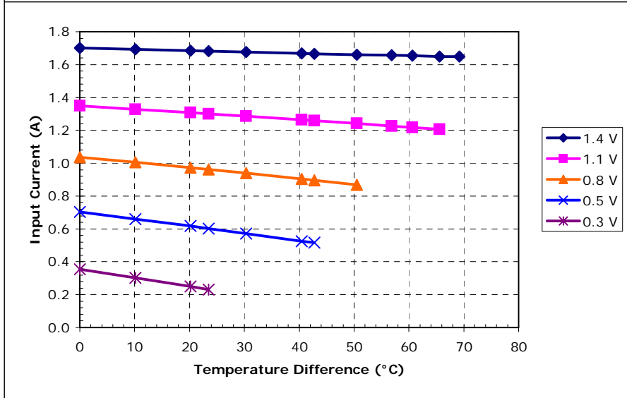
Unpotted TE-11-0.6-1.0 at a hot-side temperature of 30 °C
