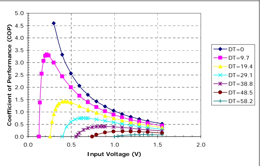
Potted TE-11-0.6-1.0 at a hot-side temperature of 50 °C
