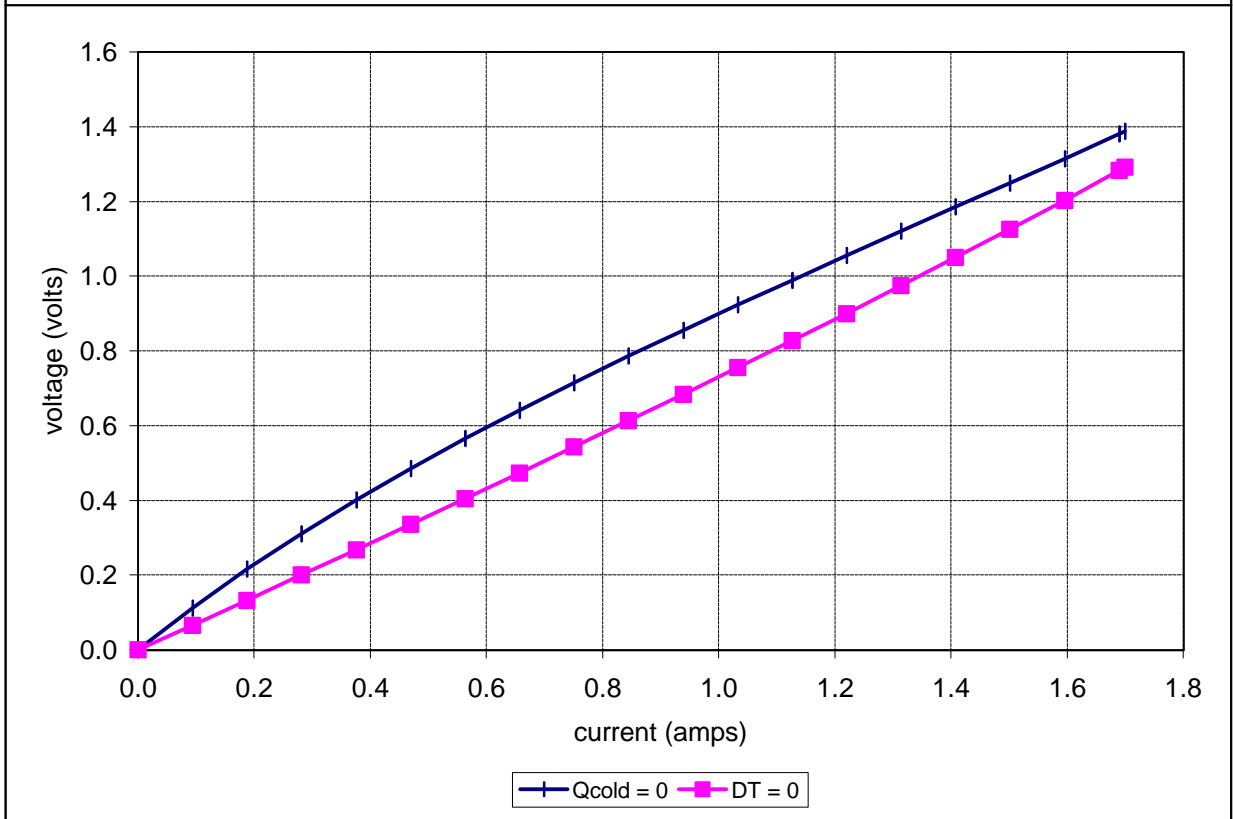
Potted TE-11-0.6-1.0 at a hot-side temperature of 25 °C
