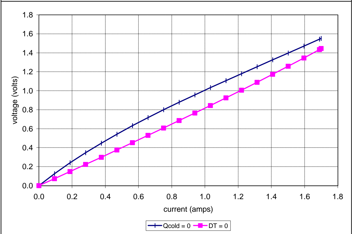
Potted TE-11-0.6-1.0 at a hot-side temperature of 50 °C
