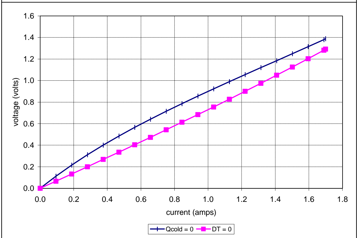
Unpotted TE-11-0.6-1.0 at a hot-side temperature of 25 °C
