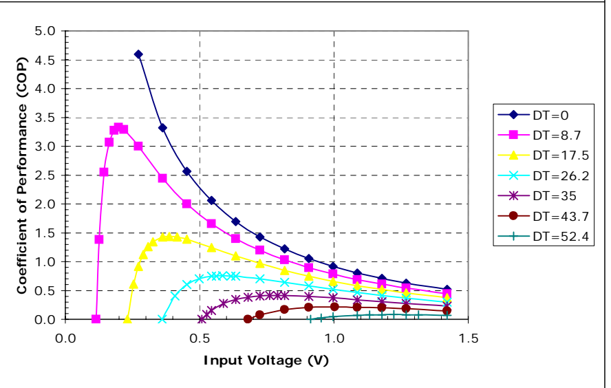
Potted TE-11-0.6-1.0 at a hot-side temperature of 30 °C
