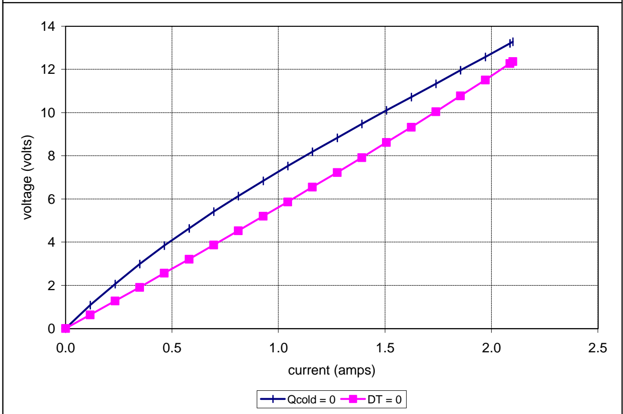
Potted TE-109-0.6-0.8 at a hot-side temperature of 25 °C
