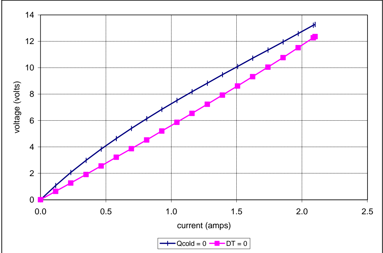
Unpotted TE-109-0.6-0.8 at a hot-side temperature of 25 °C
