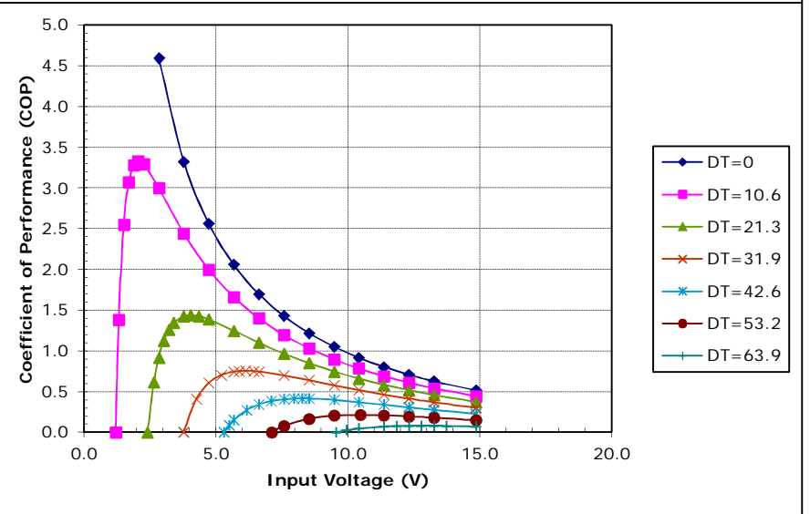
Potted TE-109-0.6-0.8 at a hot-side temperature of 50 °C
