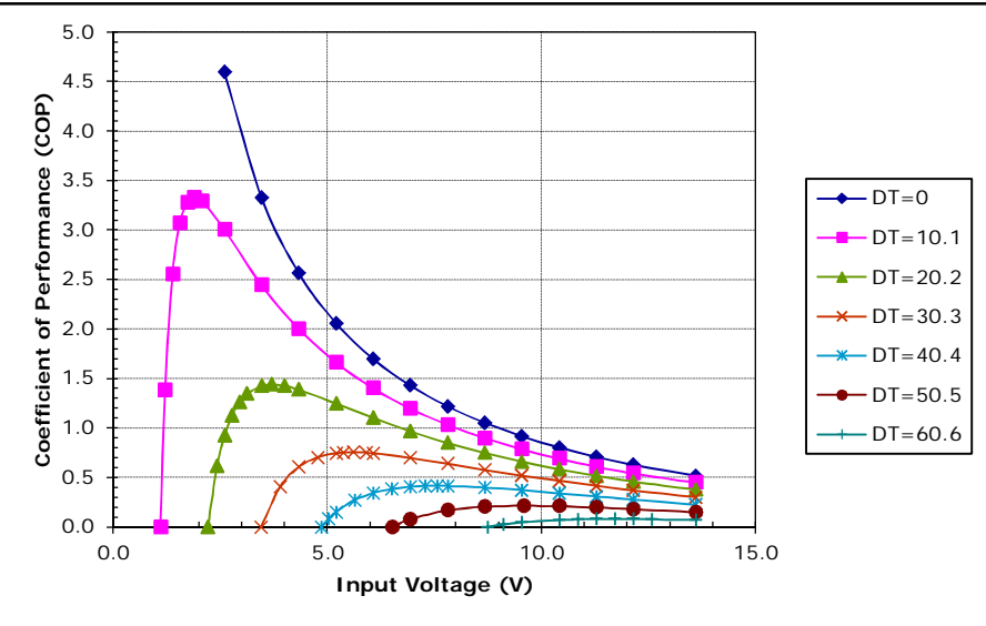
Unpotted TE-109-0.6-0.8 at a hot-side temperature of 30 °C
