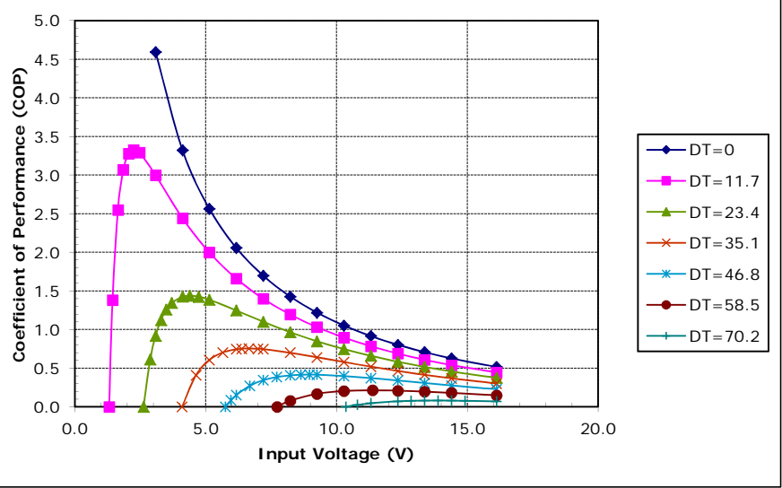
Potted TE-109-0.6-0.8 at a hot-side temperature of 70 °C
