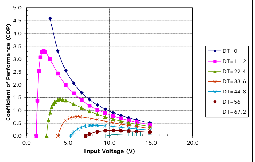
Unpotted TE-109-0.6-0.8 at a hot-side temperature of 50 °C
