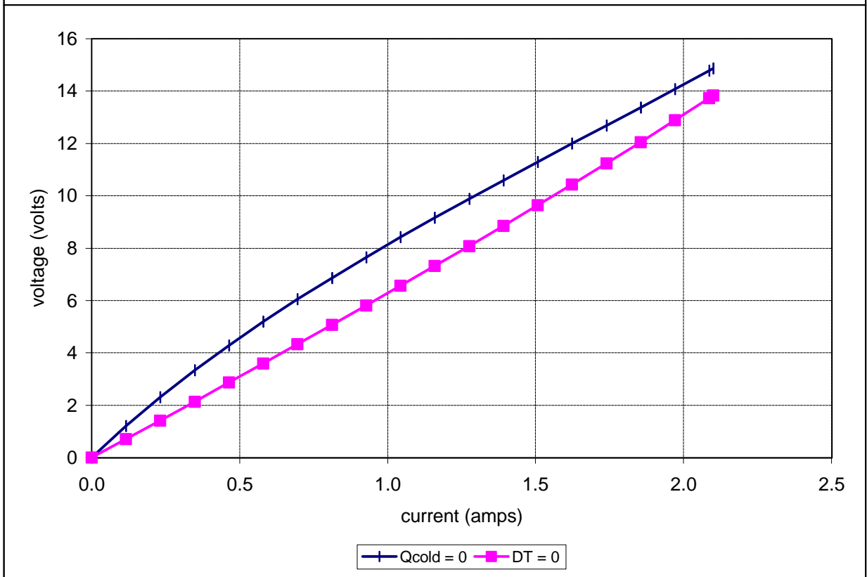
Unpotted TE-109-0.6-0.8 at a hot-side temperature of 50 °C
