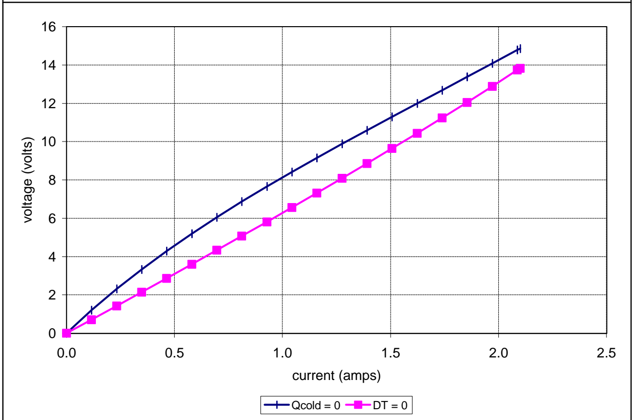
Potted TE-109-0.6-0.8 at a hot-side temperature of 50 °C
