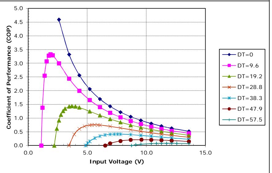
Potted TE-109-0.6-0.8 at a hot-side temperature of 30 °C
