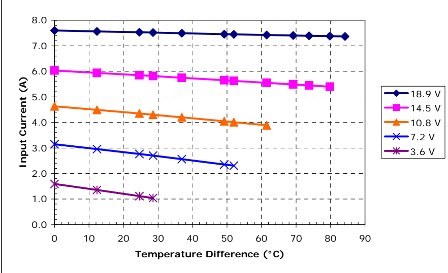
Unpotted SP-262-1.0-1.3 (Parallel) at a hot-side temperature of 70 °C
