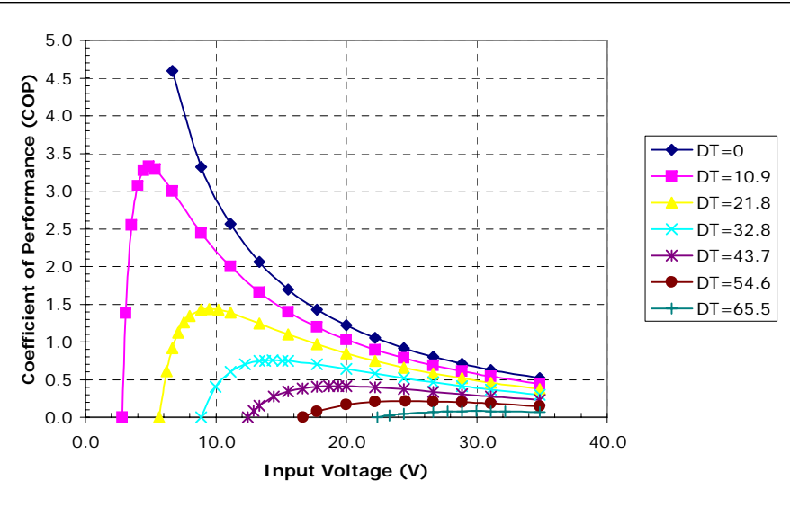
Potted SP-262-1.0-1.3 (Series) at a hot-side temperature of 50 °C
