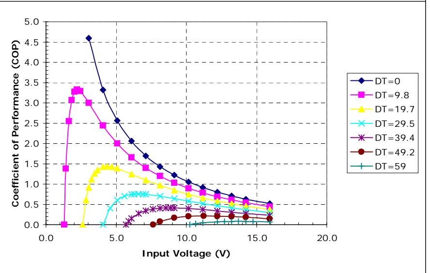
Potted SP-262-1.0-1.3 (Parallel) at a hot-side temperature of 30 °C
