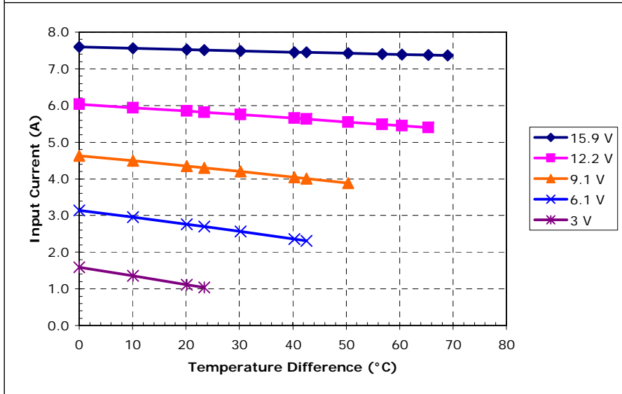
Unpotted SP-262-1.0-1.3 (Parallel) at a hot-side temperature of 30 °C
