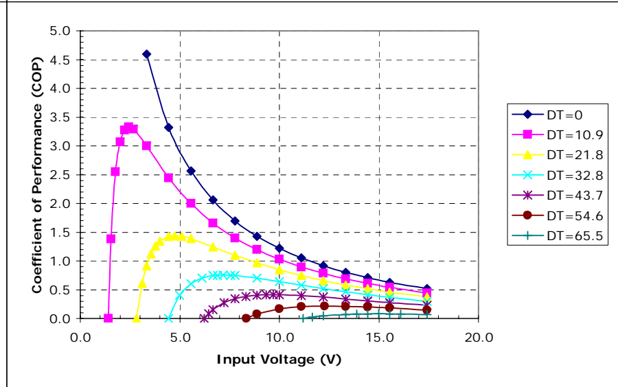
Potted SP-262-1.0-1.3 (Parallel) at a hot-side temperature of 50 °C
