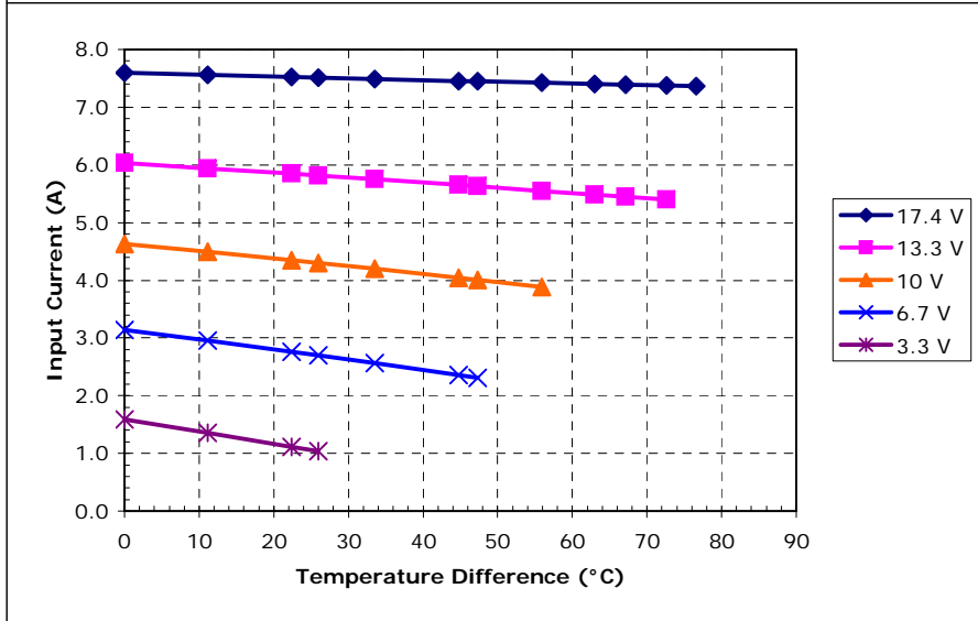
Unpotted SP-262-1.0-1.3 (Parallel) at a hot-side temperature of 50 °C
