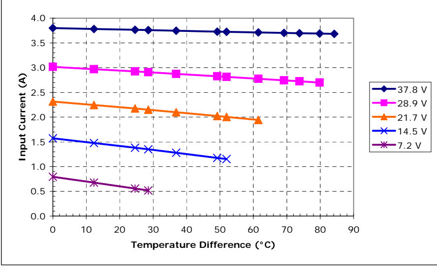
Unpotted SP-262-1.0-1.3 (Series) at a hot-side temperature of 70 °C
