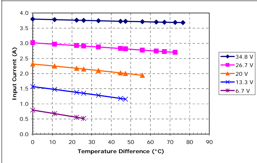
Unpotted SP-262-1.0-1.3 (Series) at a hot-side temperature of 50 °C
