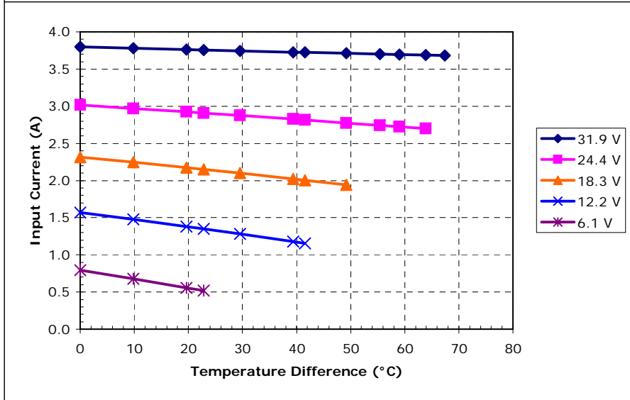
Potted SP-262-1.0-1.3 (Series) at a hot-side temperature of 30 °C
