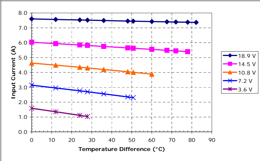
Potted SP-262-1.0-1.3 (Parallel) at a hot-side temperature of 70 °C
