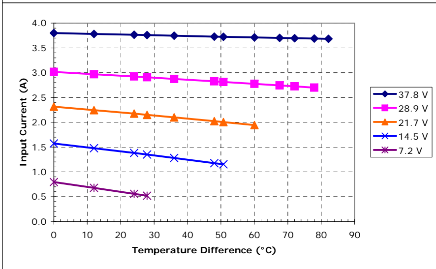
Potted SP-262-1.0-1.3 (Series) at a hot-side temperature of 70 °C
