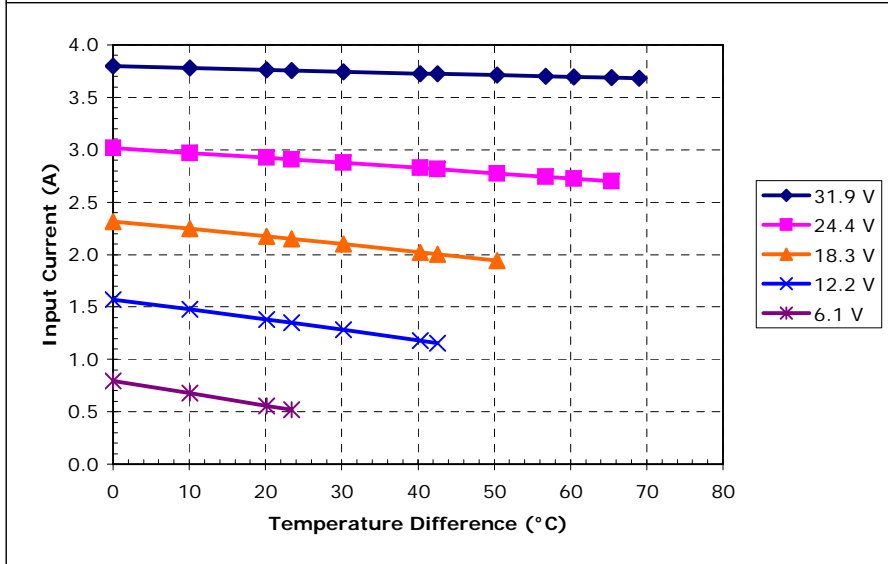
Unpotted SP-262-1.0-1.3 (Series) at a hot-side temperature of 30 °C
